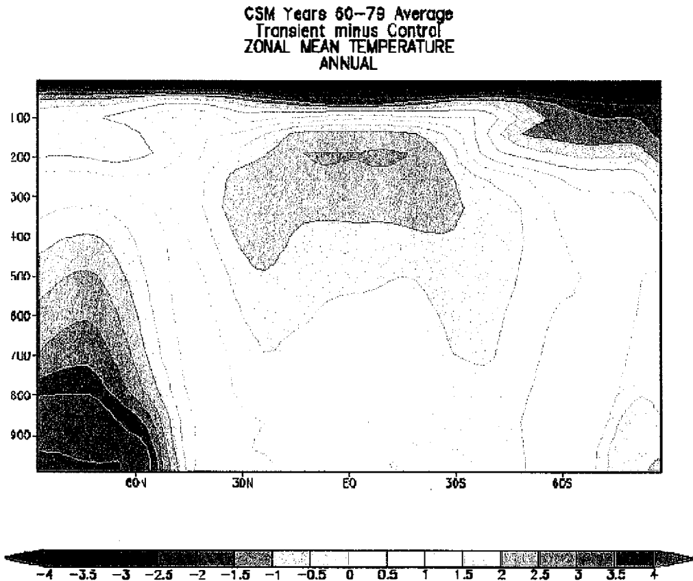
Fig. 19. Vertical cross sections of zonally-averaged model temperature changes averaged over 20 years (years 60-79) in NCAR Climate System Model in which carbon dioxide alone is increased by 1% per year (Meehl et al. , 2000).
