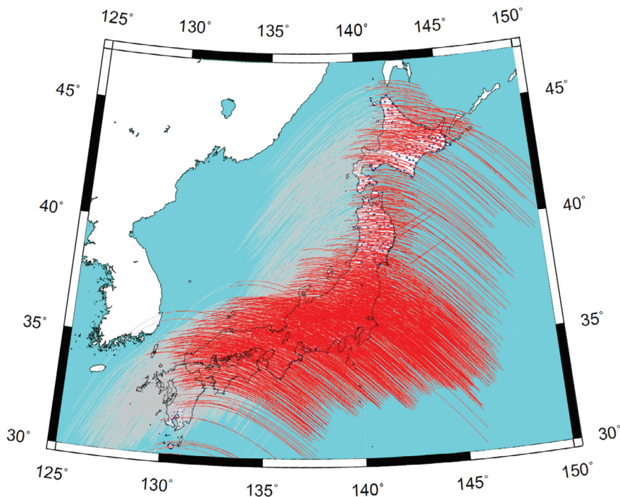
Fig. 4. SIP trajectories for GPS Satellite 15, calculated assuming a thin ionosphere as high as 350 km. Grey and red lines show the individual SIP trajectories of GEONET GPS receiver stations (used in this study) for the 2 hours before and after the earthquake origin, respectively.
