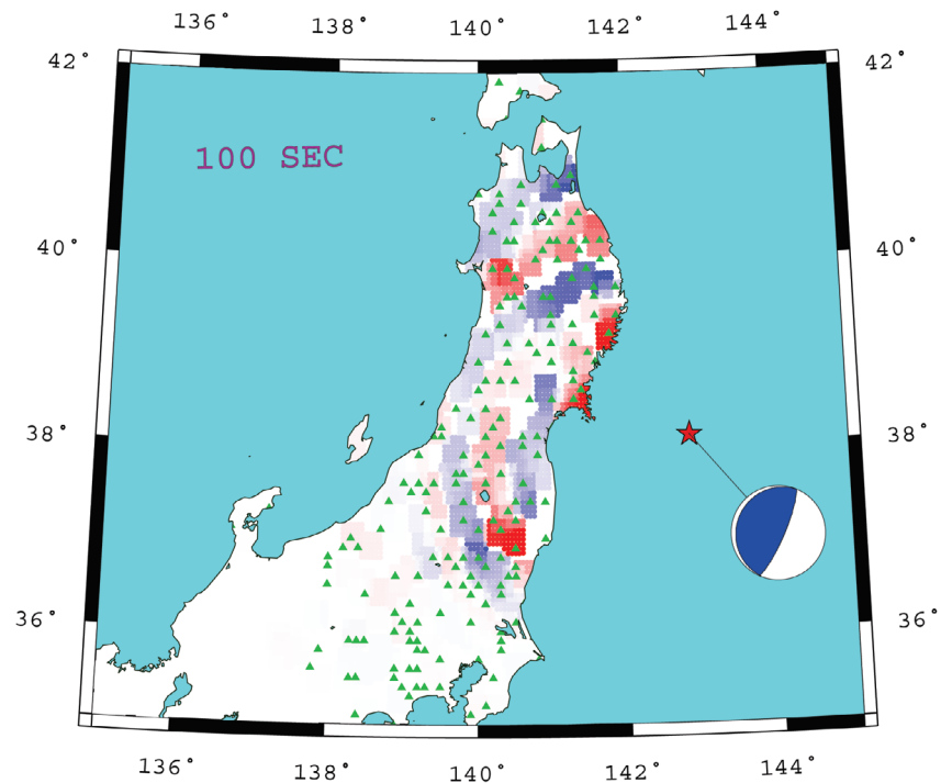
Fig. 2. Snapshot of seismic-wave propagation using data of K-net/KiK-net (NIED). The amplitude of the vertical component (velocity) is indicated by color (red = upward; blue = downward). The red star shows the epicenter of the 2011 off the Pacific coast of Tohoku Earthquake, and green triangles indicate observation stations used for this analysis. The time at upper left indicates the time from the earthquake origin.
