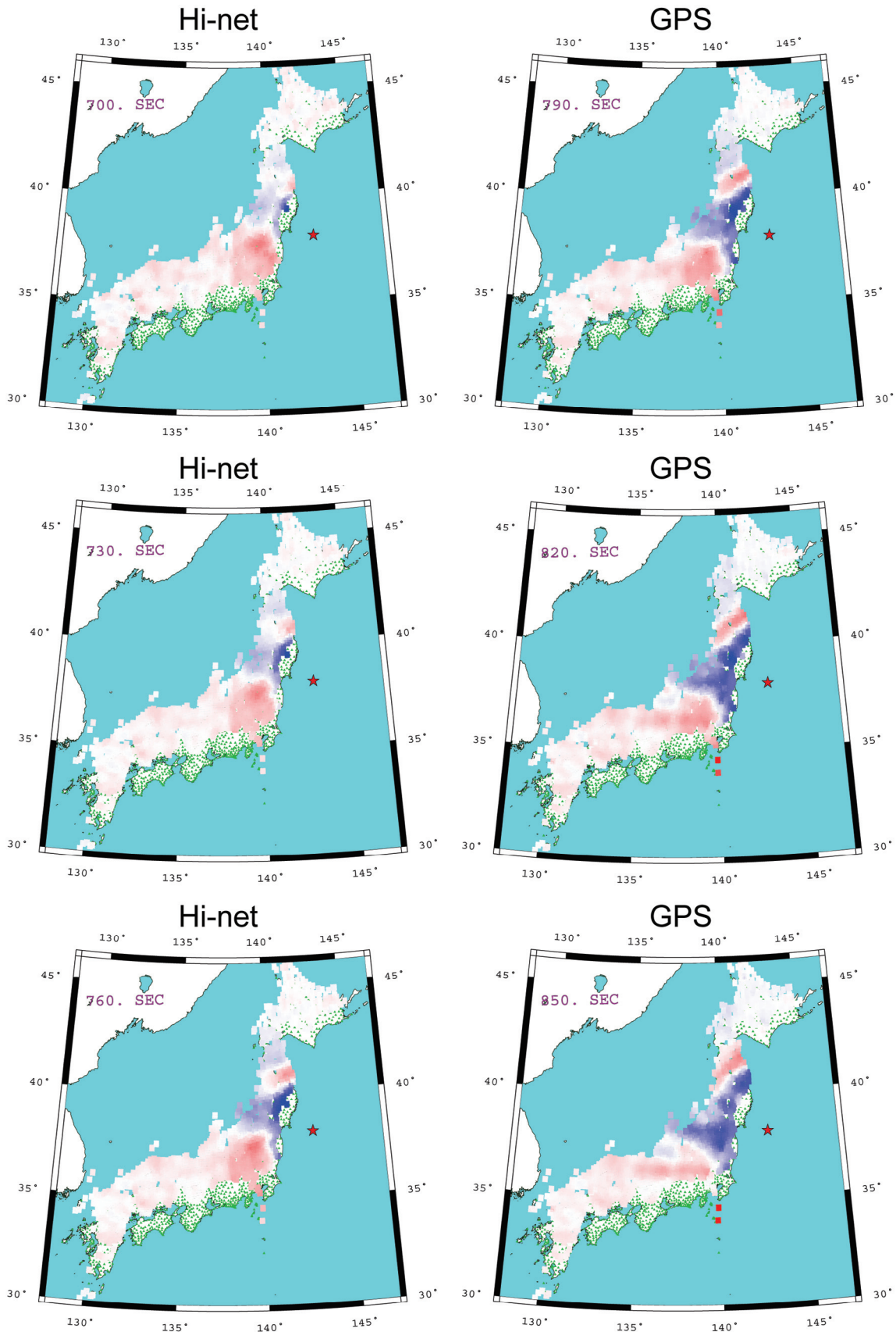
Fig. 5 Snapshots of the propagating STID for GPS Satellite 15 after the 2011 Tohoku Earthquake. The red star indicates the epicenter, and green triangles represent GPS receiver stations used in this study. The amplitude of the wavefield is shown by color (red = upward, blue = downward). The time at upper left in each panel is the time from the earthquake origin.
