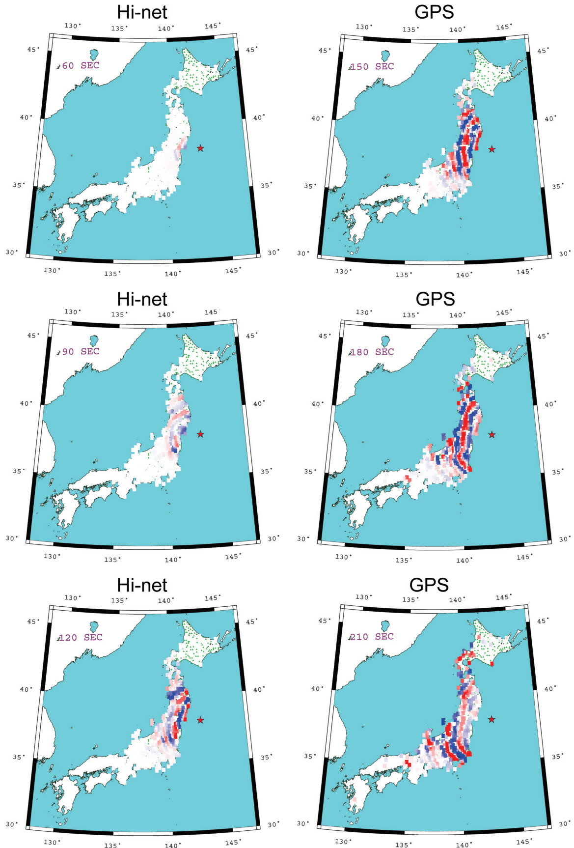
Fig. 3. Snapshots of the ground motions (velocity) over Japan after the Tohoku Earthquake (time interval, 30 s). For an explanation of symbols, etc., see Fig. 2.
