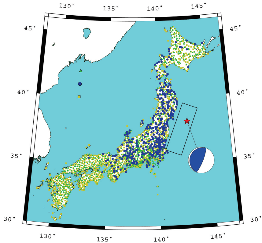
Fig. 1. Distribution of seismic stations of the National Research Institute for Earth Science and Disaster Prevention (NIED)'s Hi-net (filled triangles) and K-net/KiK-net (dots) networks, and receiver stations (filled squares) of the GPS Earth Observation Network (GEONET) GPS array. The red star shows the epicenter of the 2011 off the Pacific coast of Tohoku Earthquake, and the open rectangle represents the proposed fault rupture area of this event (modified from ERI, 2011).
