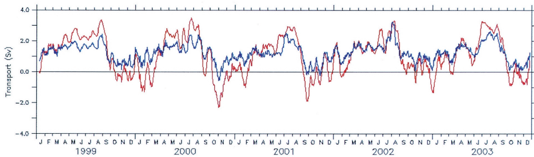
Fig. 8. Comparison between model transport (red line) and transport estimated using a resistance coefficient (blue line) during the period from 1999 to 2003.
