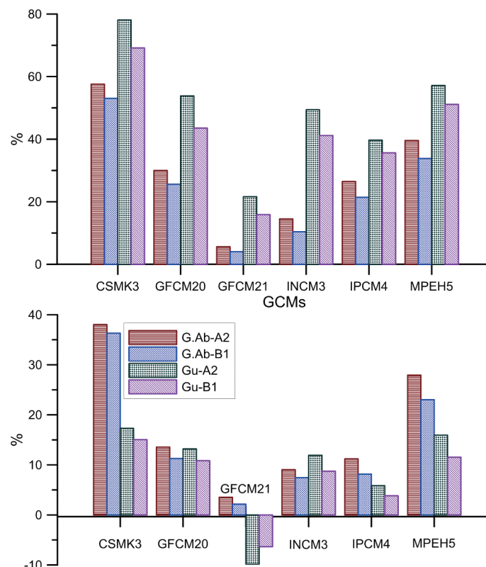
Fig. 11. Projected runoff change in percentage for dry season (top) and wet season (bottom) of Gilgel Abbay and Gumara watersheds with reference to the baseline. (Color online only)
