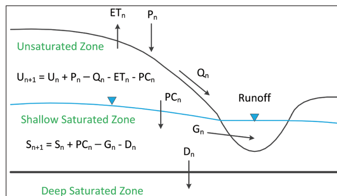
Fig. 3. Schematic diagram of GWLF hydrological routing model, where ET is evapotranspiration, P is precipitation, Q is surface runoff, and G is groundwater discharge, U is available moisture content of unsaturated zone, PC percolation from unsaturated zone into shallow saturated zone, D is deep seepage from shallow saturated zone into deep saturated zone, and the subscript "n" denotes the n-th day (modified after Haith et al. 1992). (Color online only)
