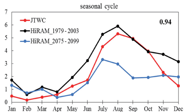
Fig. 1. Seasonal cycle of TS genesis frequency (unit: number of TS per month per year) for observation (red line), HiRAM model simulation during 1979 - 2003 (black line), and HiRAM projection during 2075 - 2099 (blue line). The number in the upper corner is the correlation coefficient between the HiRAM simulation (black line) and observation (red line).
