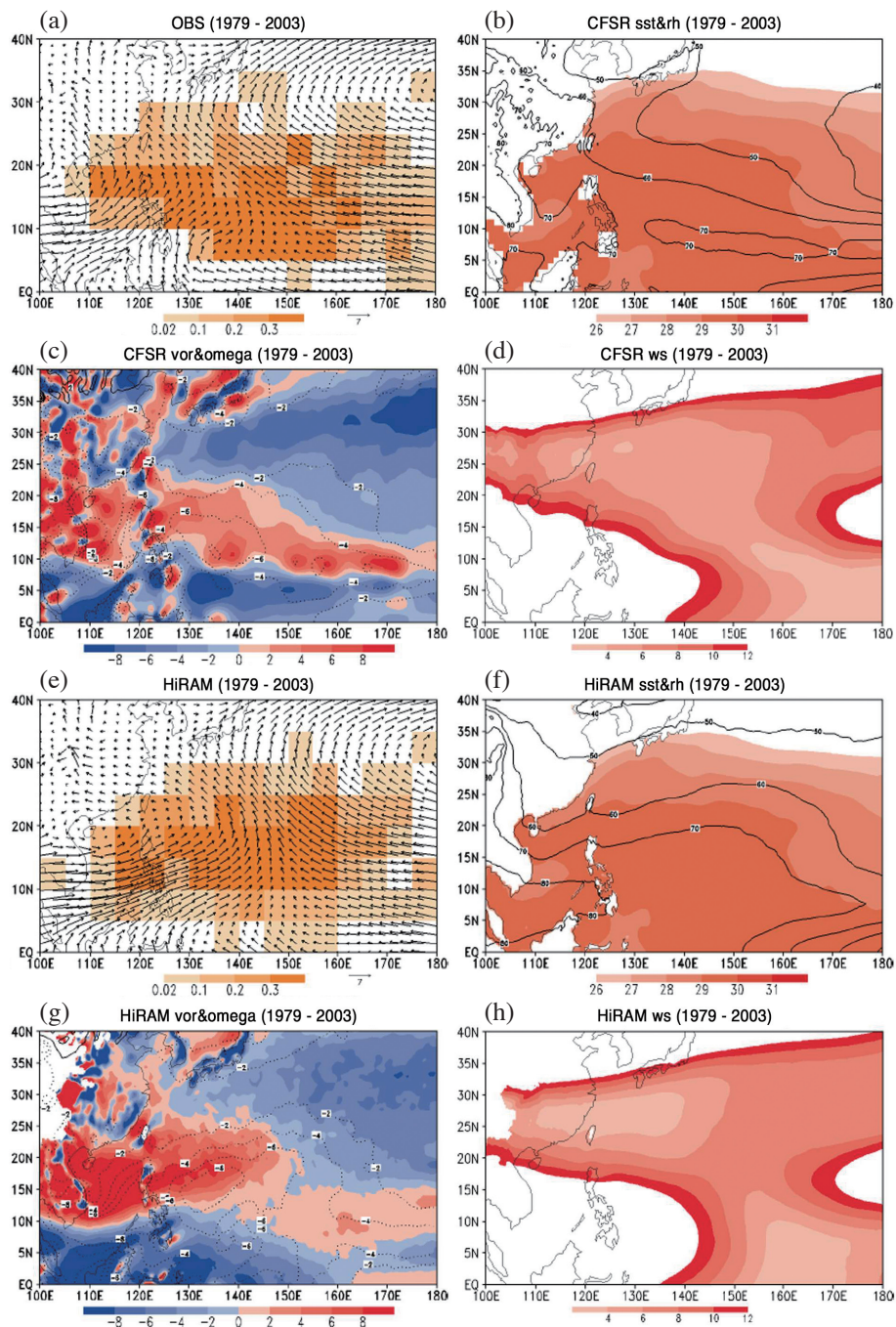
Fig. 12. Observed large-scale environment distribution during JAS for the period 1979 - 2003. (a) 850 hPa wind fields (m s -1 ) and TS formation frequency (shaded, unit: numbers per season), (b) SST (shaded, °C) and 600 hPa relative humidity (%), (c) 850 hPa relative vorticity (shaded, 10 -6 s -1 ) and 500 hPa \omega (contour, 10 -2 Pa s -1 ), (d) vertical wind shear (m s -1 ). (e) - (h) as in (a) - (d), except for HiRAM.
