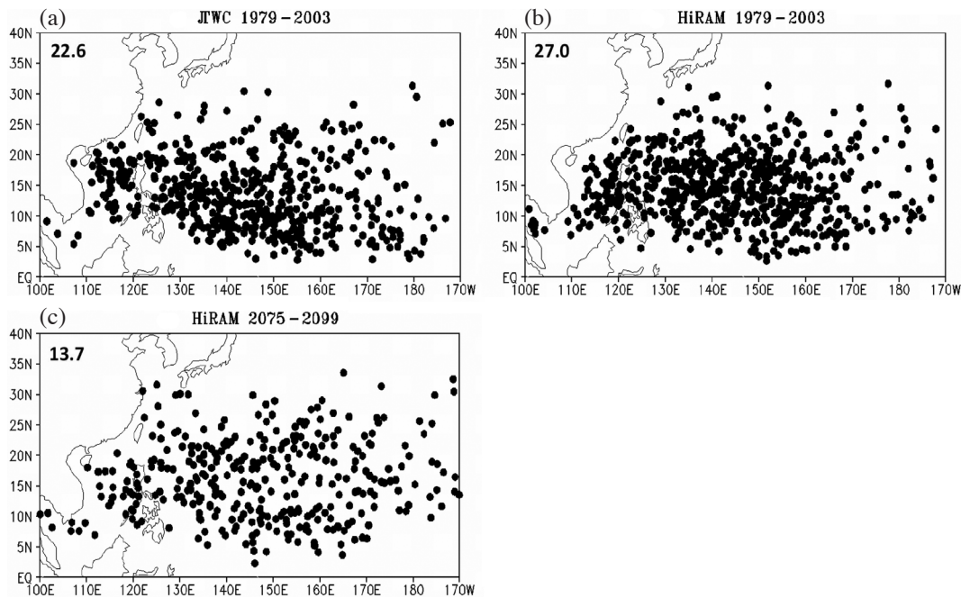
Fig. 2. TS formation location distribution (dots) from June to November (JJASON) for the period 1979 - 2003 in (a) JTWC and (b) HiRAM. (c) same as (b), but for the period 2075 - 2099. The numbers in the upper corners are TS total numbers (unit: numbers per year).
