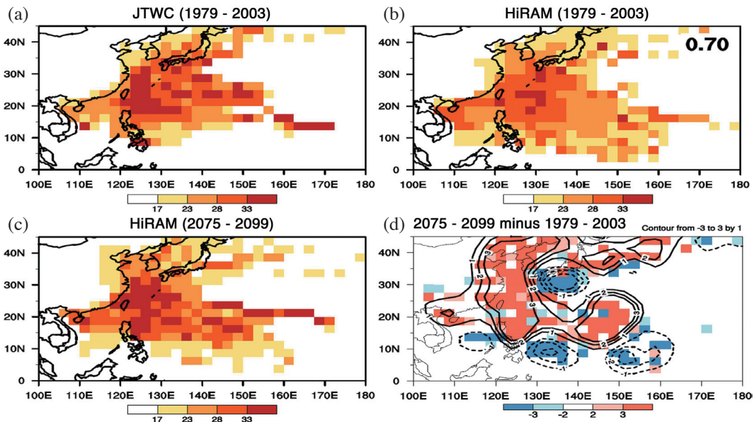
Fig. 9. (a), (b), (c), (d) same as Fig. 6, but for TS affecting TWCN region.
