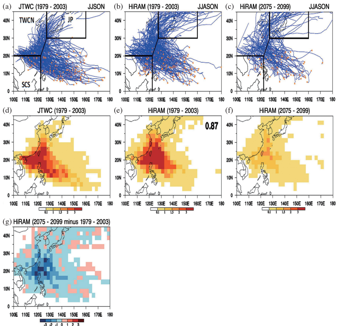
Fig. 8. Same as Fig. 4, but for TS affecting TWCN region.
