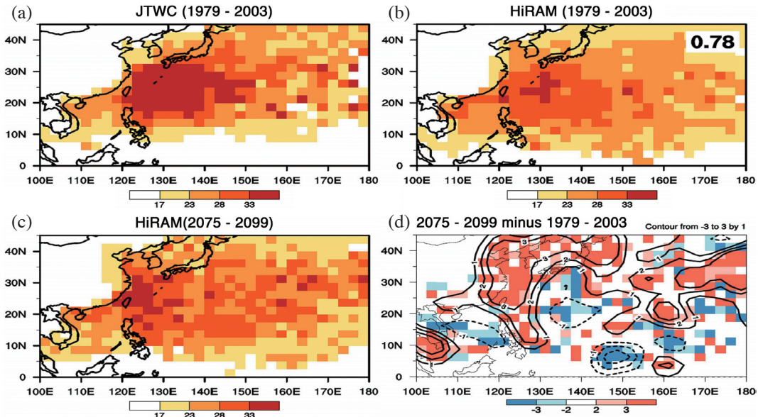
Fig. 6. TS intensity distribution (unit: \text{m s}^{-1} per 2.5^\circ longitude/latitude per year) during JJASON for the period 1979 - 2003 for (a) observation, (b) HiRAM. (c) same as (b), but for the period 2075 - 2099. (d) Difference between the present and future projection in HiRAM (2075-2099 minus 1979 - 2003).
