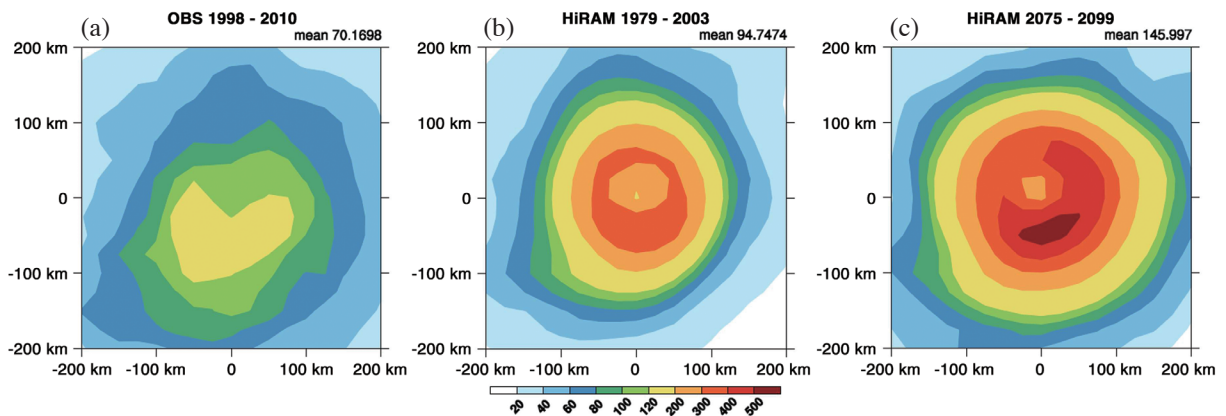
Fig. 11. (a), (b), (c) same as Fig. 7, but for TS affecting TWCN region.
