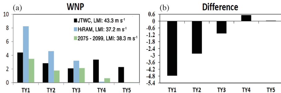
Fig. 5. (a) The frequency (unit: numbers per year) of Category 1 to 5 storms for observation and HiRAM during JJASON for the period 1979 - 2003, and HiRAM for the period 2075 - 2099. (b) Projection changes in the TS number (2075 - 2099 minus 1979 - 2003) for HiRAM. The number in the upper corner of (a) is the mean LMI (the maximum intensity achieved during a storm's lifetime) for observation, HiRAM, and future projection, respectively.
