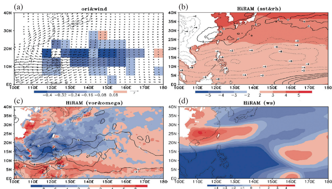
Fig. 13. Projection changes in the large-scale environment during JAS (2075 - 2099 minus 1979 - 2003) for (a) 850 hPa wind fields ( \text{m s}^{-1} ) and TS formation frequency (shaded, numbers per season), (b) SST (shaded, ^{\circ}\text{C} ) and 600 hPa relative humidity (%), (c) 850 hPa relative vorticity (shaded, 10^{-6} \text{ s}^{-1} ) and 500 hPa \omega (contour, 10^{-2} \text{ Pa s}^{-1} ), (d) vertical wind shear ( \text{m s}^{-1} ).
