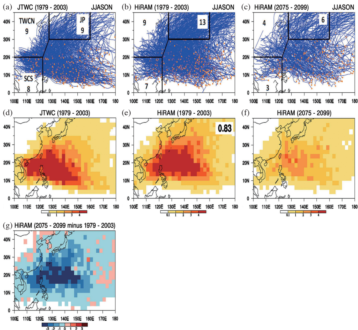
Fig. 4. TS tracks and TS frequency during JJASON for the period 1979 - 2003 for (a) JTWC and (b) HiRAM. (c) same as (b), but for the period 2075 - 2099. (d) - (f) TS frequency (numbers per 2.5° longitude/latitude per year). (g) Difference between the present and future projection in HiRAM (2075 - 2099 minus 1979 - 2003). Black lines in (a) - (c) show the boundaries of three landfall regions classified in this study. The characters TWCN, SCS, and JP represent Taiwan and the east coast of China (TWCN), the South China Sea region (including Philippines, SCS), and the Japan (JP) landfall regions, respectively. The numbers in each box are the number of TSs affecting each region (numbers per year). The number in the upper corner of (e) is the pattern correlation coefficient between HiRAM experiments and observation.
