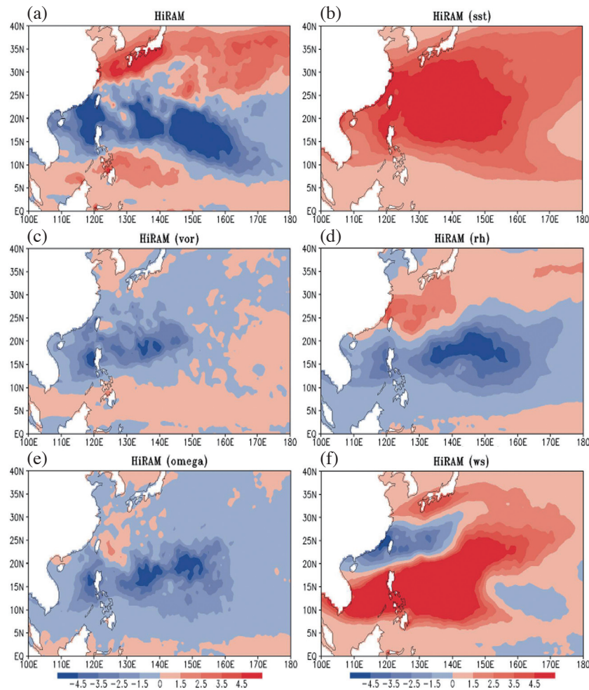
Fig. 15. GPI changes induced by all forcing terms and individual terms between the present and future time in HiRAM (2075 - 2099 minus 1979 - 2003) for (a) all forcing terms, (b) SST, (c) 850 hPa relative vorticity, (d) 600 hPa relative humidity, (e) 500 hPa \omega , (f) vertical wind shear.
