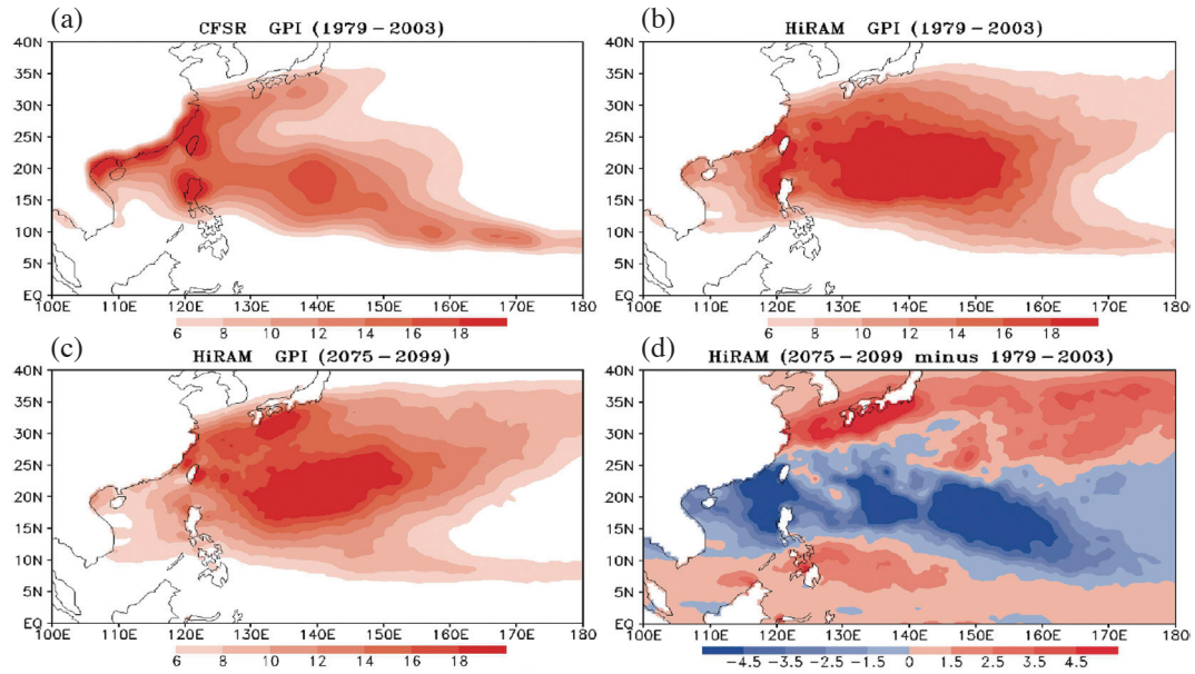
Fig. 14. GPI Distribution during JAS for the period 1979 - 2003 for (a) observation, (b) HiRAM. (c) same as (b), but for the period 2075 - 2099. (d) Difference between the present and future projection in HiRAM (2075 - 2099 minus 1979 - 2003).
