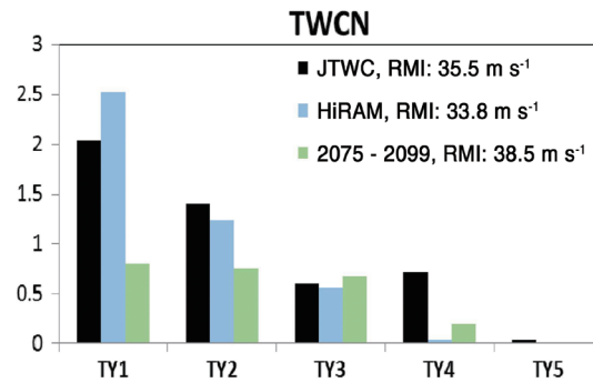
Fig. 10. Same as Fig. 5a, but for TS affecting TWCN region. TS intensity scale is determined by the maximum intensity achieved within TWCN region (RMI).
