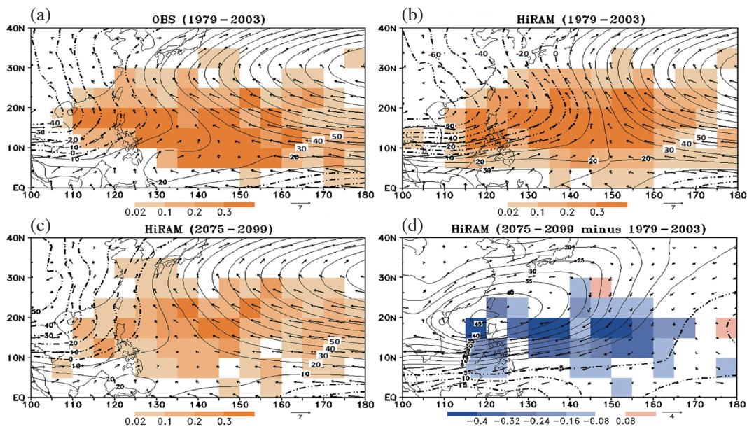
Fig. 3. TS formation frequency distribution (shaded, unit: numbers per 5^\circ longitude/latitude per year), 850 hPa wind fields ( \text{m s}^{-1} ) and 850 hPa stream function (contour, unit: 10^5 \text{ m}^2 \text{ s}^{-1} ) during JAS for the period 1979 - 2003 for (a) observation, (b) HiRAM. (c) same as (b), but for the period 2075 - 2099. (d) Difference between the present and future projection in HiRAM (2075 - 2099 minus 1979 - 2003).
