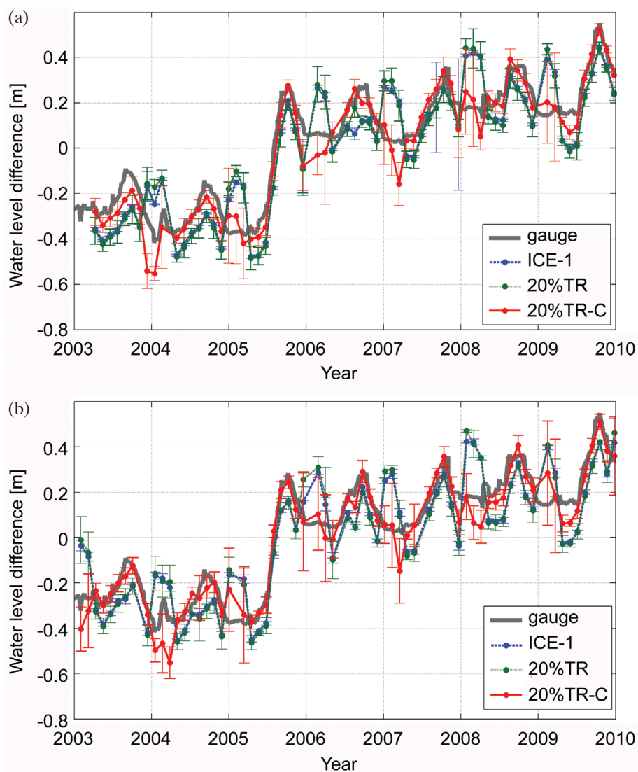
Fig. 8. Top: A comparison of water level variation for Envisat pass #240, between gauge (gray), Envisat ICE-1 (blue), 20% TR without correction (green), and 20% TR after correction (red). Bottom: A similar comparison for Envisat pass # 276.
