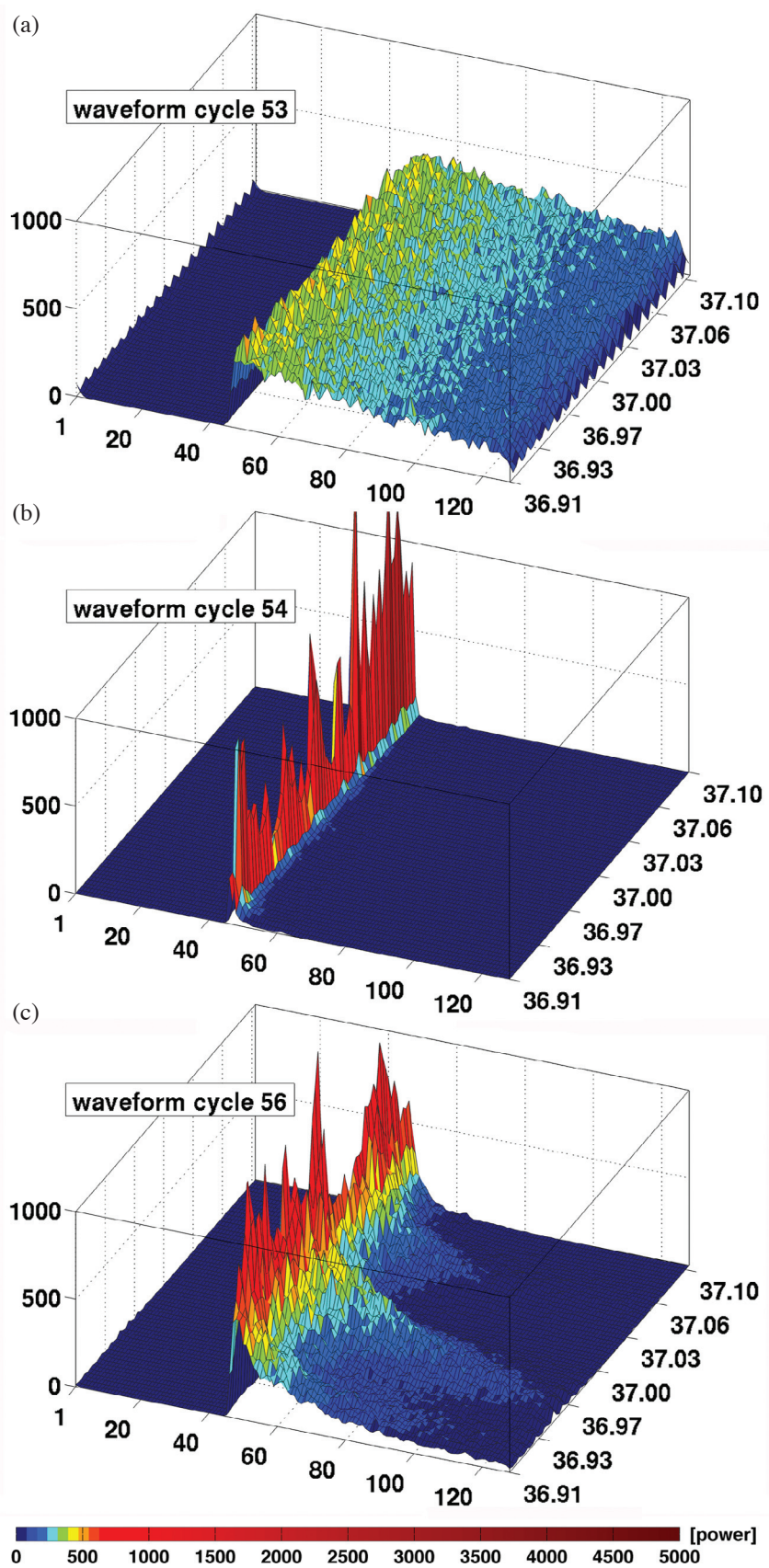
Fig. 3. Typical along-track waveforms returned from different surface conditions and corresponding months: (a) water (April - November), (b) ice (December - March), and (c) water with ice floes (March and December). X-axis is waveform gates (or bins), Y-axis indicates latitude in degree, and Z-axis indicates returned energy in power unit. These samples are demonstrated by Envisat pass #240 in cycles [from (a), (b), (c)] 53, 54, and 56.
