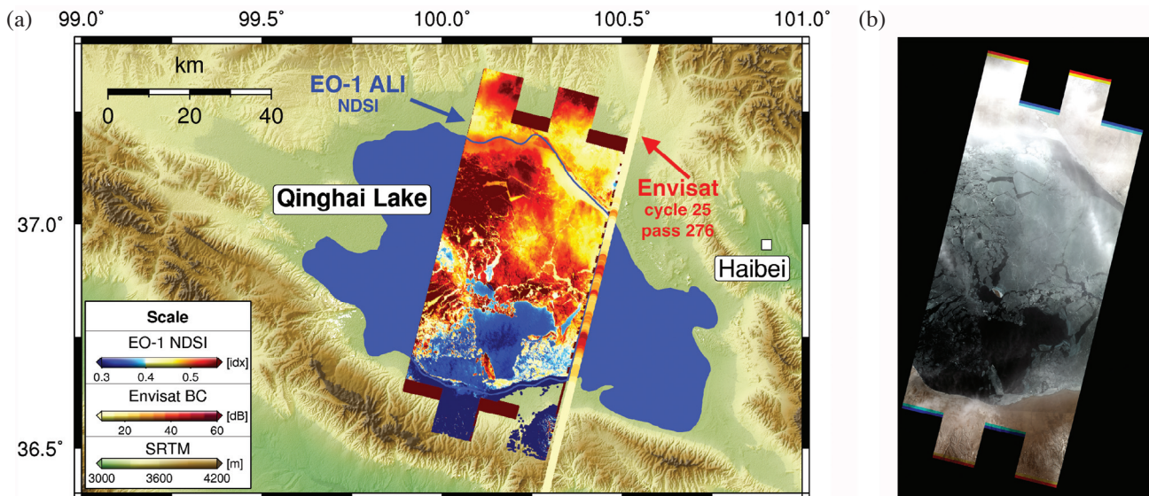
Fig. 6. (a) Lake ice/snow extent estimated by NDSI is computed from EO-1 ALI imagery on 03/21/2004. Envisat pass #276 color-coded by a backscattering coefficient (BC) was measured on 03/28/2004. The higher values of BC than normal water surface return (15 - 20 dB) fluctuate while satellite ground track overpasses ice floes. Background relief is scaled by C-band SRTM3 DEM. (b) False-color images composed by ENVI software are computed from original multispectral imagery (R: Band 3, G: Band 2, B: Band 1), with approximate cloud coverage 30 - 39% mostly in the upper part.
