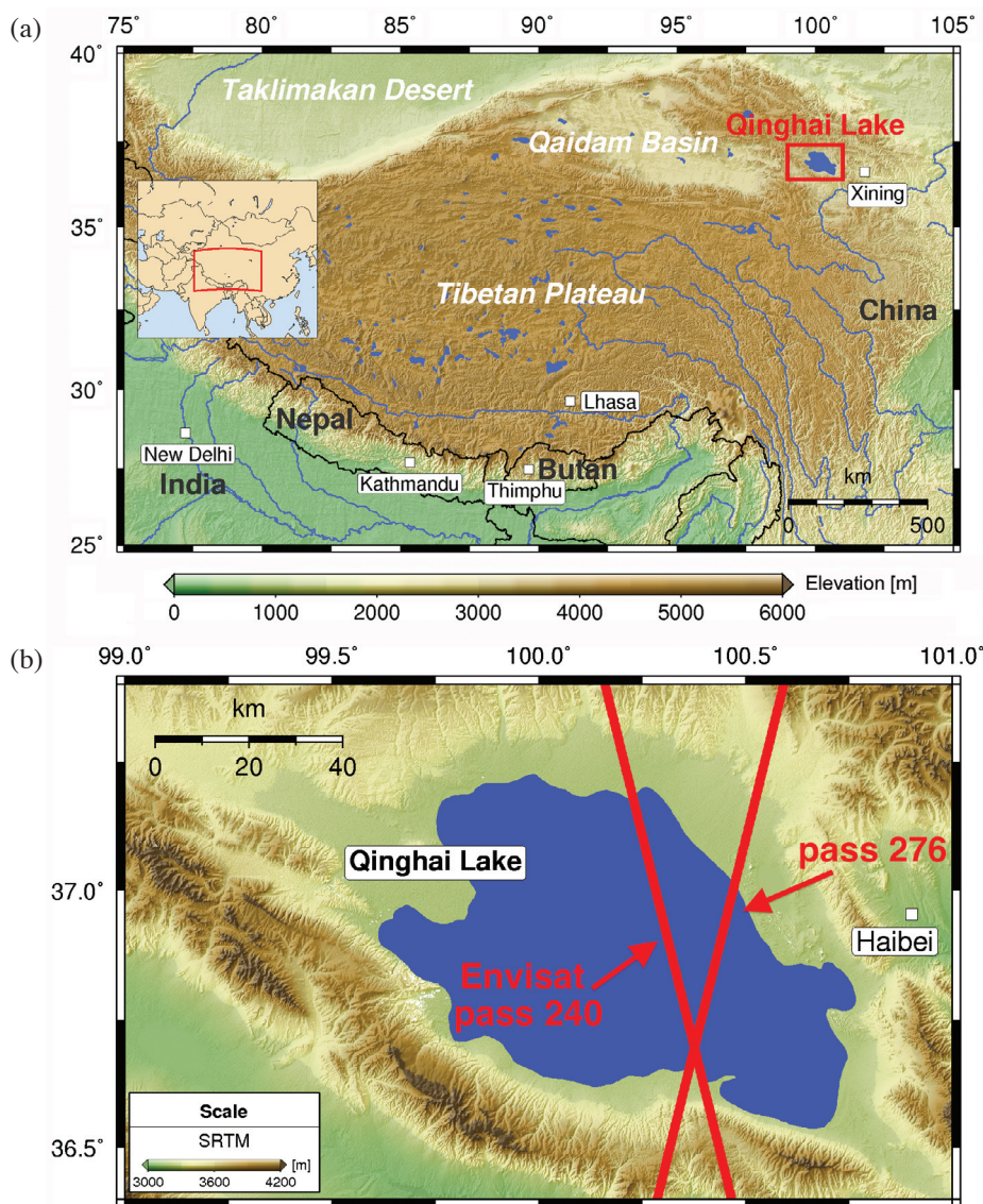
Fig. 1. (a) Location of the Qinghai Lake on the Tibetan Plateau (red box). The topographic relief is scaled by GTOPO30 DEM. (b) Two Envisat passes #240 and #276 (red) are included in this study. SRTM 3 arc-second C-band DEM is used as a topographic relief. The lake boundary refers to the World Vector Shorelines (WVS) and CIA World Data Bank II (WDBII) composed by the Generic Mapping Tools (GMT) (Wessel and Smith 2010).
