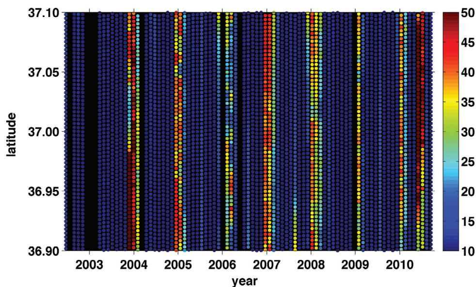
Fig. 2. Along-track (ordinate) variation of the Envisat pass #240 backscattering coefficient (BC, unit: [dB]) in time (abscissa). BC blooms are often noted in December, January, and February each year when the lake becomes icy with the least surface roughness and higher reflectivity. Some cycles are missing (e.g., early in 2003) due to data outage, a lost-lock in altimeter, or data failed to meet the edit criteria.
