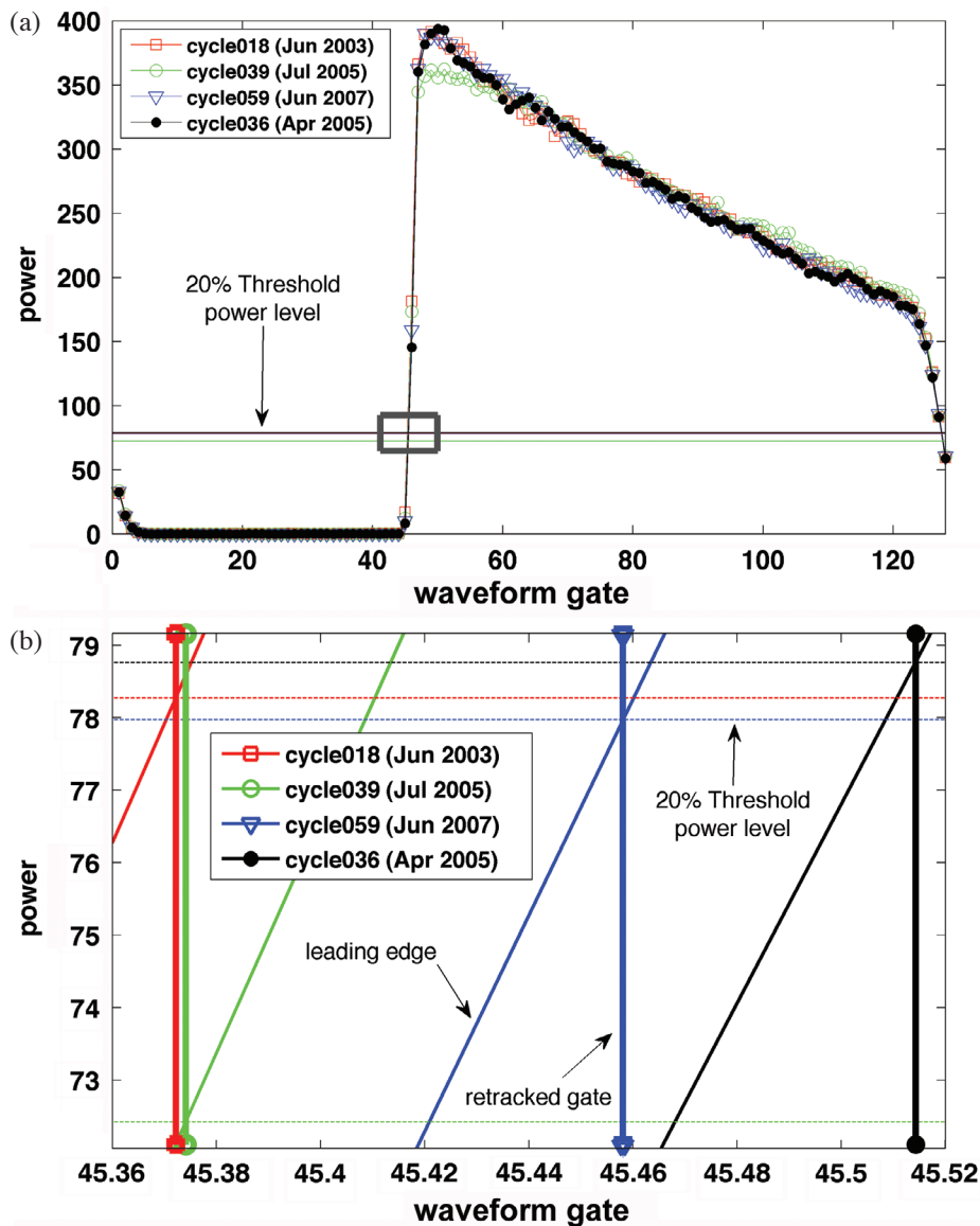
Fig. 7. A demonstration of water waveforms collected over different months. Top: Four waveforms have a similar leading/trailing edge slope and the power level computed from 20% peak power amplitude also located at a comparable level. Bottom: A blow-up view of the retracked gate denoted as a gray box in the top panel. Vertical line indicates the retracked gate obtained from the intersection between 20% threshold power level (horizontal line) and the leading edge. The offset among retracked gates is less than 0.15 (or 7 cm in length equivalent) in given examples.
