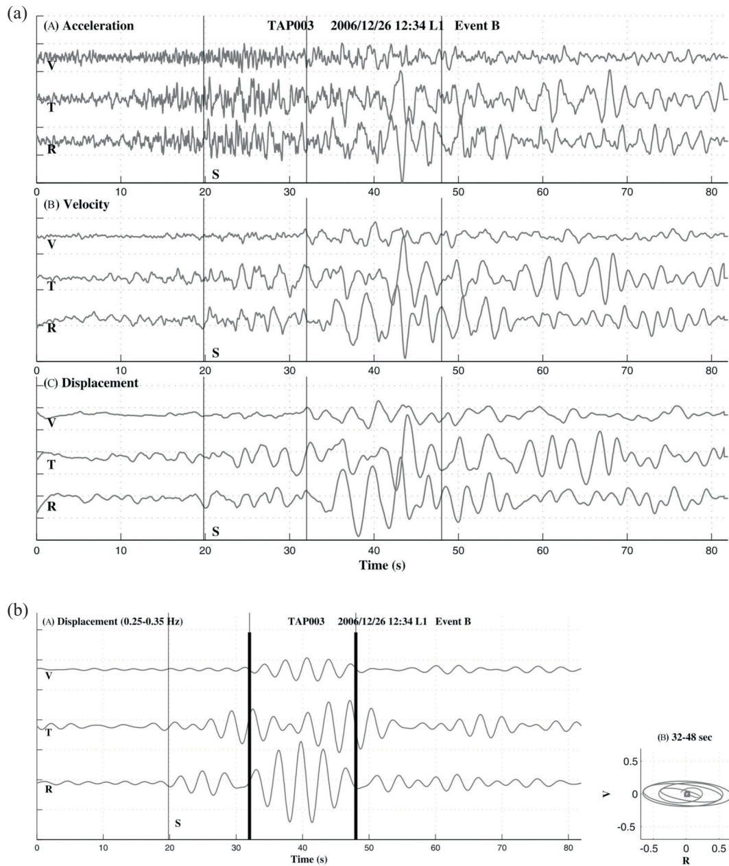
Fig. 11. (a) The rotated three-component accelerograms, velocity waveforms, and displacement waveforms of the B event recorded at TAP003; (b) The filtered displacement waveforms in the frequency band of 0.25 - 0.35 Hz and the particle motions in the time interval of 32 - 48 sec. Square refers to the start of particle motion.
