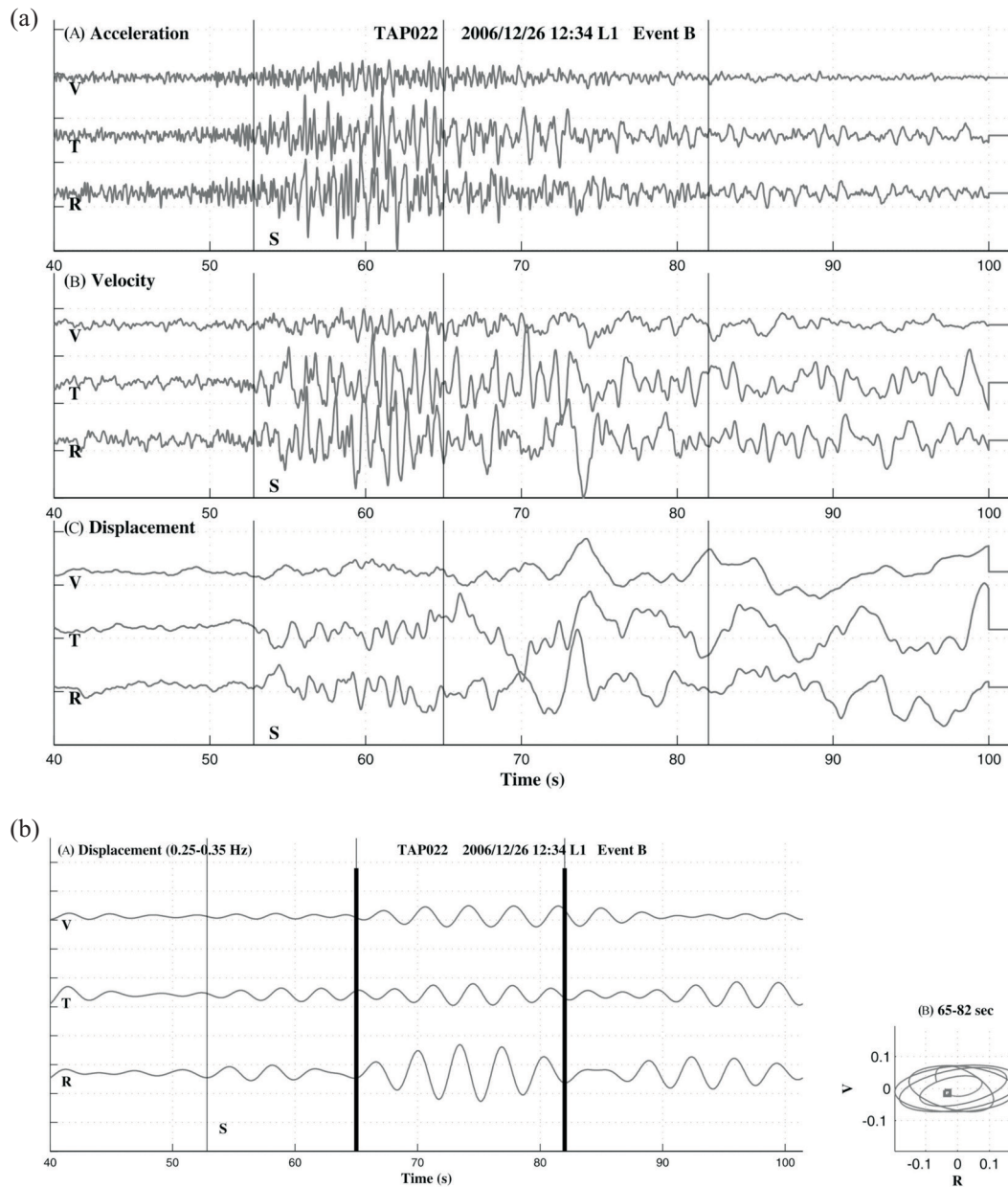
Fig. 10. (a) The rotated three-component accelerograms, velocity waveforms, and displacement waveforms of the B event recorded at TAP022; (b) The filtered displacement waveforms in the frequency band of 0.25 - 0.35 Hz and the particle motions in the time interval of 65 - 82 sec. Square refers to the start of particle motion.
