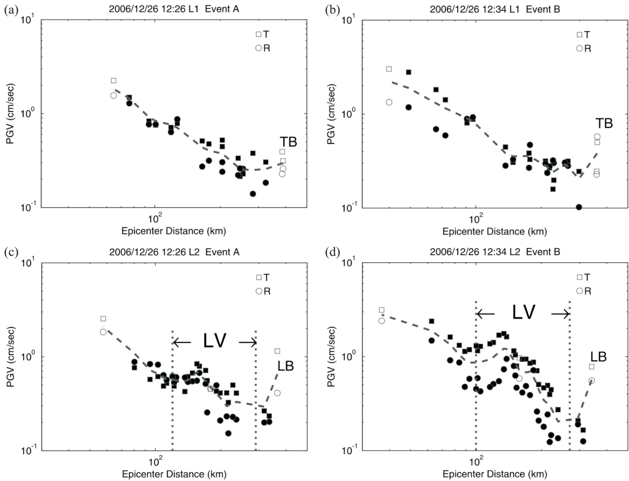
Fig. 5. The transverse and radial components of PGV filtered from 0.05 to 0.5 Hz as a function of distance: (a) and (b) along L1 for the A and B events and (c) and (d) along L2 for the two events. The squares and circles in each panel denote, respectively, transverse and radial components of filtered PGV. The solid and blank symbols indicate rock-type (Class-B and -C) and soil-type (Class-D and -E) sites, respectively. The dashed line denotes the smoothing curve for the filtered PGV. Note that in addition to the amplification in the Taipei basin (TB) and the Lanyang basin (LB), the filtered PGV of both two events show anomalously high values along the LV.
