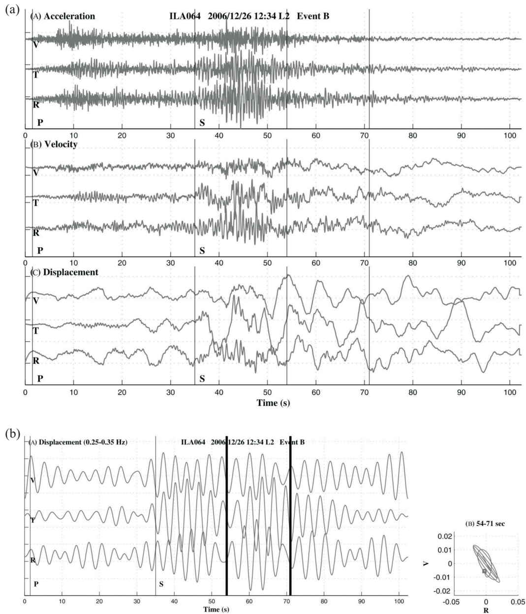
Fig. 12. (a) The rotated three-component accelerograms, velocity waveforms, and displacement waveforms of the B event recorded at ILA064; (b) The filtered displacement waveforms in the frequency band of 0.25 - 0.35 Hz and the particle motions in the time interval of 54 - 71 sec. Square refers to the start of particle motion.
