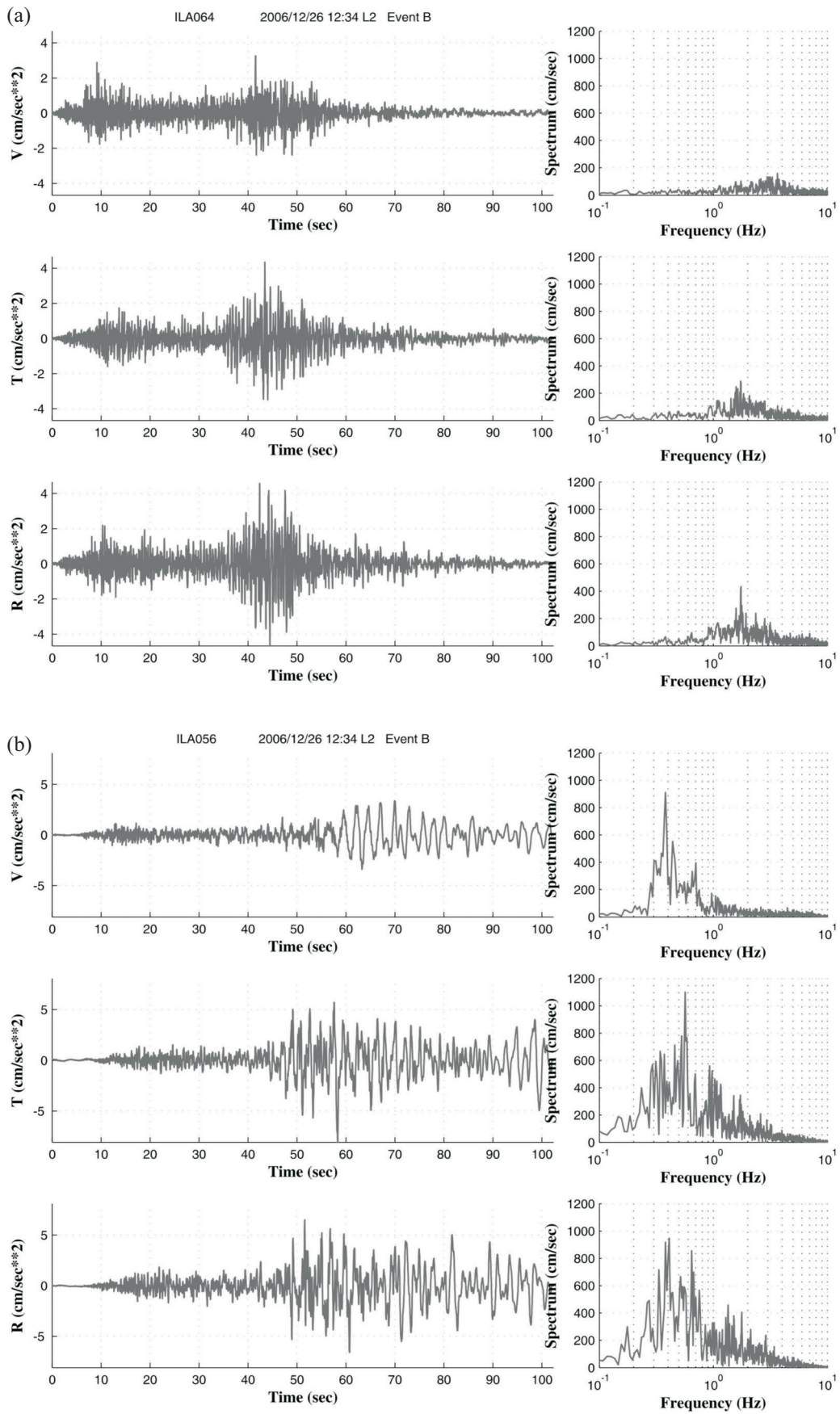
Fig. 9. The rotated three-component acceleration seismograms of the B event recorded at (a) ILA064 and (b) ILA056. The individual Fourier amplitude spectra are shown in the right panels.
