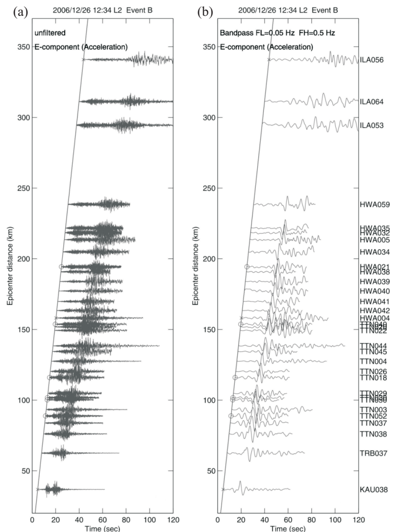
Fig. 2. (a) The original EW-component acceleration seismograms for the B event recorded at the stations along L2 as shown in Fig. 1 and (b) the related filtered acceleration waveforms in the frequency band of 0.05 - 0.5 Hz. Station names are given at the right panel. All the traces are aligned to the P-arrivals and normalized to their maximum amplitudes. Site classification defined by Lee et al. (2001) is also shown at the beginning of each trace: a circle for a Class-B site, none for a Class-C site, and an asterisk for a Class-D site.
