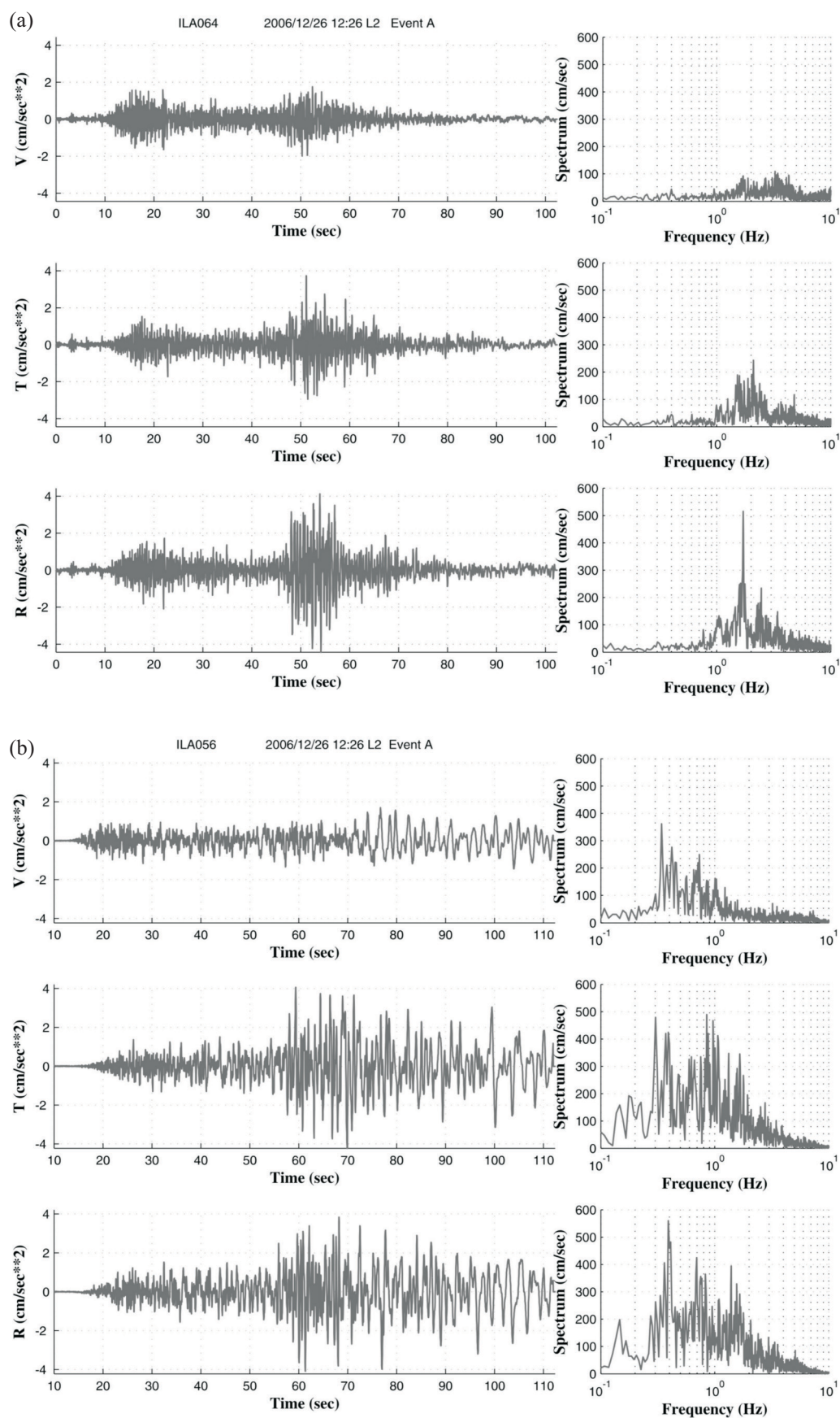
Fig. 7. The rotated three-component acceleration seismograms of the A event recorded at (a) ILA064 and (b) ILA056. The individual Fourier amplitude spectra are shown in the right panels.
