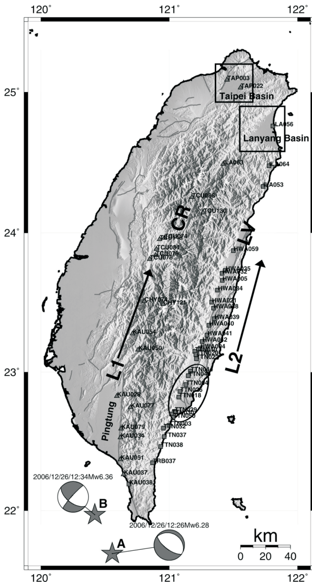
Fig. 1. Epicenters (stars) and focal mechanisms of 26 December 2006 Pingtung twin earthquakes (events A and B) offshore southwestern Taiwan. Solid lines depict the identified active faults in the area. Solid triangles and squares denote the seismic stations along lines L1 and L2 as mentioned in the text. The Taipei basin and the Lanyang basin are marked by two large open squares. The area with anomalously high PGA and PGV is marked by an ellipse.
