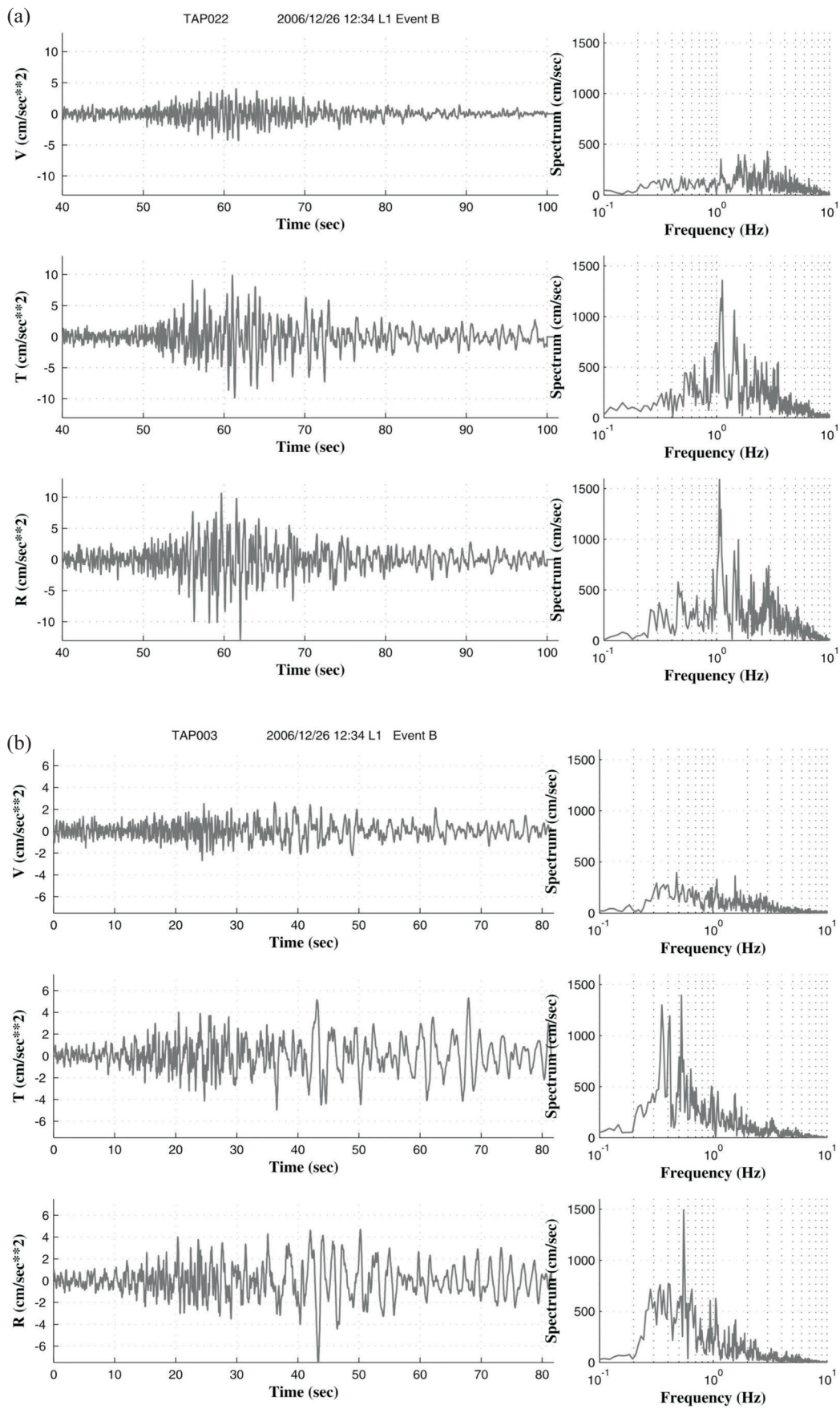
Fig. 8. The rotated three-component acceleration seismograms of the B event recorded at (a) TAP022 and (b) TAP003. The individual Fourier amplitude spectra are shown in the right panels.
