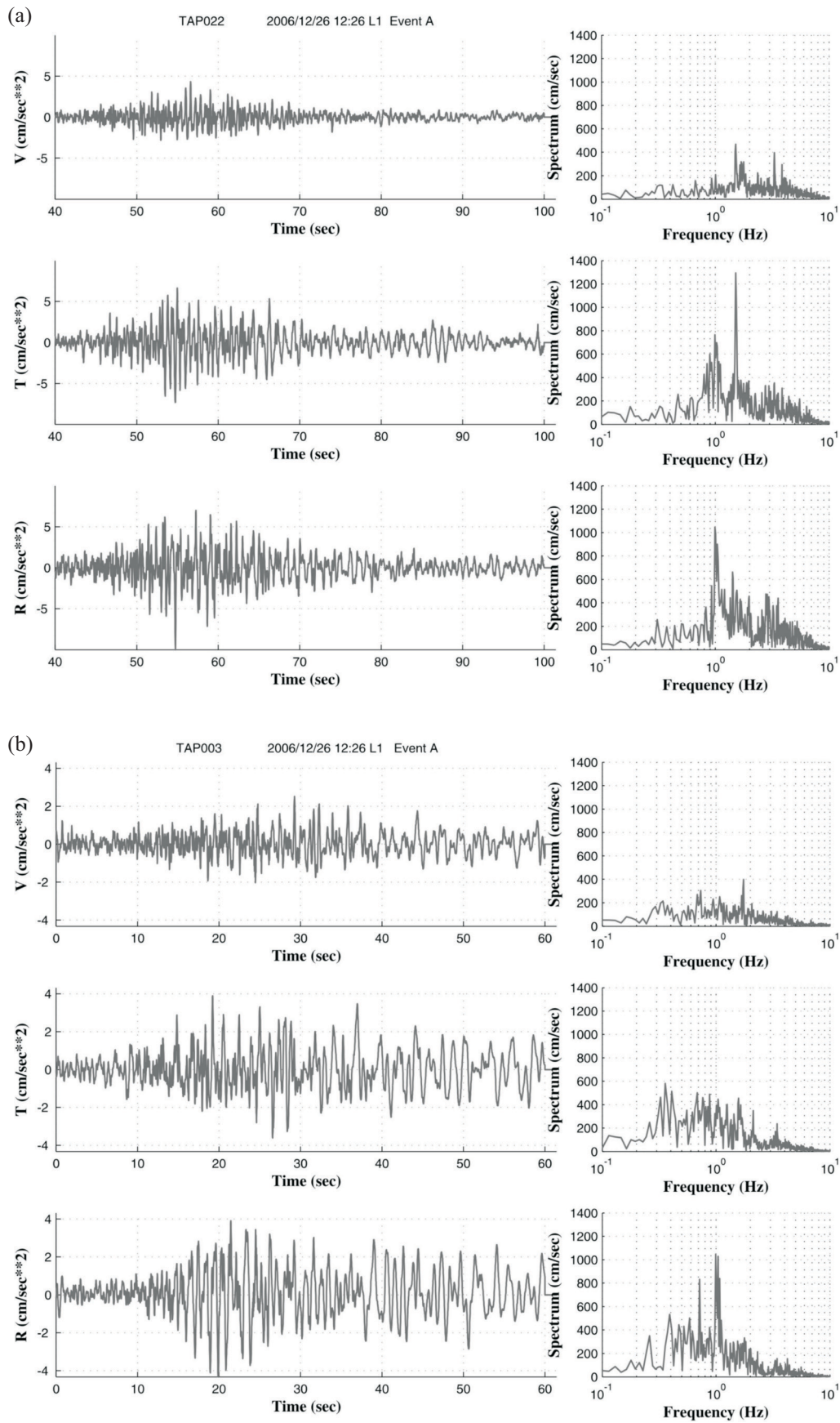
Fig. 6. The rotated three-component acceleration seismograms of the A event recorded at (a) TAP022 and (b) TAP003. The individual Fourier amplitude spectra are shown in the right panels.
