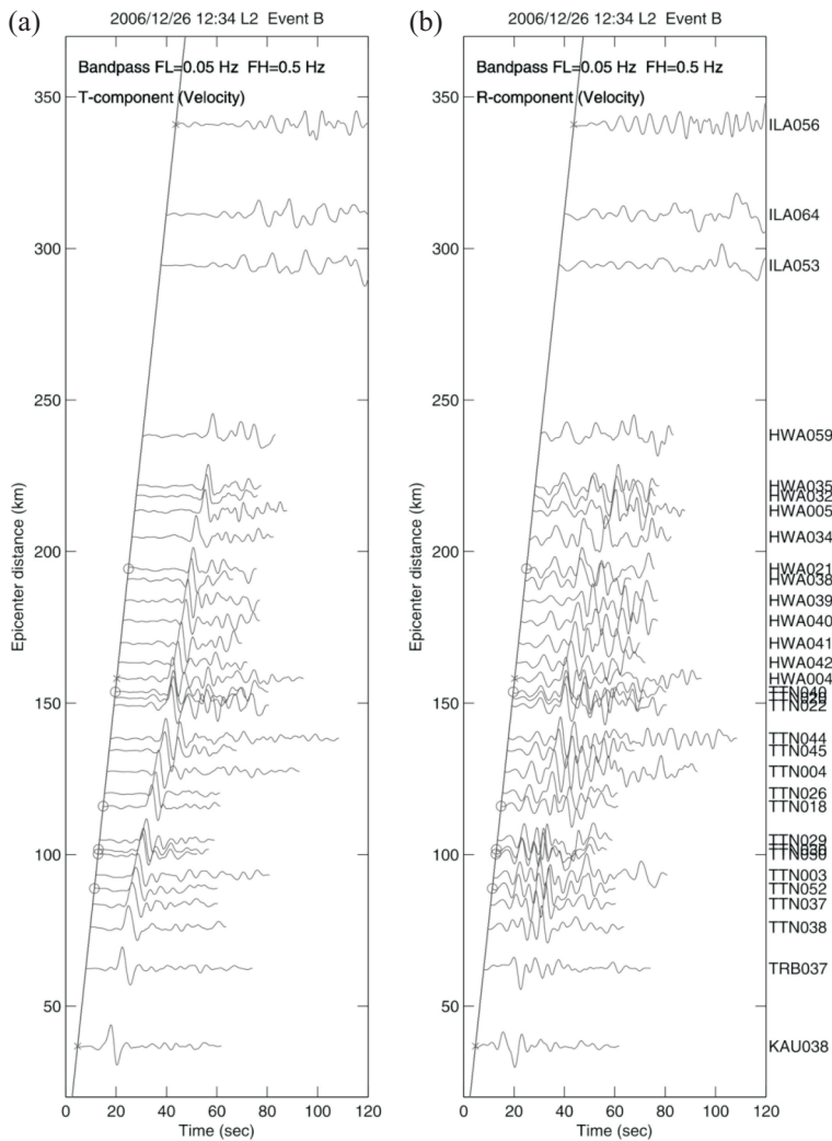
Fig. 4. (a) Transverse- and (b) radial-component ground velocity waveforms integrated from accelerograms for the B event observed at the stations along L2. Station names are shown at the right panel. All traces are filtered from 0.05 to 0.5 Hz. Site classification defined by Lee et al. (2001) is also shown at the beginning of each trace with the same symbols as shown in Fig. 3.
