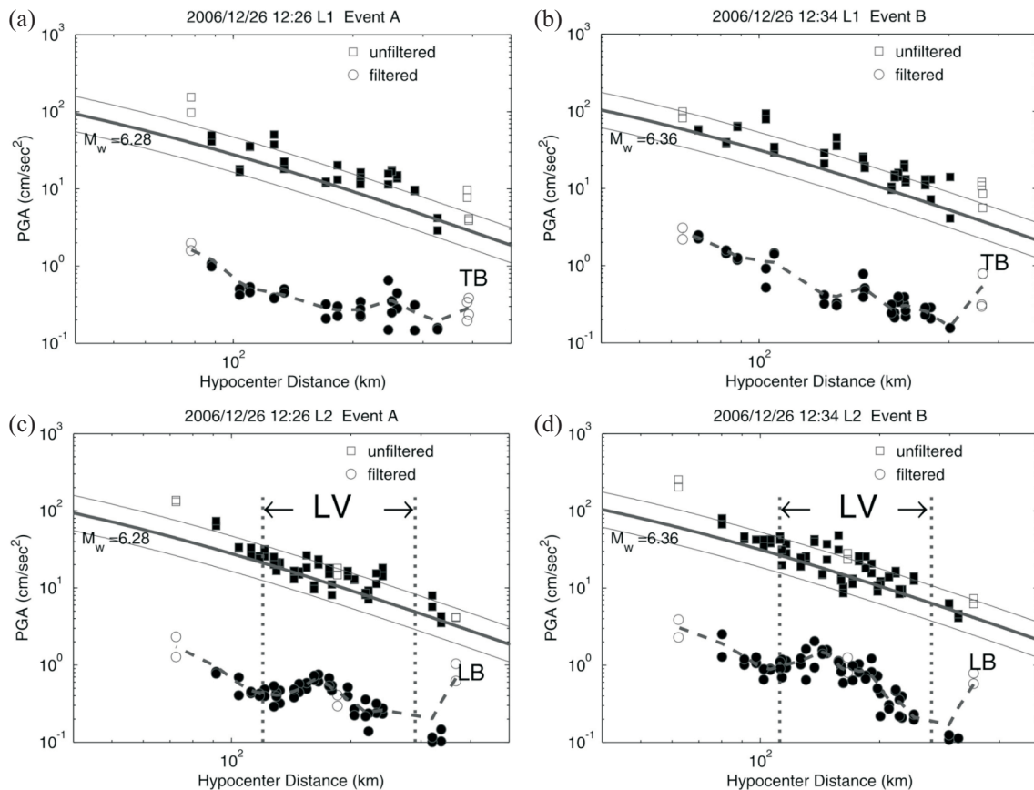
Fig. 3. Horizontal PGA as a function of distance: (a) and (b) along L1 for the A and B events and (c) and (d) along L2 for the two events. The squares and circles in each panel denote, respectively, unfiltered and filtered PGA. The solid and blank symbols indicate rock-type (Class-B and -C) and soil-type (Class-D and -E) sites, respectively. The thick and thin solid lines, respectively, depict the PGA attenuation curve and the standard deviation inferred by Lin and Lee (2008) for rock sites. The dashed line denotes the smoothing curve for the filtered PGA. Note that in addition to the amplification in the Taipei basin (TB) and the Lanyang basin (LB), the filtered PGA of both twin events show anomalously high values along the LV.
