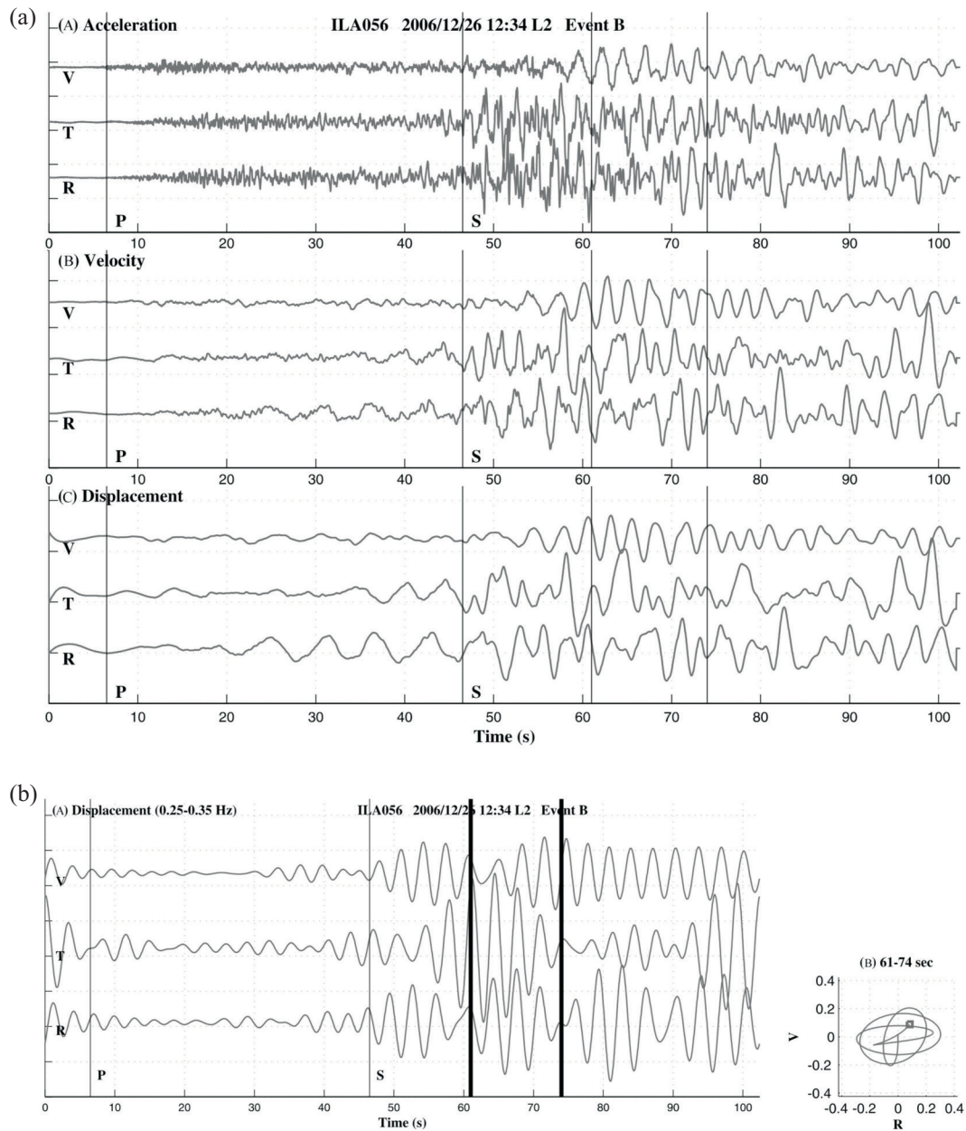
Fig. 13. (a) The rotated three-component accelerograms, velocity waveforms, and displacement waveforms of the B event recorded at ILA056; (b) The filtered displacement waveforms in the frequency band of 0.25 - 0.35 Hz and the particle motions in the time interval of 61 - 74 sec. Square refers to the start of particle motion.
