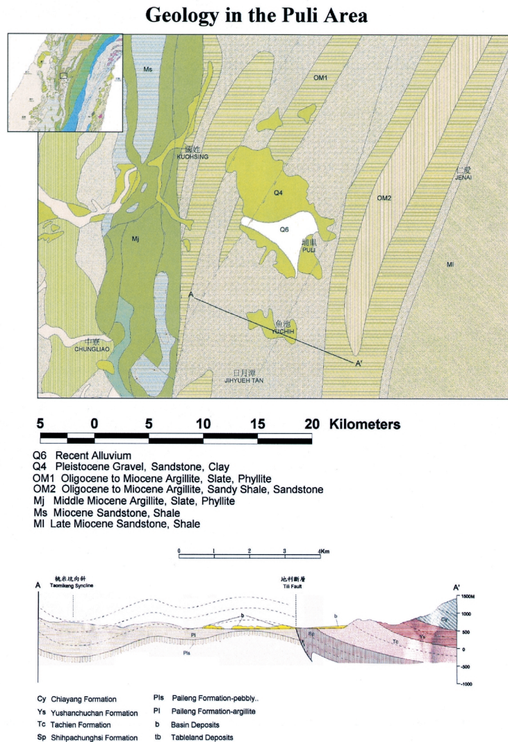
Fig. 3. Map sketching the geology of the Puli area and the geological section along line AA' near Puli (revised from Huang et al. 2000).
