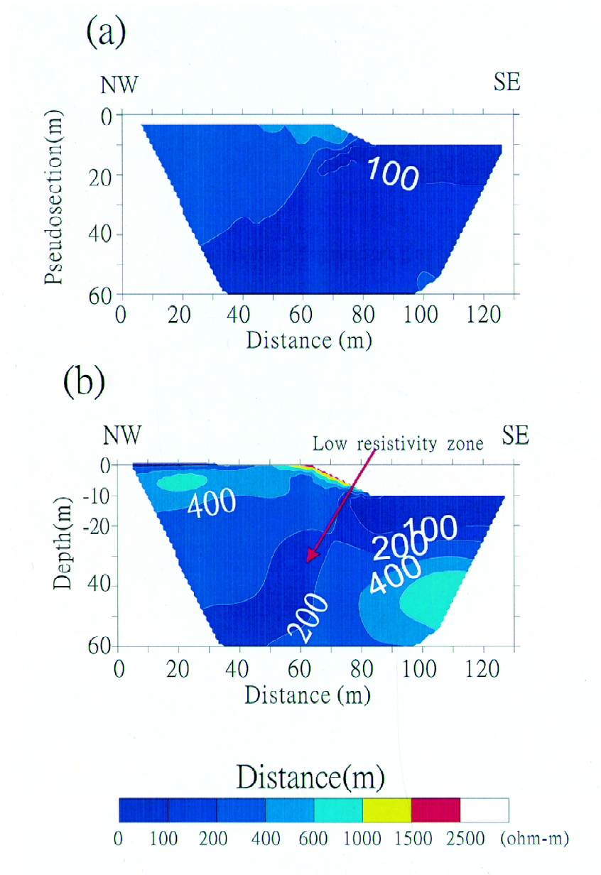
Fig. 7. (a) The apparent resistivity pseudosection of survey line L2. (b) The inversion result of the data shown in (a).
