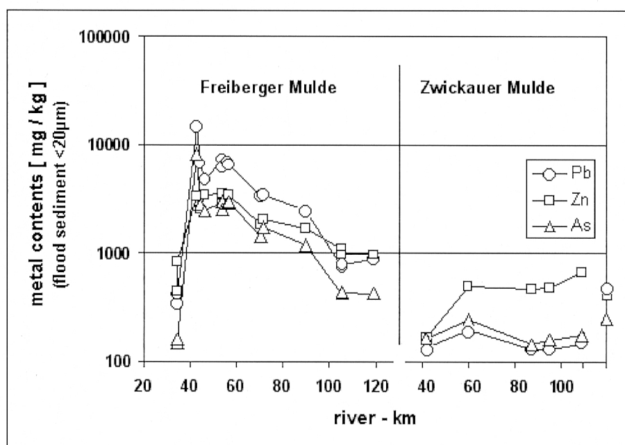
Fig. 2. As, Pb and Zn concentrations in the < 20 \mu\text{m} fraction of flood sediments along the length of the Freiburger Mulde and Zwickauer Mulde. Symbols at the right border of the graph refer to the United Mulde, about 2 kilometres downstream of the confluence.
