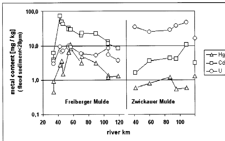
Fig. 3. Hg, Cd, and U concentrations in the < 20 μm fraction of flood sediments along the length of the Freiberger Mulde and Zwickauer Mulde. Symbols at the right border of the graph refer to the United Mulde, about 2 kilometres downstream of the confluence.
