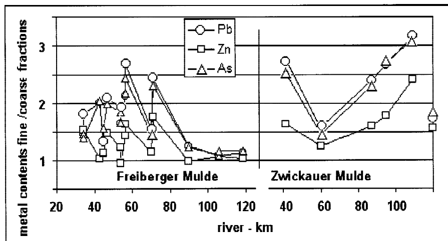
Fig. 4. Enrichment factors of Pb, Zn, and As in fine grained (< 20 μm) flood sediments relative to coarse grained (< 2 mm) flood sediments (note that the < 2 mm fraction contains also the (< 20 μm) fraction as explained in the text).
