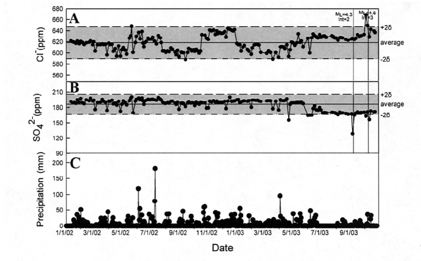
Fig. 3. Temporal variations of (A) \text{Cl}^- and (B) \text{SO}_4^{2-} concentrations in the 50-m deep Chingshan hot spring. The vertical lines represent the same as Fig. 2. (C) Daily precipitation recorded in the Chingshan rain gauge station (data from the CWBT).
