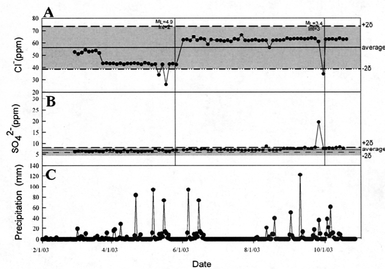
Fig. 6. Temporal variations of (A) \text{Cl}^- and (B) \text{SO}_4^{2-} concentrations in the Yuanshan hot spring. The vertical lines represent the same as Fig. 2. (C) Daily precipitation recorded in the Ilan rain gauge station (data from the CWBT).
