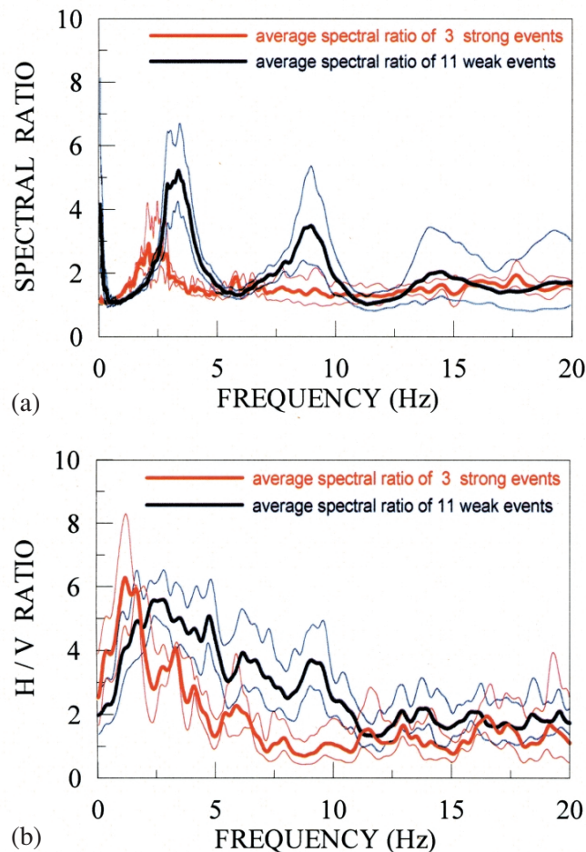
Fig. 1. (a) Strong and weak motion spectral ratios of surface to 11-m deep borehole station for the LSST array. (b) H/V spectral ratio for strong events (red line) and weak events (black line) for the same data used in (a). Thick line is the mean value and thin lines show the one standard deviation range. Red lines for strong motions and blue lines for weak motions.
