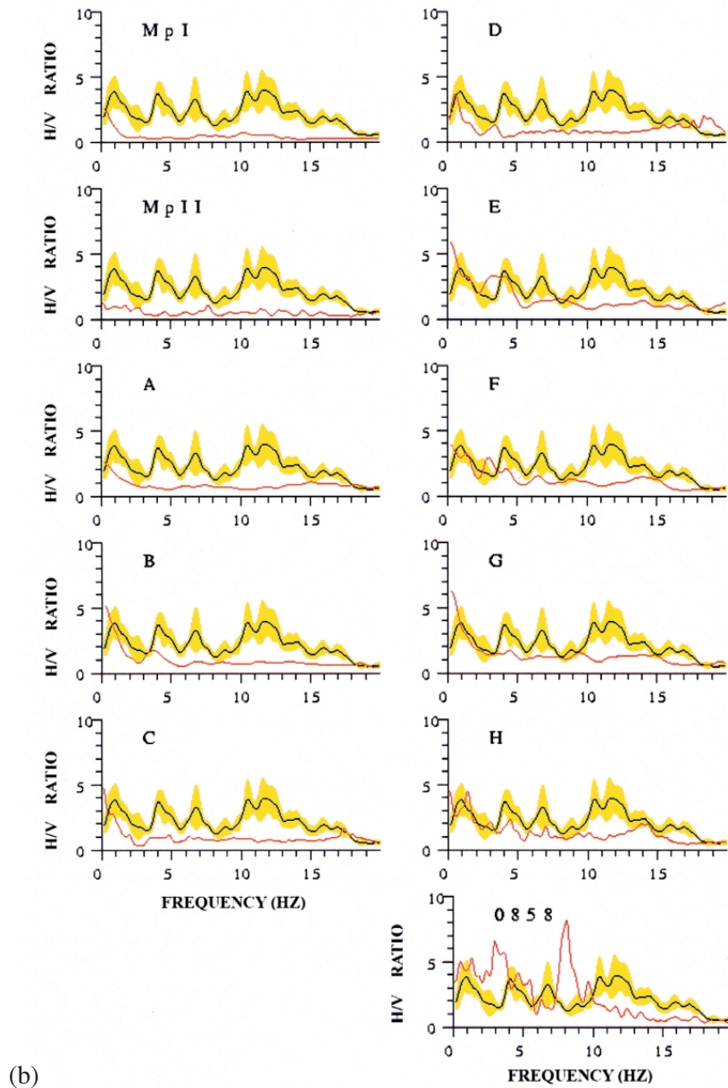
Fig. 6. Spectral ratios in the different time windows calculated from the mainshock and one aftershock of the 1995 Hyogo-ken Nanbu earthquake (red line). Time windows are the same as those in Fig. 5. Black line is the mean ratio of the weak motions before the Kobe mainshock and yellow area shows the one standard deviation area; (a) The results of surface to a 16-m deep borehole station pair are given and are the same as those of Aguirre and Irikura (1997). (b) The results of H/V ratios from the surface station.
