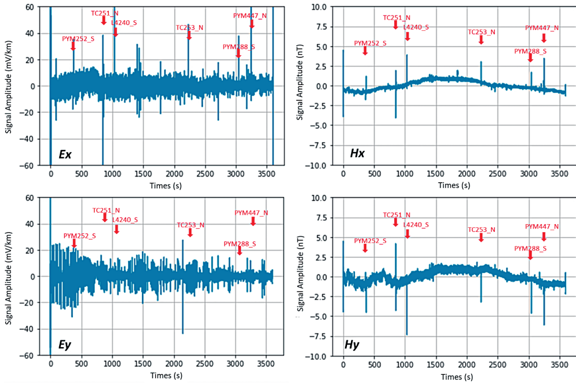
Fig. 5. The time series of the electric fields and magnetic fields collected between 22:00 and 22:59 on 12/21/17 at the RW010 station (after application of a power-line filter).
