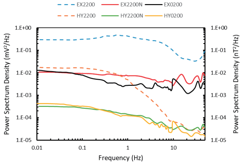
Fig. 10. The RW010 power spectra of the electric and magnetic fields collected during the 22:00-22:59 period on 12/21/17 for both the “only trains passing” contexts (EX2200 and HY2200) and the “no trains passing” contexts (EX2200N and HY2200N), and the RW010 power spectra of the background fields collected during the 02:00 - 02:59 period on 12/22/17 (EX0200 and HY0200).
