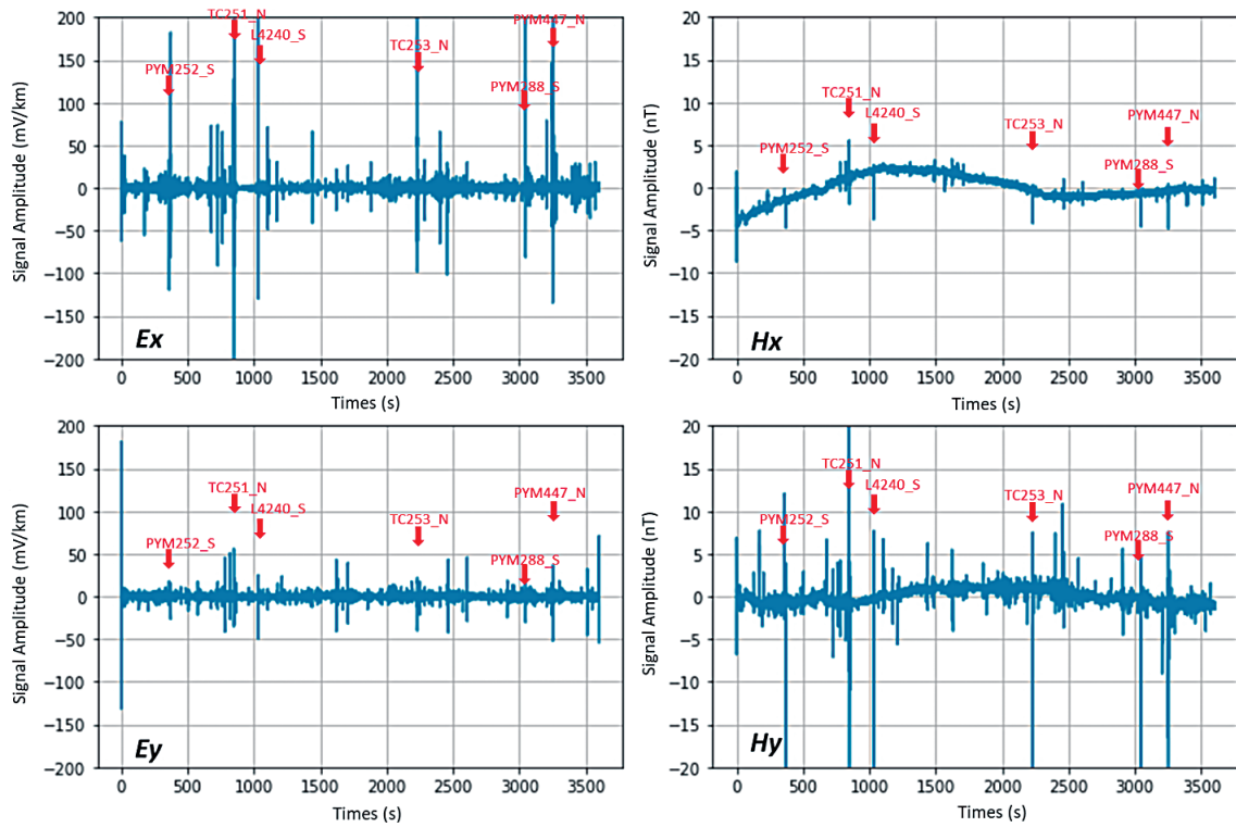
Fig. 3. The time series of the electric fields ( E_x and E_y ) and magnetic fields ( H_x and H_y ) collected between 22:00 and 22:59 on 12/21/17 at the RW002 station (after application of a power-line filter; the red arrows indicate the times of the trains' passing).
