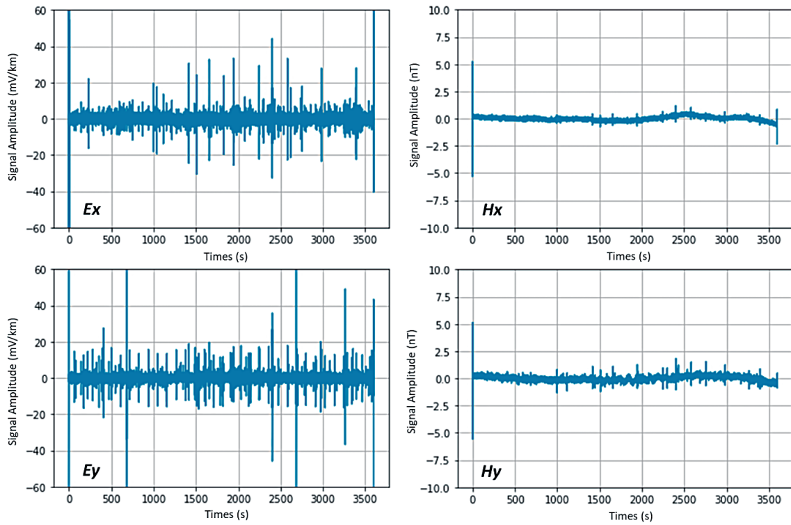
Fig. 7. The time series of the electric fields and magnetic fields collected between 02:00 and 02:59 on 12/22/17 at the RW010 station (after application of a power-line filter).
