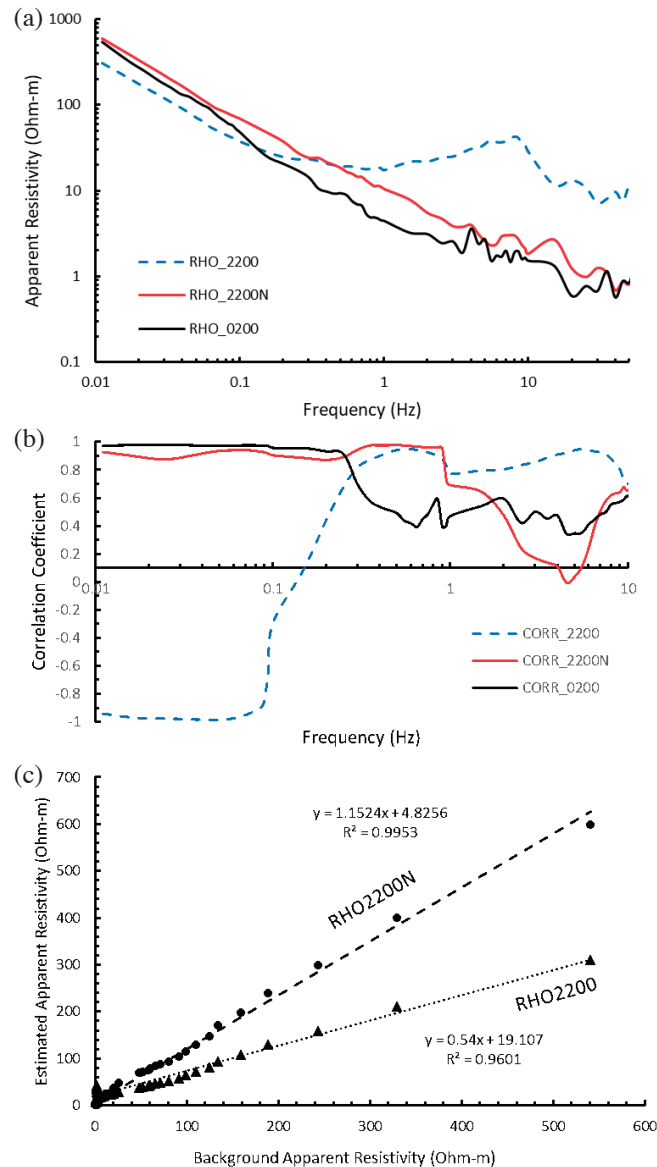
Fig. 12. (a) The RW010 apparent-resistivity measurements collected during the 22:00 - 22:59 period on 12/21/17 for both the “only trains passing” context (RHO_2200) and the “no trains passing” context (RHO_2200N), and the RW010 background-resistivity measurements (RHO_0200) collected during the 02:00 - 02:59 period on 12/22/17. (b) The correlation coefficients of the electric and magnetic spectra for the “only trains passing” context (CORR_2200) during the 22:00 - 22:59 period, the “no trains passing” context (CORR_2200N) during the 22:00 - 22:59 period, and the background context (CORR_0200) during the 02:00 - 02:59 period at RW002 on 12/22/17. (c) A comparison of the estimated apparent resistivities of RHO_2200 and RHO_2200N with the background resistivities of RHO_0200 at the RW010 site for frequencies less than 1 Hz.
