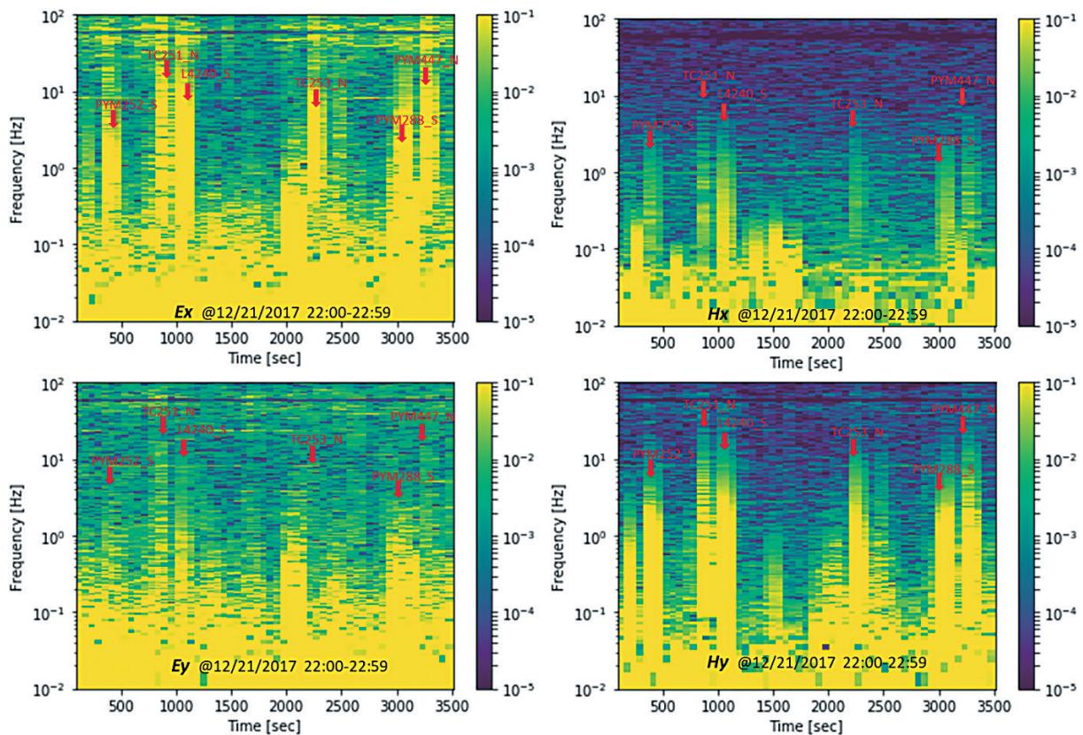
Fig. 4. The frequency-time spectrum maps of the electric and magnetic fields collected between 22:00 and 22:59 on 12/21/17 at the RW002 station.
