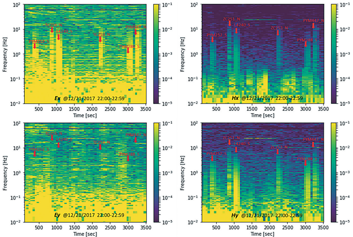
Fig. 6. The frequency-time spectrum maps of the electric and magnetic fields collected between 22:00 and 22:59 on 12/21/17 at the RW010 station.
