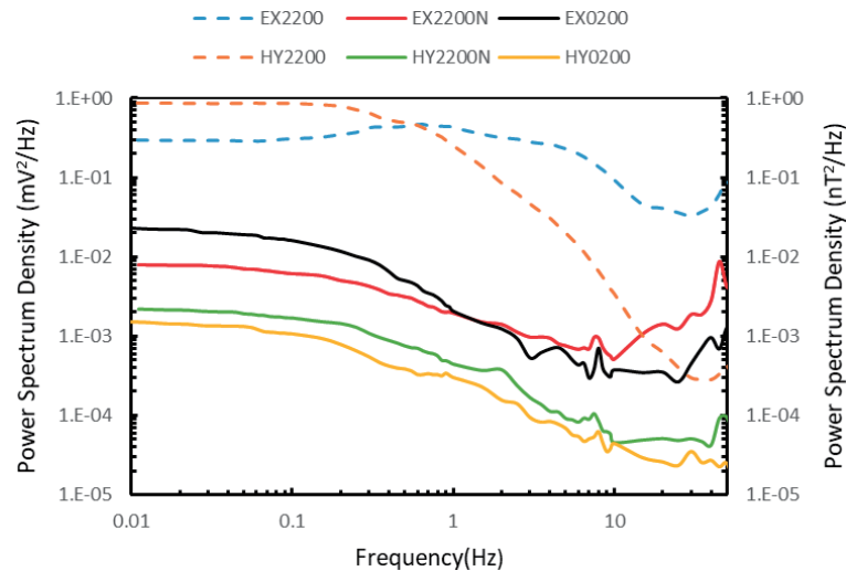
Fig. 9. The RW002 power spectra of the electric and magnetic fields collected during the 22:00 - 22:59 period on 12/21/17 for both the “only trains passing” contexts (EX2200 and HY2200) and the “no trains passing” contexts (EX2200N and HY2200N), and the RW002 power spectra of the background electric and magnetic fields collected during the 02:00-02:59 period on 12/22/17 (EX0200 and HY0200).
