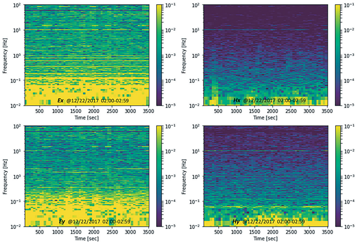
Fig. 8. The frequency-time spectrum maps of the electric and magnetic fields collected between 02:00 and 02:59 on 12/22/17 at the RW010 station.
