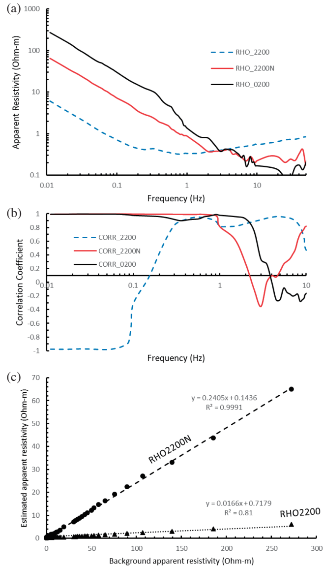
Fig. 11. (a) The RW002 apparent-resistivity measurements collected during the 22:00 - 22:59 period on 12/21/17 for both the “only trains passing” context (RHO_2200) and the “no trains passing” context (RHO_2200N), and the background-resistivity measurements collected during the 02:00 - 02:59 period on 12/22/17 (RHO_0200). (b) The correlation coefficients of the electric and magnetic spectra for the “only trains passing” context (CORR_2200) during the 22:00 - 22:59 period, the “no trains passing” context (CORR_2200N) during the 22:00 - 22:59 period, and the background context (CORR_0200) during the 02:00 - 02:59 period at RW002 on 12/22/17. (c) A comparison of the apparent resistivities of RHO_2200 and RHO_2200N with the background resistivities of RHO_0200 at the RW010 site for frequencies less than 1 Hz.
