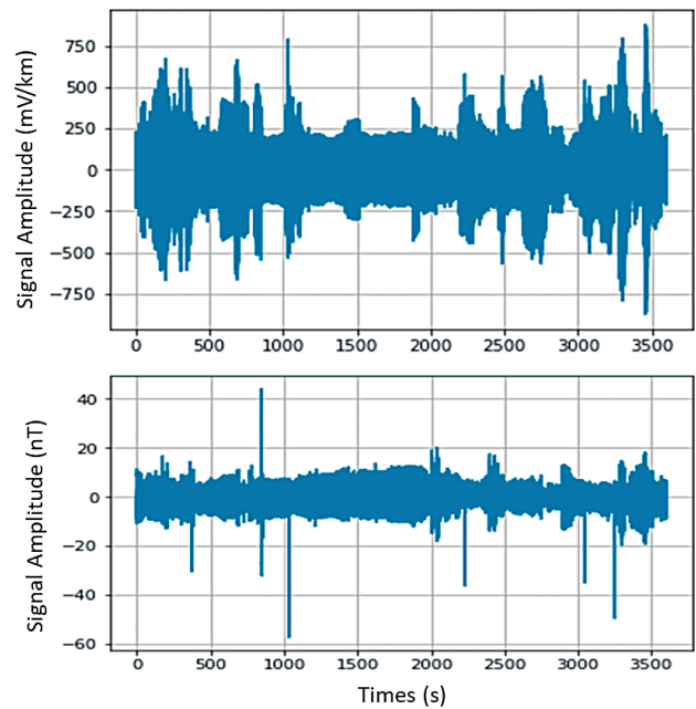
Fig. 2. The time series of the electric field perpendicular to the track ( E_x ) and the magnetic field parallel to the track ( H_y ) collected between 22:00 and 22:59 on 12/21/17 at the RW002 station (without filtering).
