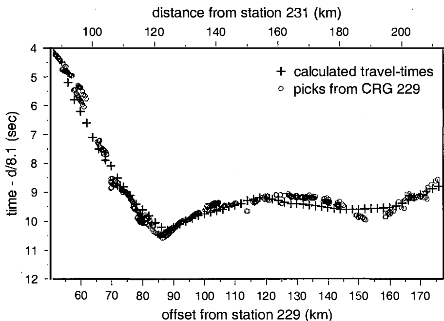
Fig. 10. Calculated travel-times (crosses) of all refracted P waves compared to the observed travel-times (open circles) in the common receiver gather of station 229.
