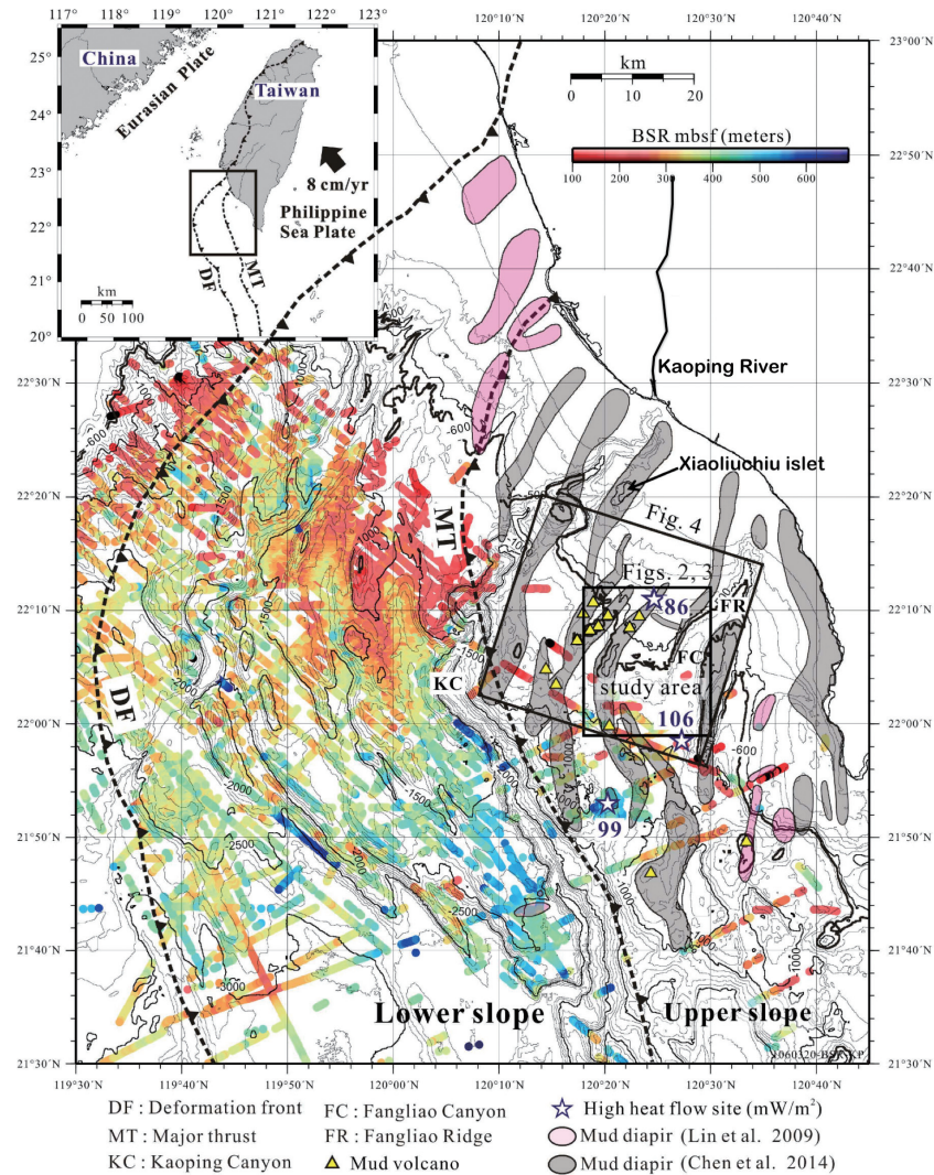
Fig. 1. Tectonic feature, bathymetry and related structures off SW Taiwan. Upper panel shows the regional topography and tectonic features. The deformation front (DF) separates the passive continental margin in the west and active accretionary wedge in the east. The major thrust (MT) separates the lower slope and upper slope of the accretionary wedge. The solid boxes indicate our study area. The distribution of the bottom simulating reflector (BSR) of Liu et al. (2006) is shown by the color scale. MBSF: meters below seafloor.
