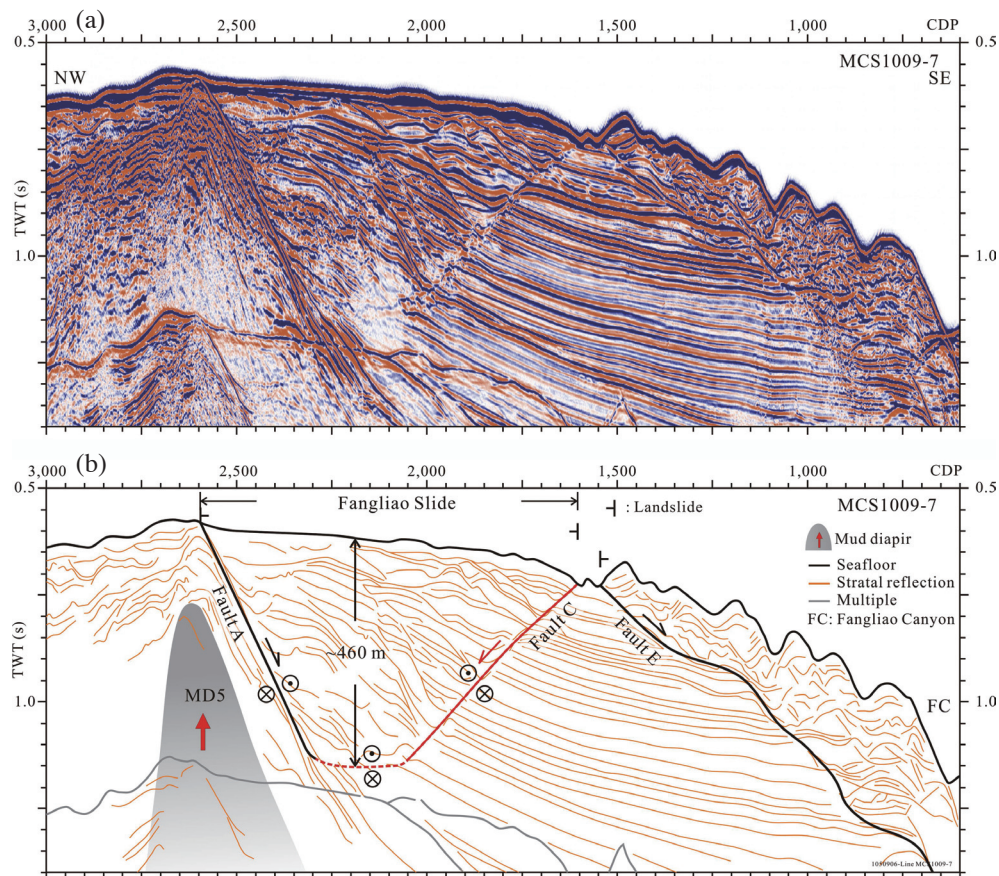
Fig. 6. (a) MCS profile MCS1009-7 and (b) the seismic interpretation. The upper portion of the Fangliao Slide shows a wedged shape; the wedge is bounded by fault A in the west and fault C in the east. See the profile location in Fig. 3.
