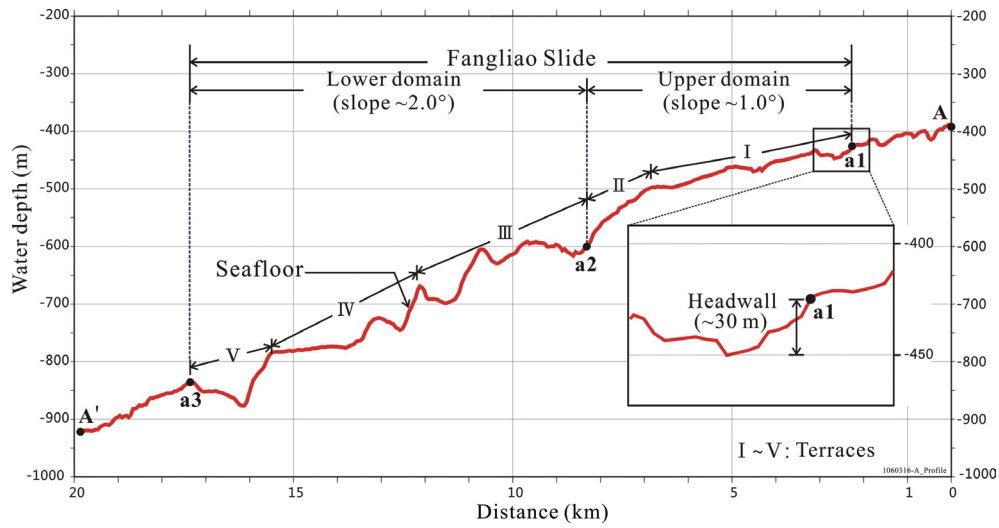
Fig. 5. A bathymetric profile along the sliding direction of the Fangliao Slide. The headwall has ~30 m vertical offset. The upper domain contains terraces I and II with a gentle slope of \sim 1^\circ . The lower domain contains terraces III to V with a slightly steeper slope of \sim 2^\circ . The profile location is shown in Fig. 2.
