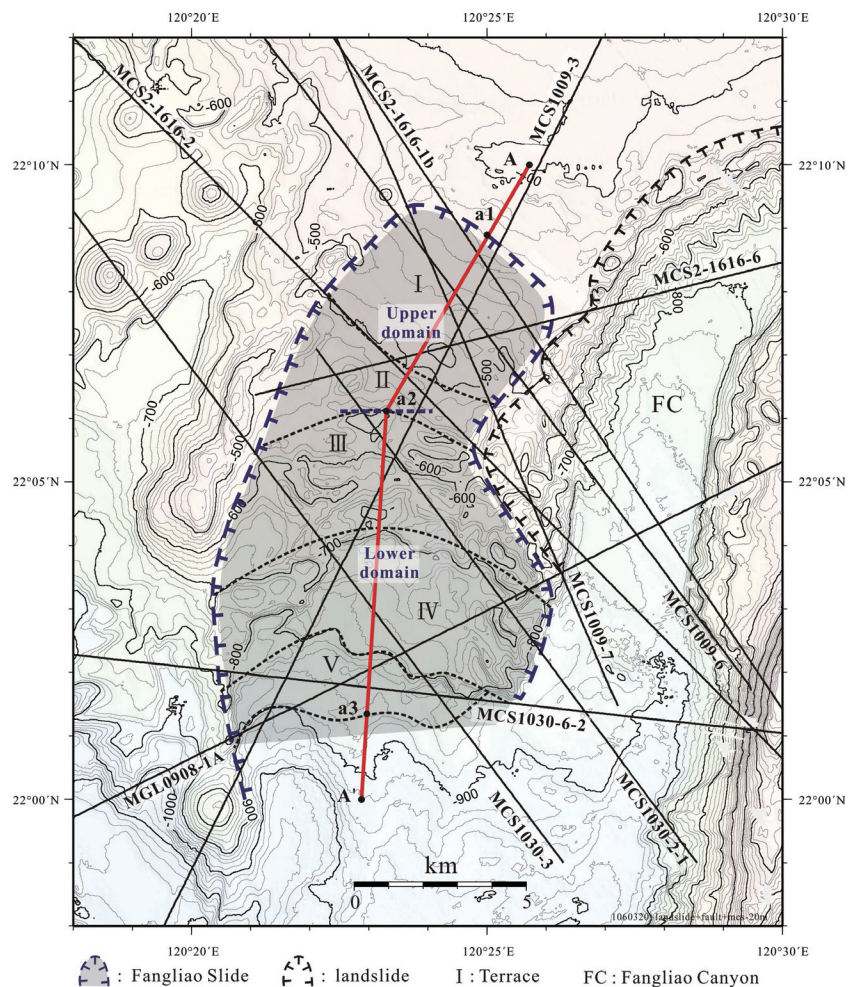
Fig. 2. Distribution of the seismic reflection profiles used in this study. Black lines are seismic profiles. The red line is the track of the bathymetric profile shown in Fig. 5.
