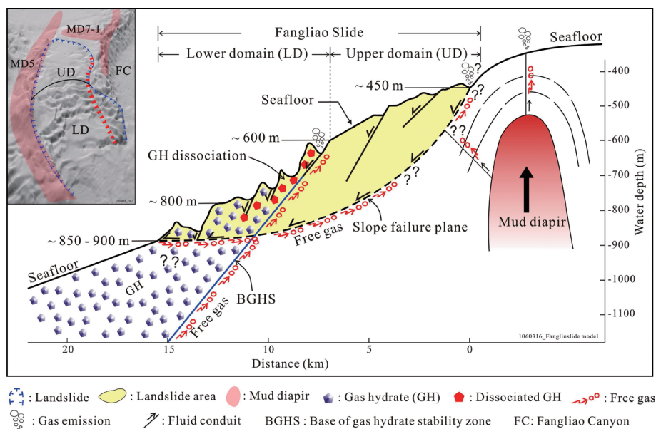
Fig. 11. A schematic model explains the sliding scenario of the Fangliao Slide. Mud diapirism and gas hydrate dissociation are two main factors for the slope failure of the Fangliao Slide. The slope failure was first triggered by mud diapirism. Free gas came out of the mud diapir could enhance the slope failure. Secondly, the gas hydrate dissociation and upward free gases could augment the slope failure in the lower domain resulting more corrugated seafloor.
