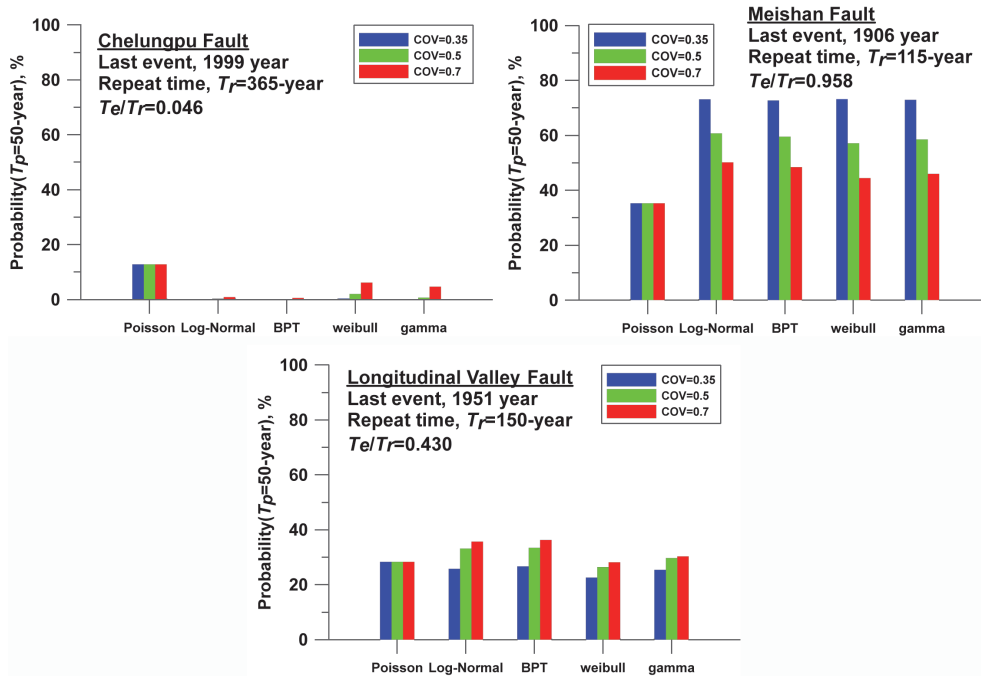
Fig. 10. The next 50-year conditional probabilities for earthquake occurrence for the Chelungpu, Meishan and Longitudinal Valley faults. A mean 365-year recurrence time is assumed for the Chelungpu fault, a mean 115-year recurrence time for the Meishan fault, and a mean 150-year recurrence time for the Longitudinal Valley fault. Graphs show the results using five distributions with COV = 0.35, 0.5, and 0.7. (Color online only)
