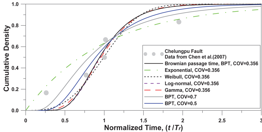
Fig. 7. Comparison of the five distributions and the recurrence-time data from paleoseismological investigation of the Chelungpu fault, including COV = 0.356. In addition, the BPT distribution using COV = 0.5 and 0.7 are also plotted. (Color online only)
