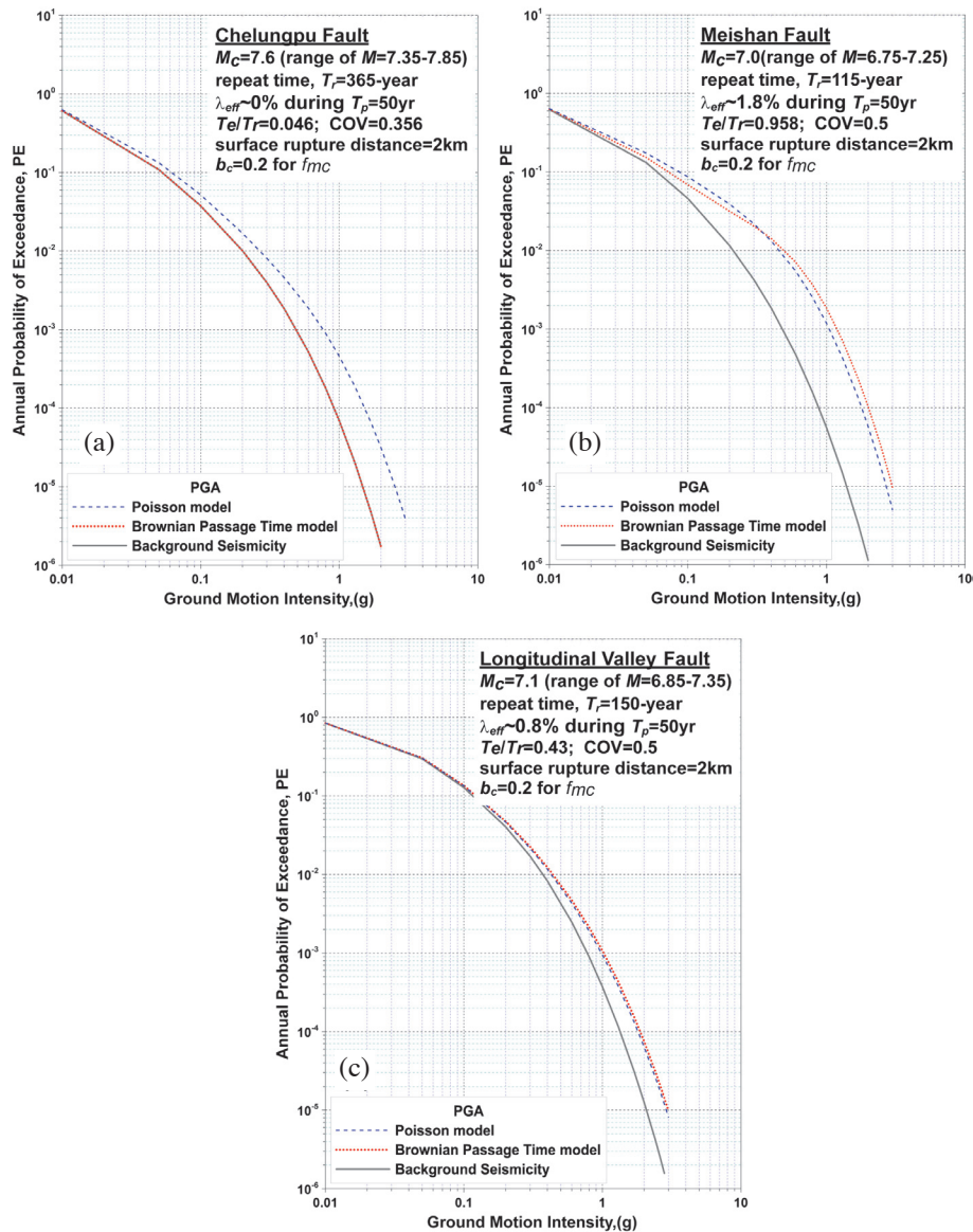
Fig. 12. Comparison of the PGA hazard curves using the time-independent and time-dependent models for the Chelungpu (a), the Meishan (b), and the Longitudinal Valley (c) faults. The study site is located on the footwall of the fault. Five NGA-West2 GMPEs are used and assumed the V_{S30} = 760 \text{ m s}^{-1} . (Color online only)
