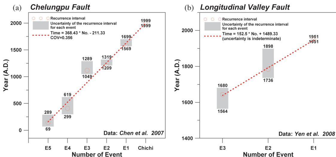
Fig. 5. The paleoseismological fault data and its mean occurrence interval. On the (a) is the recurrence interval of the Chelungpu fault was estimated about 365 years, and the (b) is the recurrence interval of the Longitudinal Valley fault was estimated about 150 years. (Color online only)
