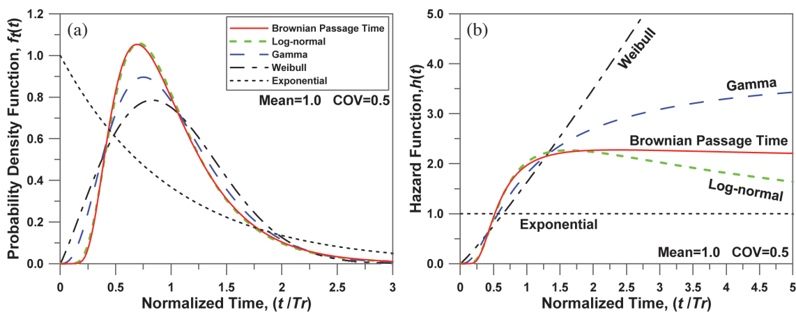
Fig. 6. (a) Probability density distribution and (b) the Hazard function of the Exponential (Poisson) model, Brownian Passage Time model, Log-normal model, Gamma model, and Weibull model. All distributions have mean = 1 and standard deviation = 0.5 (except the exponential distribution). (Color online only)
