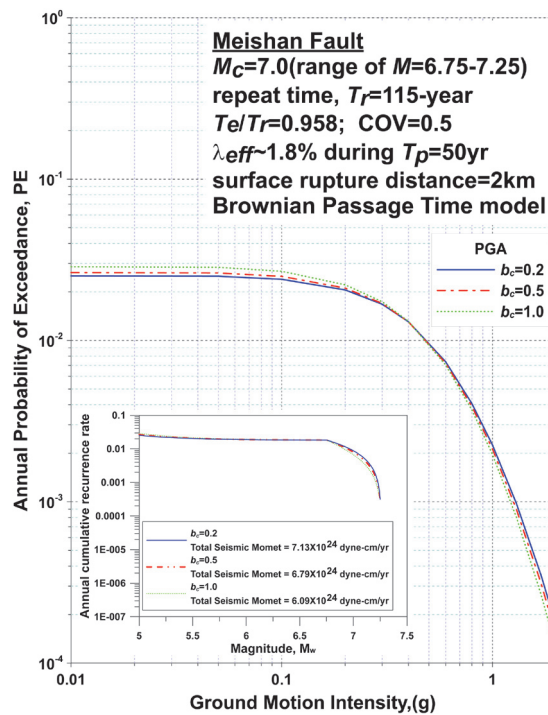
Fig. 14. Comparison of the PGA hazard curves for a site near the Meishan fault between considering different b_c -value in the truncated exponential model, f_{mc}(m) , for the characteristic earthquake range. The cumulative probability density function of magnitude for describing the relative rate of earthquakes are compared. (Color online only)
