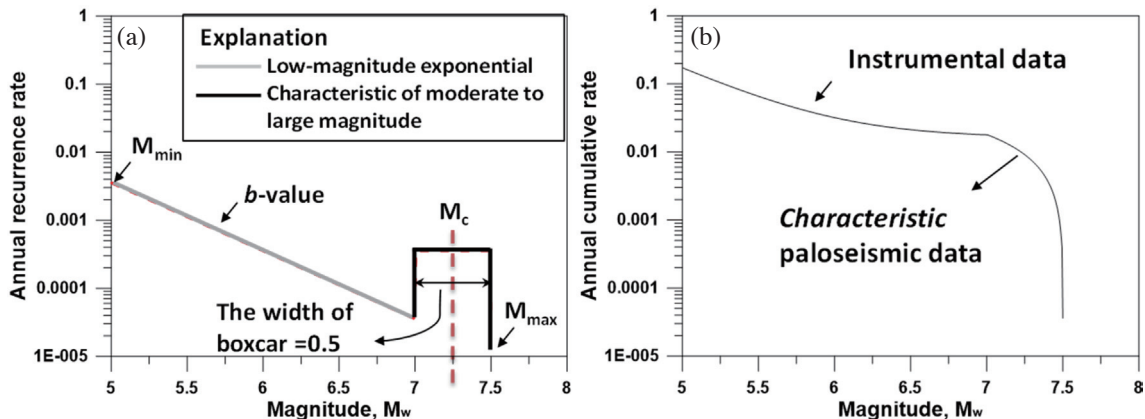
Fig. 3. The Characteristic Earthquake Model from Youngs and Coppersmith (1985). On the (a) is the schematic illustration of the characteristic earthquake model; the (b) is the cumulative probability density magnitude of the model. (Color online only)
