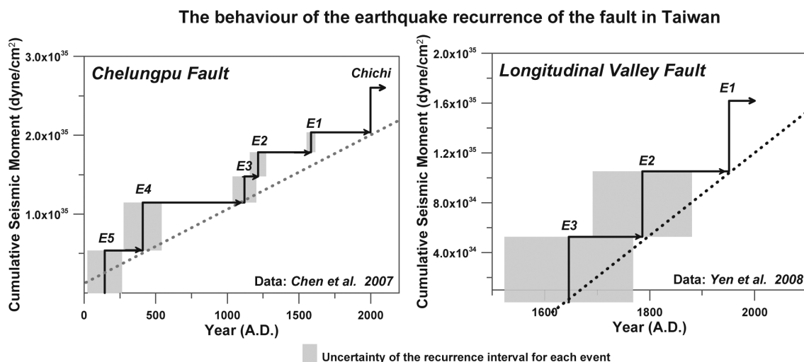
Fig. 4. The behaviour of the earthquake recurrence in the Chelungpu fault (left) and the Longitudinal Valley fault (right) in Taiwan follows the time-predictable model based on a consistent slip rate level at which failure occurs. In this figure, the moment magnitude scale referring from Hanks and Kanamori (1979): M = 2/3 \cdot \log M_0 - 10.7 .
