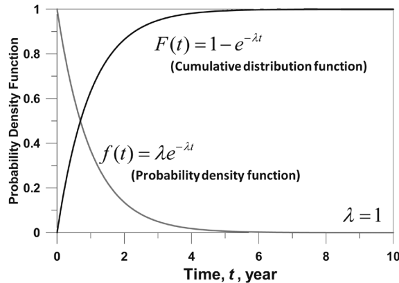
Fig. 2. The probability density function (pdf) and cumulative distribution function (PDF) of Poisson process.
