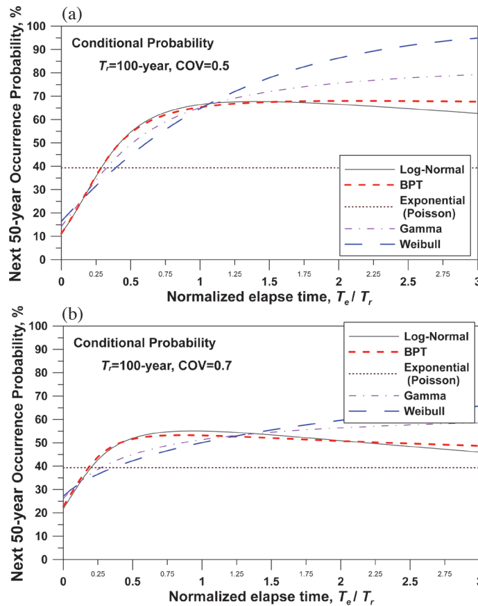
Fig. 11. Comparison of the five probability models used in estimated the next 50-year ( T_p ) conditional probabilities of earthquake occurrence for example. All models have mean = 100 years and COV = 0.5 for (a) and 0.7 for (b). (Color online only)
