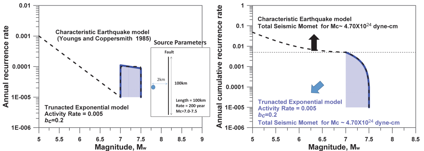
Fig. 9. Schematic illustration of the comparison of earthquake recurrence between the characteristic earthquake model and the truncated exponential model. The fault source parameters include that the repeat time is 200-year and the characteristic magnitude range is 7.0 - 7.5. The b_c -value = 0.2 is assumed in the truncated exponential model (blue area). The left is the recurrence rate of each magnitude; the right is the cumulative recurrence rate of each magnitude. (Color online only)
