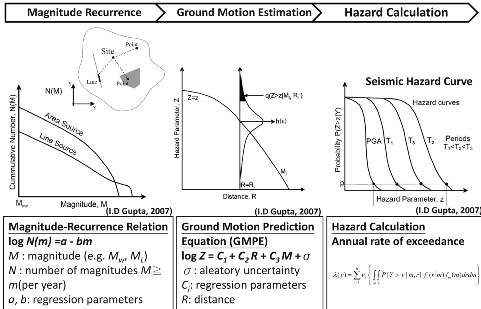
Fig. 1. Schematic illustration of the basic three steps in probabilistic seismic hazard analysis.
