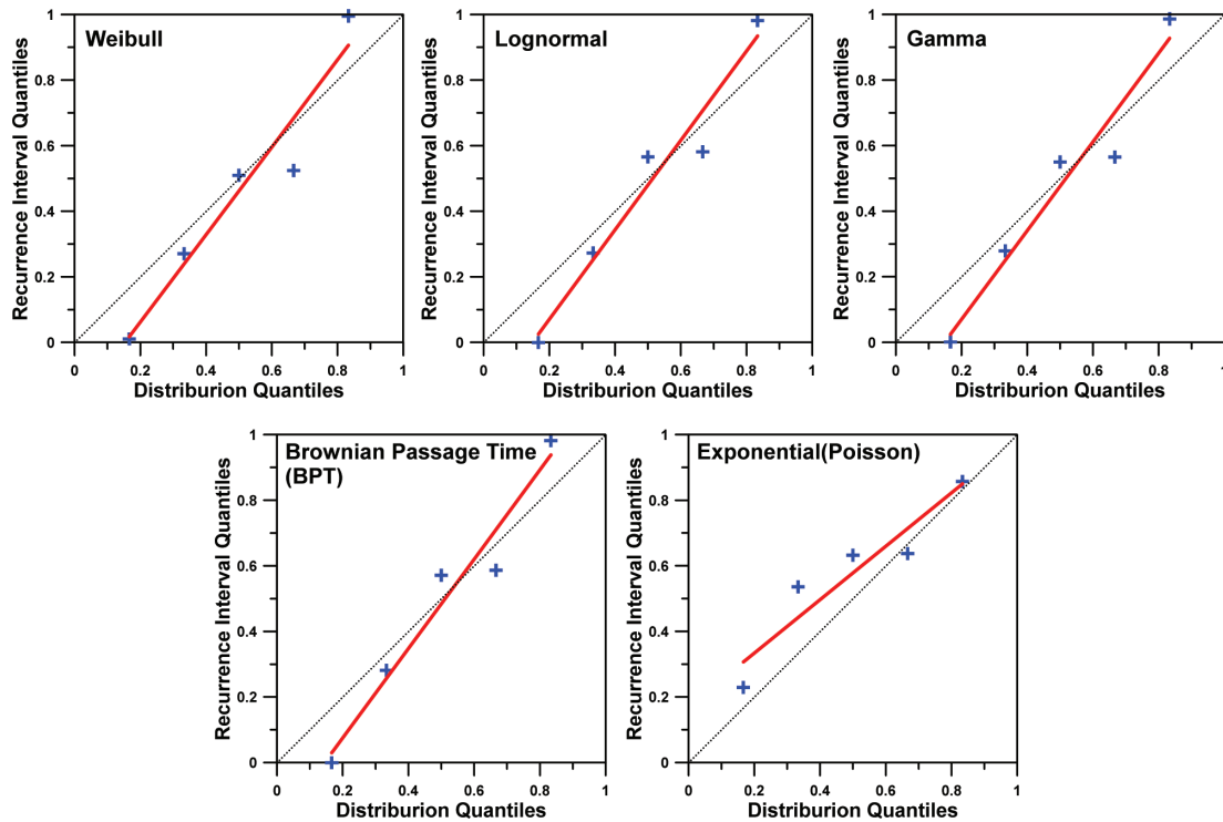
Fig. 8. The QQ-plots of the paleoearthquake data of the Chelungpu fault and the five distribution models. The distribution models include the Weibull model, Log-normal model, Gamma model, Brownian Passage Time model, and Exponential (Poisson) model. Assuming COV = 0.356 of the Chelungpu fault. In the plot, the sample data is displayed with the plot symbol '+' and the red line is a robust linear fit of the order statistic of the two samples. In the test, the results shows that the robust linear of renewal models fit more closely to the line of 1:1 than the Poisson model fitting. (Color online only)
