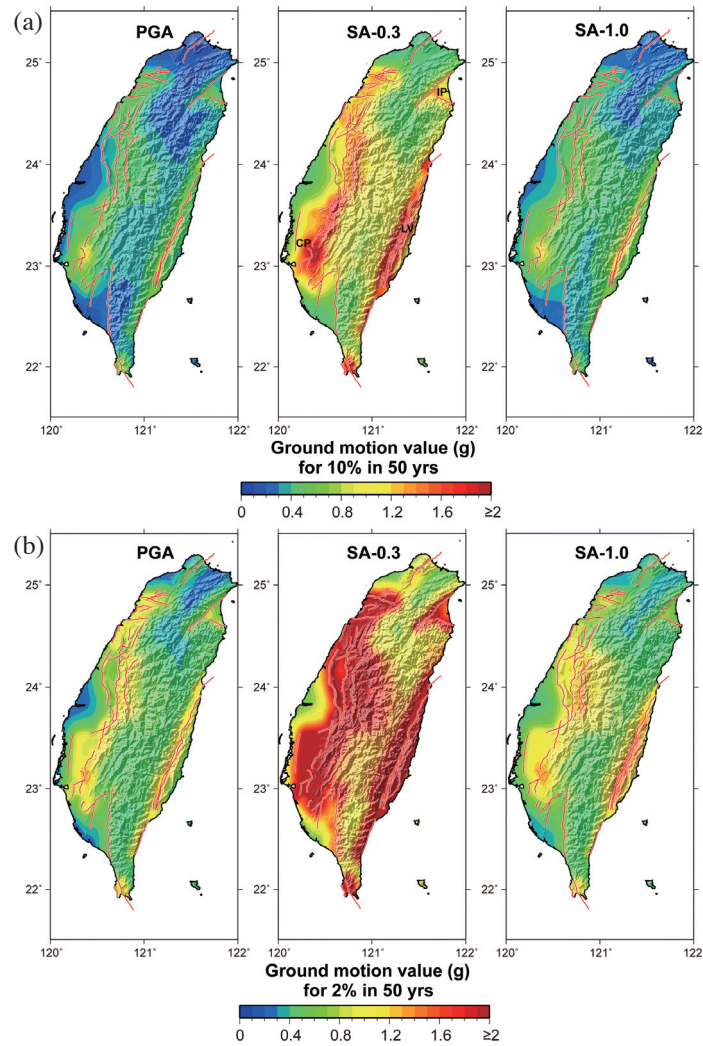
Fig. 5. Hazard maps of PGA, Sa at 0.3 s (SA-0.3), and Sa at 1.0 s (SA-1.0) for (a) 10% PoE in 50 years (corresponding to a recurrence interval of 475 years) and (b) 2% PoE in 50 years (correspondence to a recurrence interval of 2475 years) based on the parameters of TEM seismogenic structures. Locations of Chianan Plain, Ilan Plan, and Longitudinal Valley are denoted by CP, IP, and LV, respectively. (Color online only)
