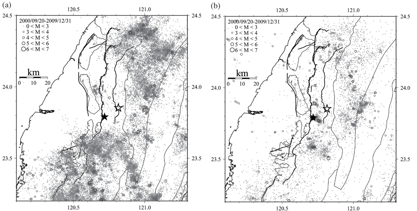
Fig. 9. Seismicity (a) above and (b) below 15 km depth one year after the 1999 Chi-Chi earthquake (open star). The solid star denotes the 2009 Mingjian earthquake. Thin lines indicate the geological boundaries, and bold lines are active faults.
