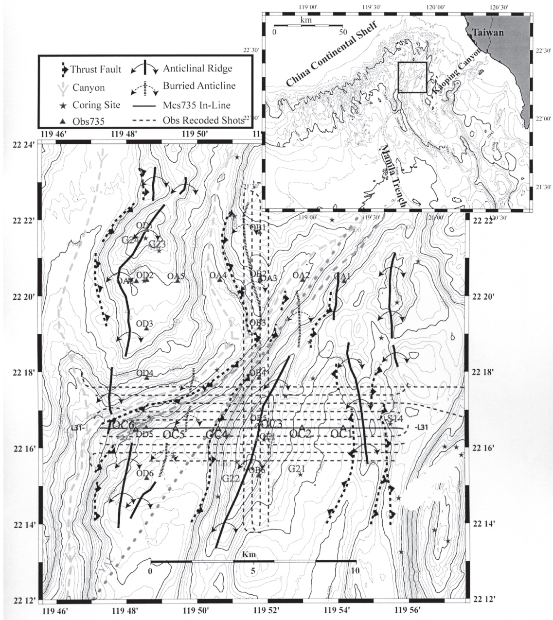
Fig. 1. Structural setting and combined MCS/OBS seismic layout. The OBS locations are marked by triangles. MCS735 shots recorded by the OBS transect C are marked with dashed lines, and the MCS735-31 in-line with a thick line.
