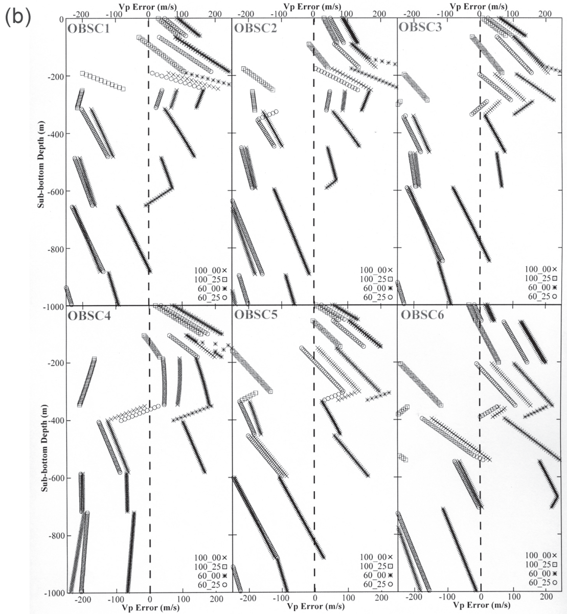
Fig. 8b. Residual acoustic velocities (“observed” - modeled) as predicted from the shear-wave and acoustic velocity profiles beneath OBSs from the effective medium theory for hydrate and quartz-free sediments (crosses), 25% hydrate (squares), 60% clay (stars), and 25% hydrate and 60% clay (circles).
