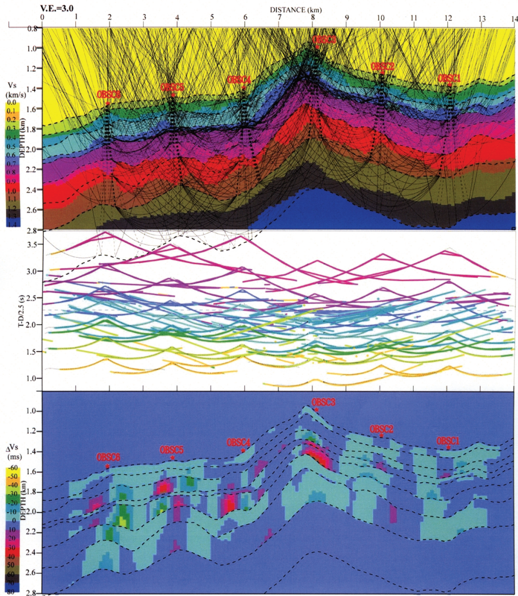
Fig. 4. a) Subset of the 24721 rays and shear-wave velocity model of the P-S inversion. The up-going S ray paths are plotted with dashed lines. b) Modeled times are plotted with lines, observed times are marked with small bars representative of the 10 ms data incertitude. c) Deviation from the initial constant gradient model. OBS locations are indicated with stars.
