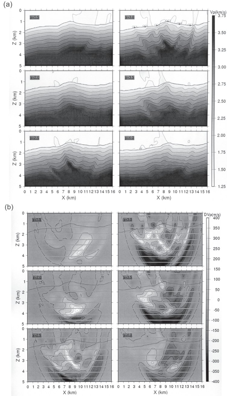
Fig. 6. a) Vertical cross sections of the final acoustic velocity model between 1.5 and 4.0 km cross line. b) Vertical cross sections of deviation from the initial model. The sea-floor is marked by a thick line. OBS locations are indicated with circles on the y = 3 km section.
