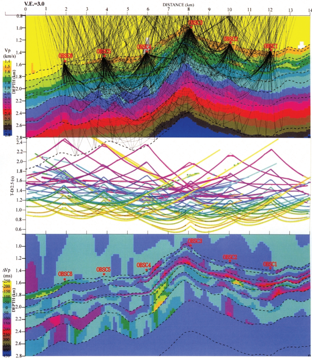
Fig. 3. a) Subset of the 24721 rays and acoustic velocity model for the P-P inversion. b) Modeled times are plotted with lines, observed times are marked with small bars representative of the 10 ms data incertitude. c) Deviation from the initial constant gradient model. OBS locations are indicated with stars.
