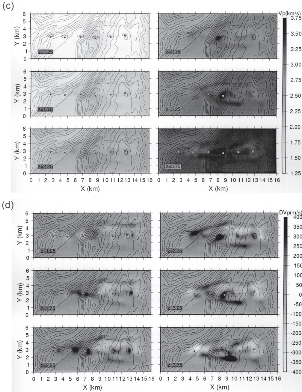
Fig. 6 (Continued). c) Horizontal cross sections of the final model between 1.25 and 3.75 km depth. d) Horizontal cross sections of the deviation from the initial model, plotted along rays. Bathymetric data is contoured at 50-m intervals. OBS locations are indicated with circles.
