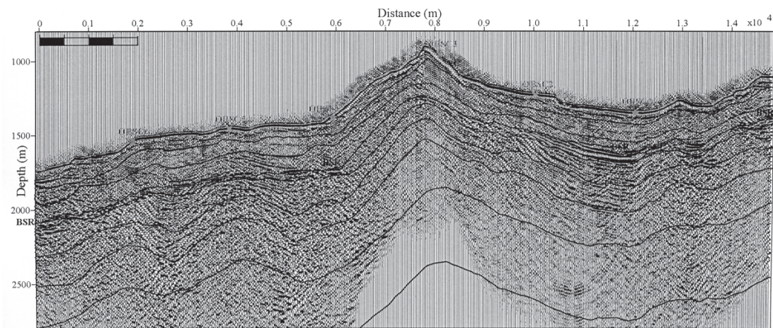
Fig. 2. Post-stack depth migrated section MCS735-31. A total of 9 horizons are digitized for the node-based velocity model. OBS locations are indicated with crosses.
