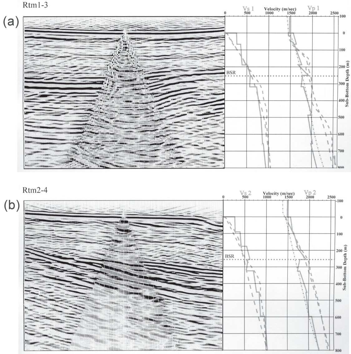
Fig. 7. Seismic depth images from component RTM migration of the OBS records overlain on the MCS735 in-line depth migrated section, and acoustic and shear-waves velocities resulting from the 1-D RMS analysis of the 4 OBS datumed components (dashed lines), the 2-D RauInvr inversion, and the 3-D first arrival tomographic inversion (dash-dotted lines). The seismic images have no vertical exaggeration. a) OBSC1-3 horizontal component. b) OBSC2-4 vertical component. c) OBSC3-1 hydrophone component. d) OBSC4-2 horizontal component. e) OBSC5-1 hydrophone component. f) OBSC6-2 horizontal component.
