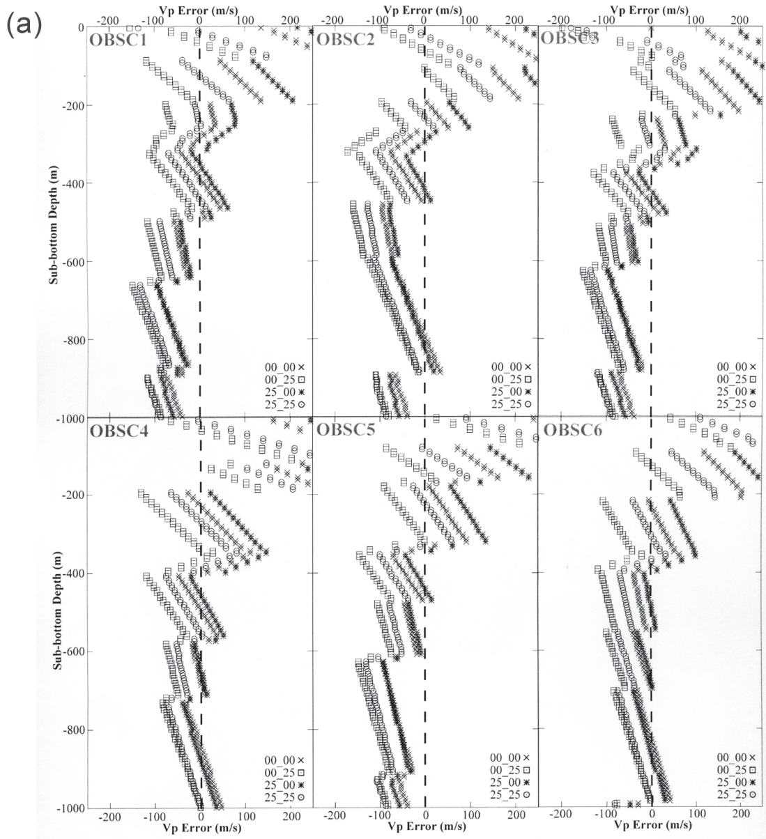
Fig. 8a. Residual acoustic velocities (“observed” - modeled) as predicted from the shear-wave and acoustic velocity profiles beneath OBSs from the weighted equation for hydrate and clay-free sediments (crosses), 25% hydrate (squares), 25% clay (stars), and 25% hydrate and clay (circles).
