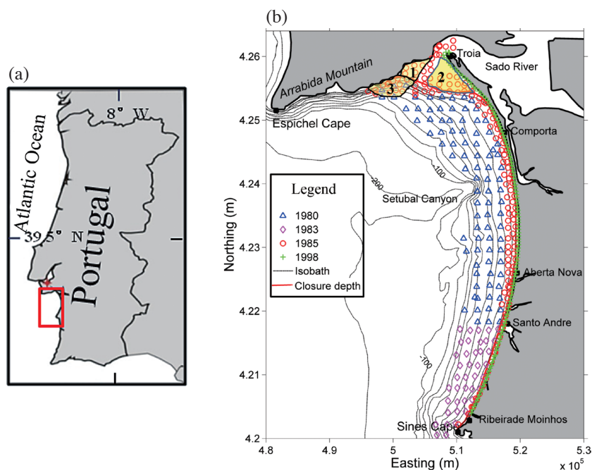
Fig. 1. Map showing the study area location in Portugal (a); Bathymetric map showing sampling locations in different years (b). Regions 1 and 2 are on the ebb-tidal delta and region 3 is located at the delta front near to the northern extremity of the system. The contour intervals of the isobaths on the inner shelf are in 10 m and the red line shows the location of closure depth.
