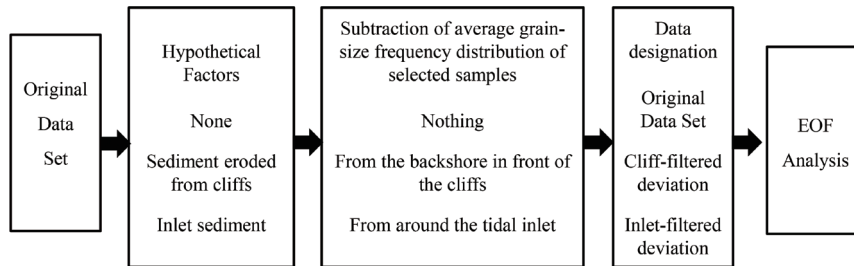
Fig. 2. Flow chart for the grain-size analysis that applies the filtering concept in the EOF technique.
