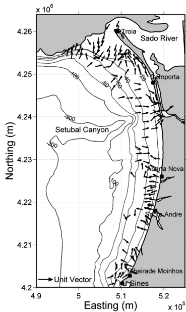
Fig. 9. Sediment transport vectors in the study area deduced from the Gao-Collins model.
