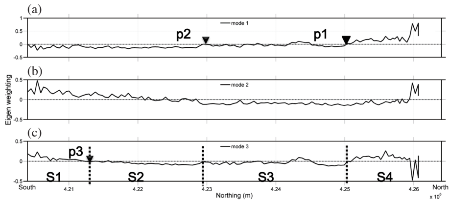
Fig. 5. Berm sample EOF analysis results and Eigen weightings in mode 1 (a), in mode 2 (b), and in mode 3 (c). The shoreline is divided into 4 segments according to the zero-crossing locations p1 - p3 (see details in text).
