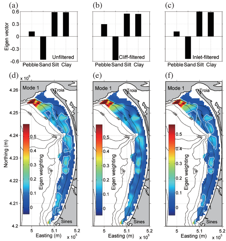
Fig. 11. EOF analysis results of different grain-size data sets (based on the flow chart shown in Fig. 2) for Eigen-mode 1. Eigen vectors (top) and Eigen weightings (bottom) of (a), (d) unfiltered data set; (b), (e) cliff-filtered; and (c), (f) inlet-filtered deviations, respectively.
