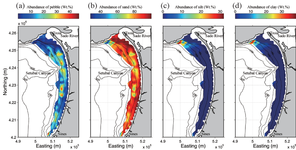
Fig. 6. Distribution pattern plots over the bathymetric contours of pebble (a), sand (b), silt (c), and clay (d), respectively. The abundance (weight %) of each size class is indicated by the color bar on the top.
