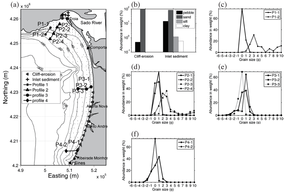
Fig. 8. The locations where sediment is chosen to represent cliff erosion (solid triangle) and inlet sediment (cross) and the sites to present the grain size spectrum (a); characteristic grain-size composition of the two important sediment sources (b); grain-size distribution curves of four profilers (c) - (f).
