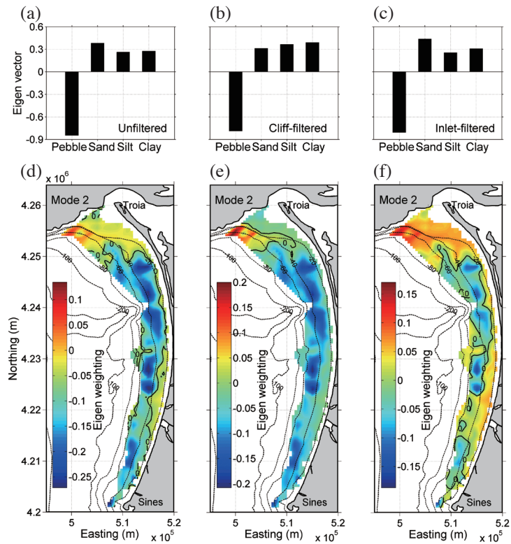
Fig. 12. EOF analysis results for different grain-size data sets (based on the flow chart shown in Fig. 2) for Eigen-mode 2. Eigen vectors (top) and Eigen weightings (bottom) of (a), (d) unfiltered data set; (b), (e) cliff-filtered; and (c), (f) inlet-filtered, respectively.
