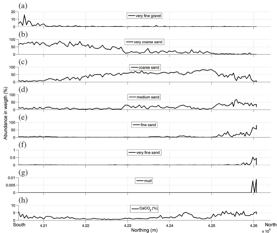
Fig. 3. Abundance (weight %) of very fine gravel (a), very coarse sand (b), coarse sand (c), medium sand (d), fine sand (e), very fine sand (f), mud (g), and CaCO 3 (h) on the berm along the shoreline. The southern end is on the left, the northern end is on the right.
