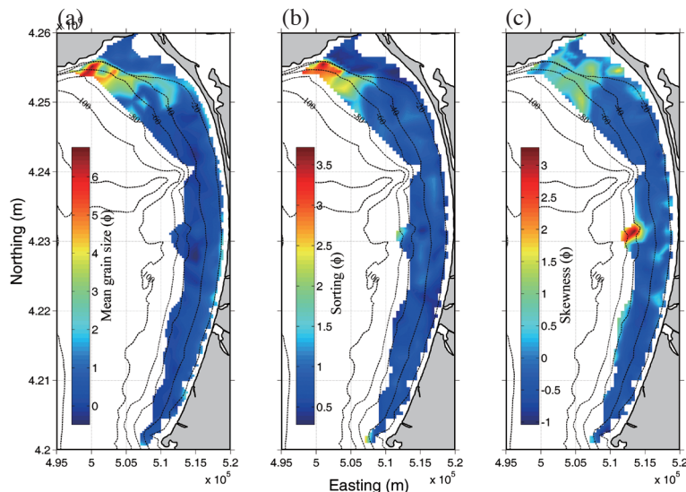
Fig. 7. The mean grain-size spatial distribution (a), sorting (b), and skewness (c).
