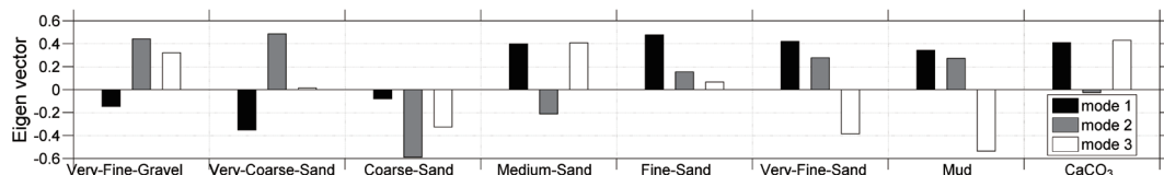
Fig. 4. Berm sample EOF analysis results and Eigen vectors for the first three modes.
