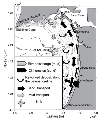
Fig. 13. Embayed system conceptual model for the sources, sinks and sediment transport patterns.
