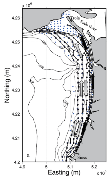
Fig. 10. Sediment transport pathways in the nearshore area (black arrows) and offshore zones (gray arrows) deduced from the McLaren model.
