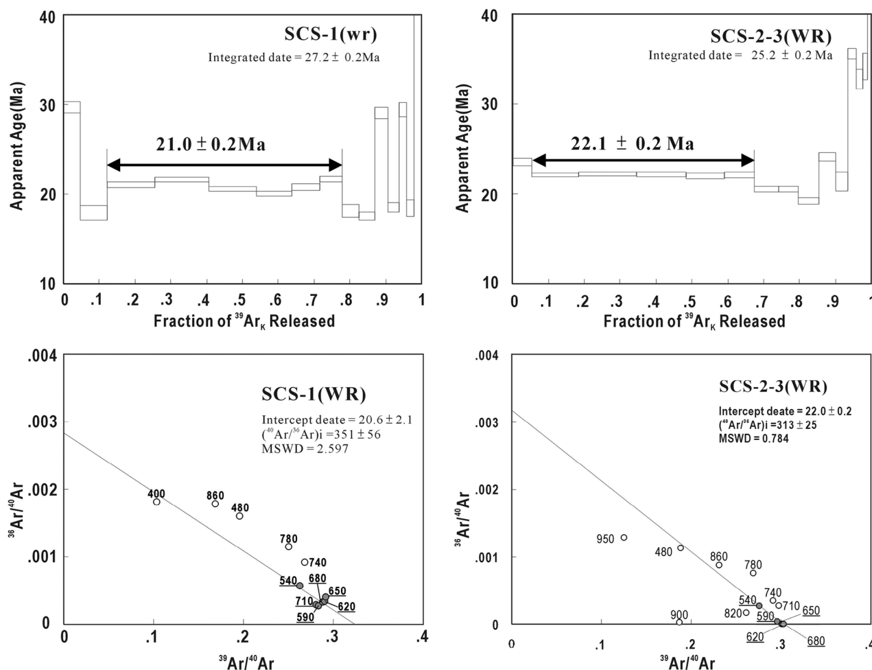
Fig. 2. Whole-rock ^{40}\text{Ar}/^{39}\text{Ar} age spectrum and isotope correlation diagram for dredged basalts SCS-1 and SCS-2-3.
