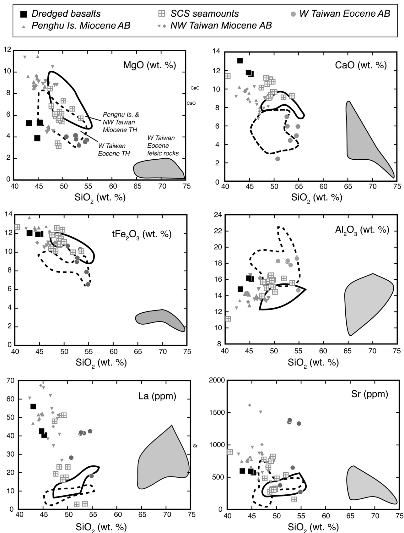
Fig. 4. Variation diagrams of MgO, Fe 2 O 3 , CaO, Al 2 O 3 , Sr and La versus SiO 2 , respectively, for dredged basalts at offshore SW Taiwan. Data sources and symbols are the same as Fig. 3.
