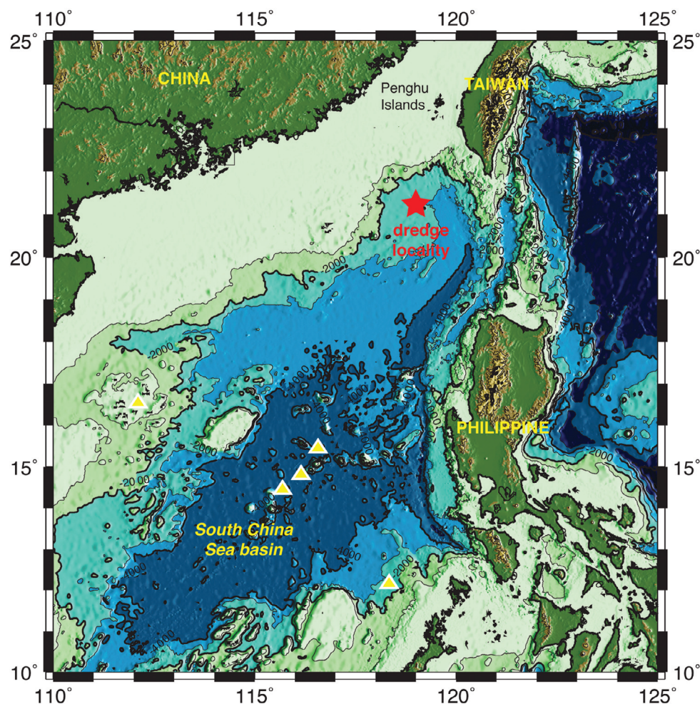
Fig. 1. Bathymetric map (created from the TECDC graphic service at IESAS, Taipei) showing locality of dredged basalts in this study (marked as a red star). Yellow triangles mark localities of the SCS seamounts used to compare their geochemical features with dredged basalts in this study (see the text for details).
