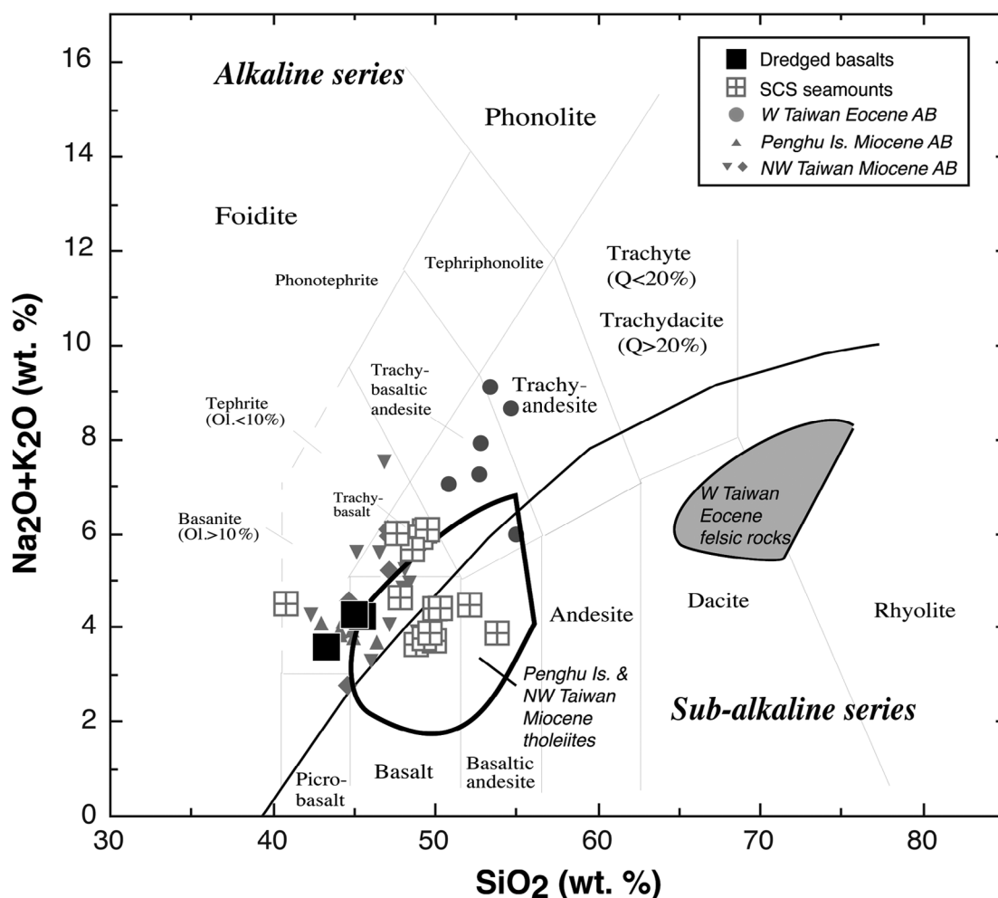
Fig. 3. Diagram of total alkali ( \text{K}_2\text{O} + \text{Na}_2\text{O} ) versus \text{SiO}_2 for dredged basalts at offshore SW Taiwan. SCS seamounts (Tu et al. 1992), the Eocene volcanic rocks drilled in the Taiwan Strait and onland Taiwan taken from Wang et al. (2012) and Miocene intraplate basalts in the Penghu Islands from Chung et al. (1994, 1995) are also shown for comparison. Rock type boundaries are from Le Maitre et al. (1989).
