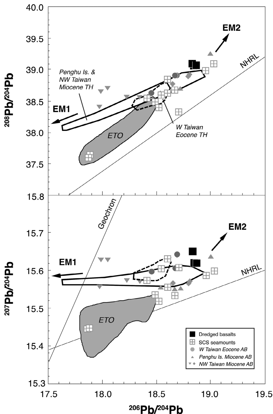
Fig. 7. ^{208}\text{Pb}/^{204}\text{Pb} and ^{207}\text{Pb}/^{204}\text{Pb} versus ^{206}\text{Pb}/^{204}\text{Pb} diagrams for dredged basalts at offshore SW Taiwan. Data for the ETO are from Sun (1980). The enriched mantle components EM1 and EM2 are from Hart (1988). The NHRL is from Hart (1984). Other data sources are the same as in Fig. 6.
