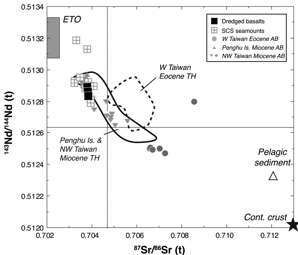
Fig. 6. Variation of ^{87}\text{Sr}/^{86}\text{Sr} (t) versus ^{143}\text{Nd}/^{144}\text{Nd} (t) for dredged basalts at offshore SW Taiwan. Data sources and symbols are the same as Fig. 3. Field of the East Taiwan Ophiolite (ETO) is from Jahn (1986) and Chung and Sun (1992). The composition of average continental crust from Taiwan is from Lan et al. (1990).
