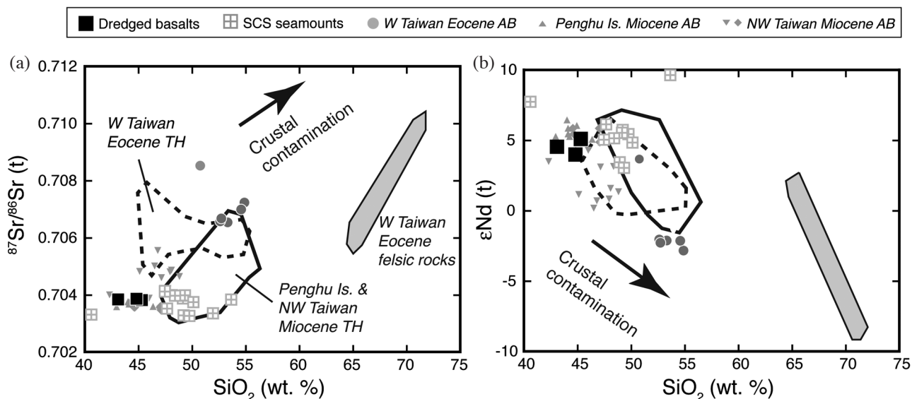
Fig. 8. Diagrams of (a) ^{87}\text{Sr}/^{86}\text{Sr} and (b) \epsilon\text{Nd}_{(t)} versus \text{SiO}_2 (wt. %) for dredged basalts at offshore SW Taiwan to show effect of crustal contamination on these rocks. Data sources and symbols are the same as Fig. 3.
