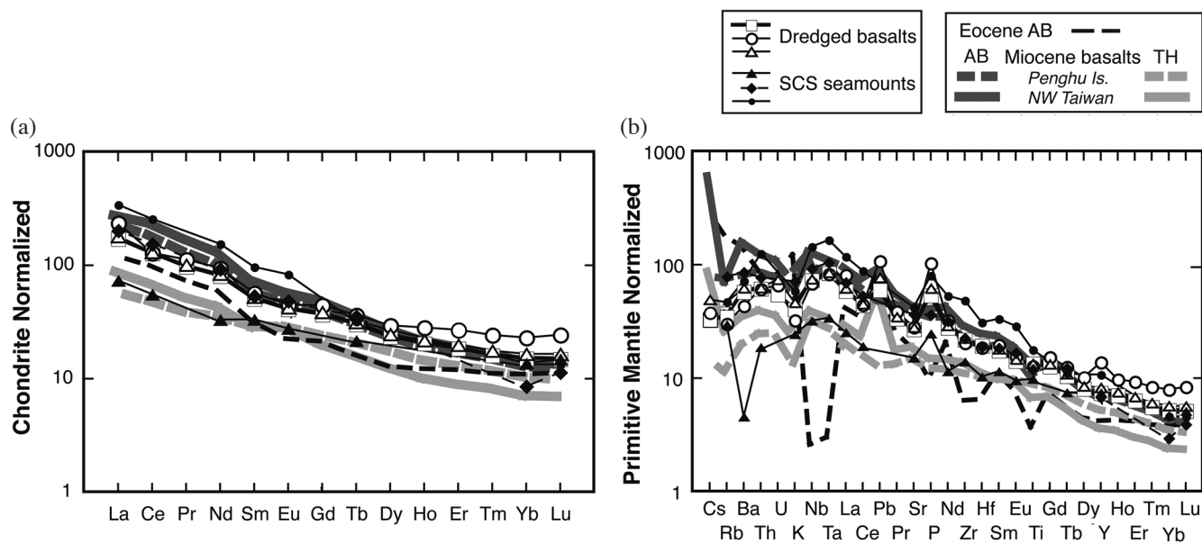
Fig. 5. A Chondrite-normalized REE variation diagram (a) and a primitive mantle-normalized trace element variation diagram (b) for dredged basalts at offshore SW Taiwan. Normalization constants are from Sun and McDonough (1989). Representative SCS seamounts (Tu et al. 1992), the Eocene volcanic rocks drilled in the Taiwan Strait and onland Taiwan from Wang et al. (submitted) and Miocene intraplate basalts in the Penghu Islands from Chung et al. (1994, 1995) are also shown for comparison. The letters in the legend representing the lithology, TH: tholeiite; AB: alkali basalt.
