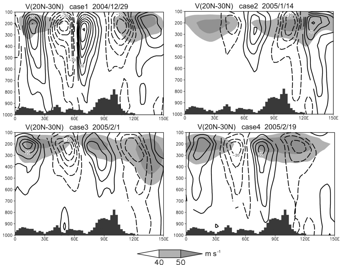
Fig. 3. Same as in Fig. 2, but for the longitude-height cross section of anomalous meridional wind (averaged over 20^{\circ} – 30^{\circ} N). Dark bar and gray shading denote topography and total zonal wind, respectively. Contour represents meridional wind anomaly with 5 \text{ m s}^{-1} interval.
