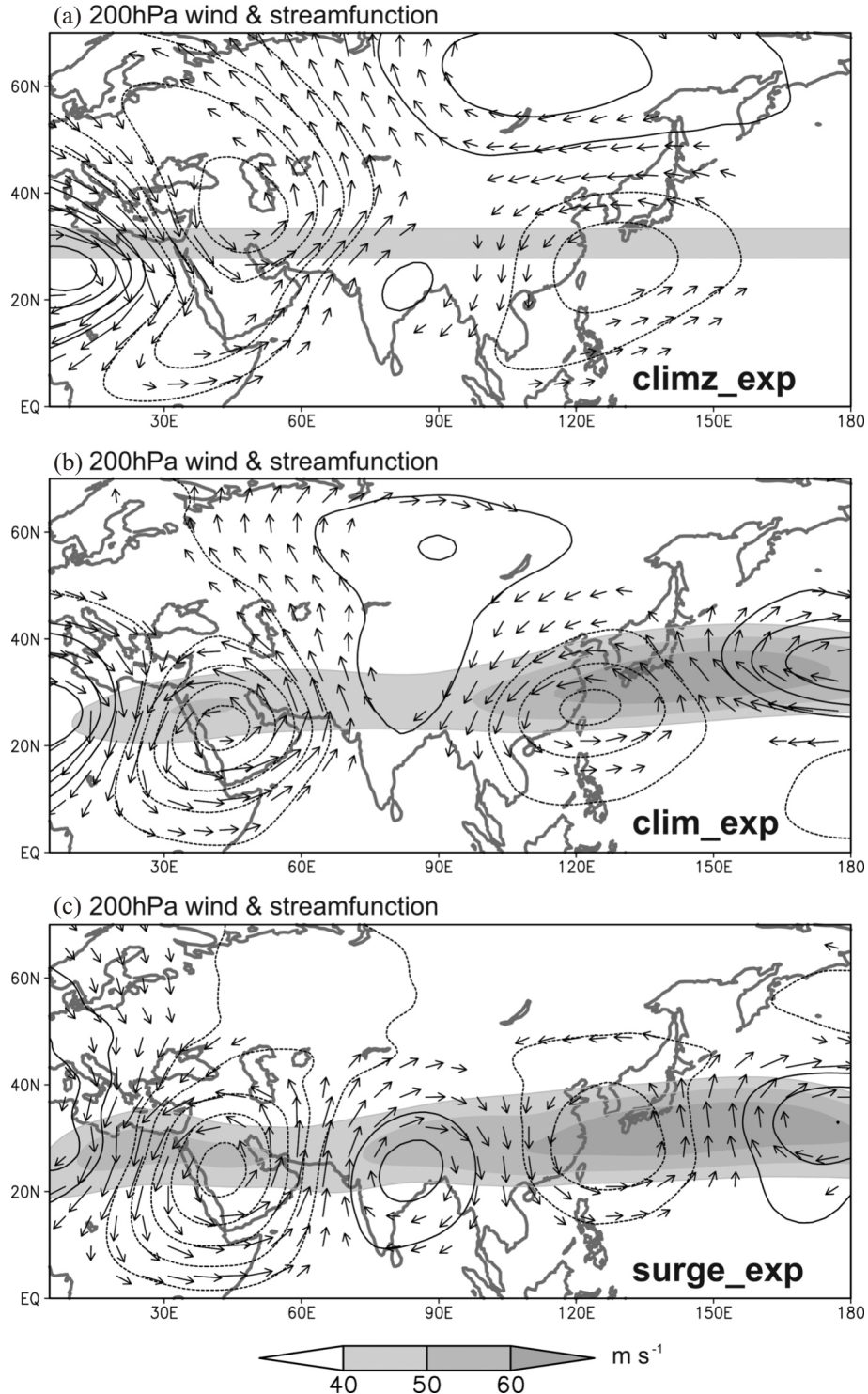
Fig. 9. Steady response (representing 200-hPa streamfunction anomaly) to the RWS as shown in Fig. 8b. (a) - (c) are simulated results of climz_exp , clim_exp , and surge_exp . Contour interval is 100 \text{ m}^2 \text{ s}^{-2} , and shading denotes 200-hPa zonal wind larger than 40 \text{ m s}^{-1} .
