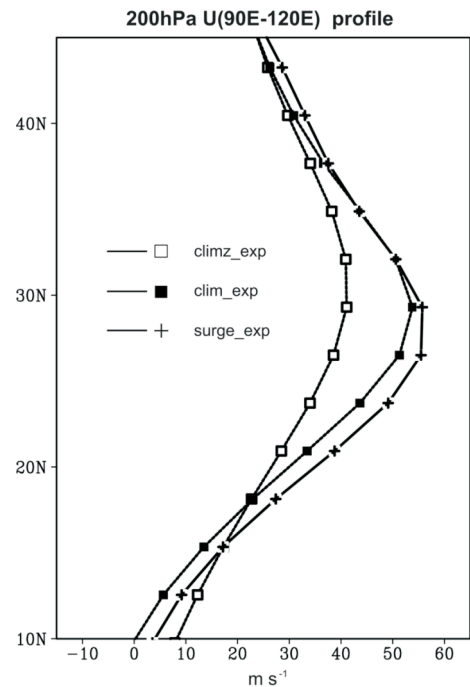
Fig. 7. Meridional profile of the 200-hPa zonal wind averaged over 90^\circ\text{E} - 120^\circ\text{E} for the three basic flows: climatological zonal mean flow ( climz_exp ), climatological time mean flow ( clim_exp ), and mean flow in January - February 2005 ( surge_exp ).
