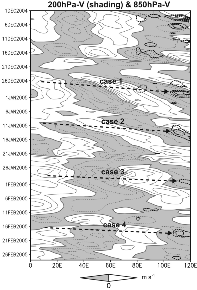
Fig. 4. Hovmöller diagrams of the 200-hPa (shading) and 850-hPa (contour) meridional wind anomaly averaged over 20°–30°N. Only the 850 hPa northerly anomaly in East Asia (80°–120°E) less than -3 \text{ m s}^{-1} is plotted. Contour interval is 3 \text{ m s}^{-1} . Dashed arrows denote the wave trains linked with cold surges.
