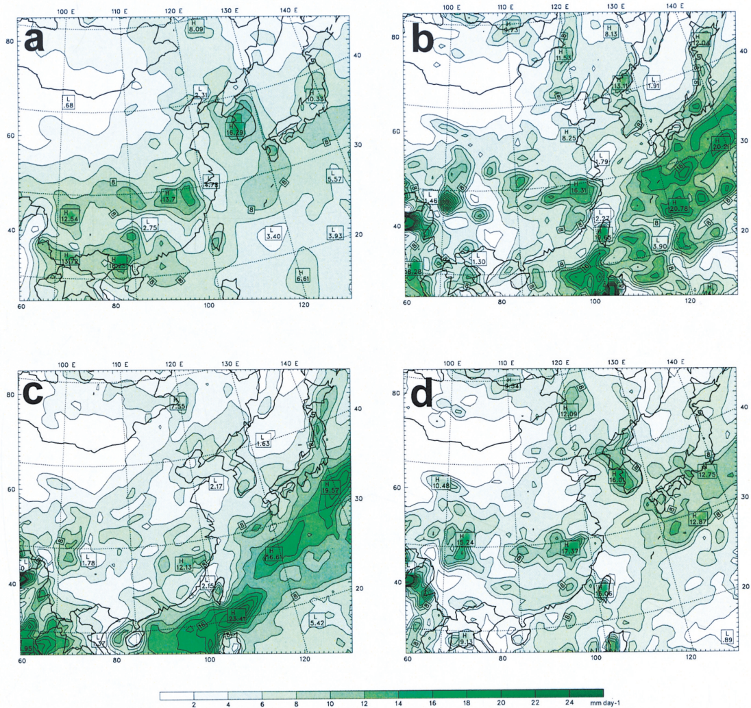
Fig. 2. Seasonal mean precipitation over East Asia during the summer of 1998 (JJA) in (a) observation, (b) GR60, (c) KF60, and (d) AK60. The contour intervals are 2 \text{ mm day}^{-1} .
