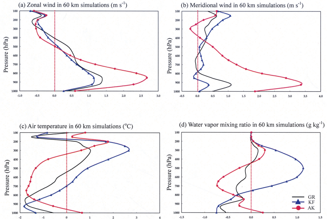
Fig. 8. Vertical profiles of seasonal mean bias (model - reanalysis) in (a) zonal wind and (b) meridional wind, (c) air temperature, and (d) water vapor mixing ratio during the summer of 1998 (JJA) averaged over the land in the nested domain.
