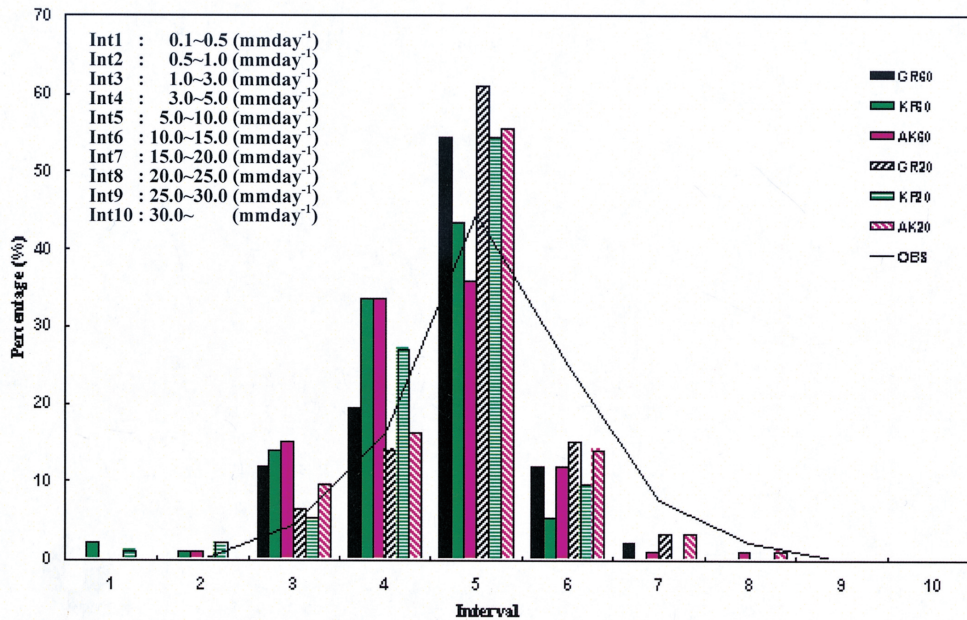
Fig. 7. Daily precipitation intensity averaged over the land in the nested domain during the summer of 1998 (JJA) in observation and simulations. The frequency of intensity within a given interval is represented as the percentage of the total number of rain events.
