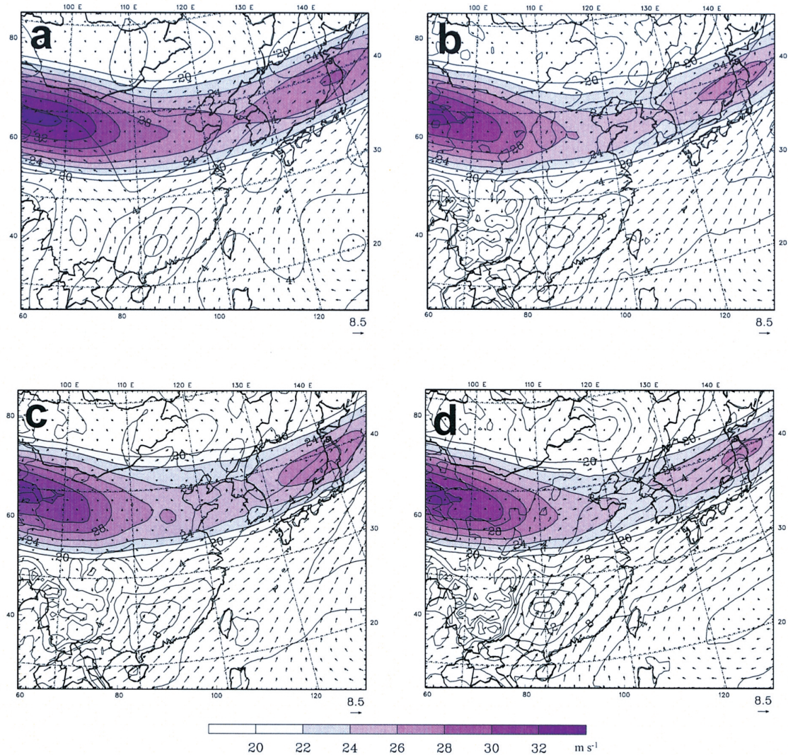
Fig. 3. Seasonal mean 850 hPa wind vector and speed with 200 hPa wind speed (shaded) superposed over East Asia during the summer of 1998 (JJA) in (a) NCEP reanalysis, (b) GR60, (c) KF60, and (d) AK60. The contour intervals are 2 \text{ m sec}^{-1} .
