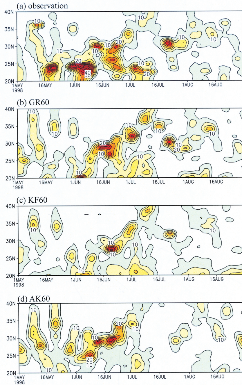
Fig. 5. Time-latitude distribution of daily precipitation (mmday -1 ) averaged between 110° and 120°E from 1 May to 31 Aug. in 1998 in (a) observation, (b) GR60, (c) KF60, and (d) AK60. The contour intervals are 5 mm day -1 .
