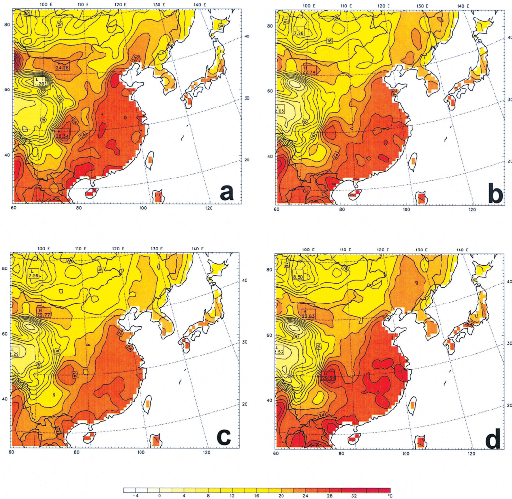
Fig. 4. Seasonal mean surface air temperature over East Asia during the summer of 1998 (JJA) in (a) observation, (b) GR60, (c) KF60, and (d) AK60. The contour intervals are 2°C.
