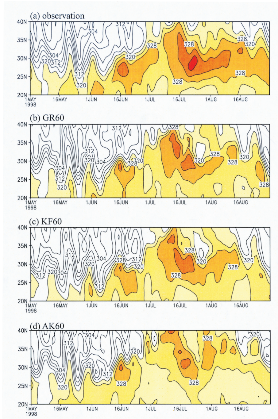
Fig. 6. The same as in Fig. 4 but for 850 hPa equivalent temperature with contour intervals of 4 K.
