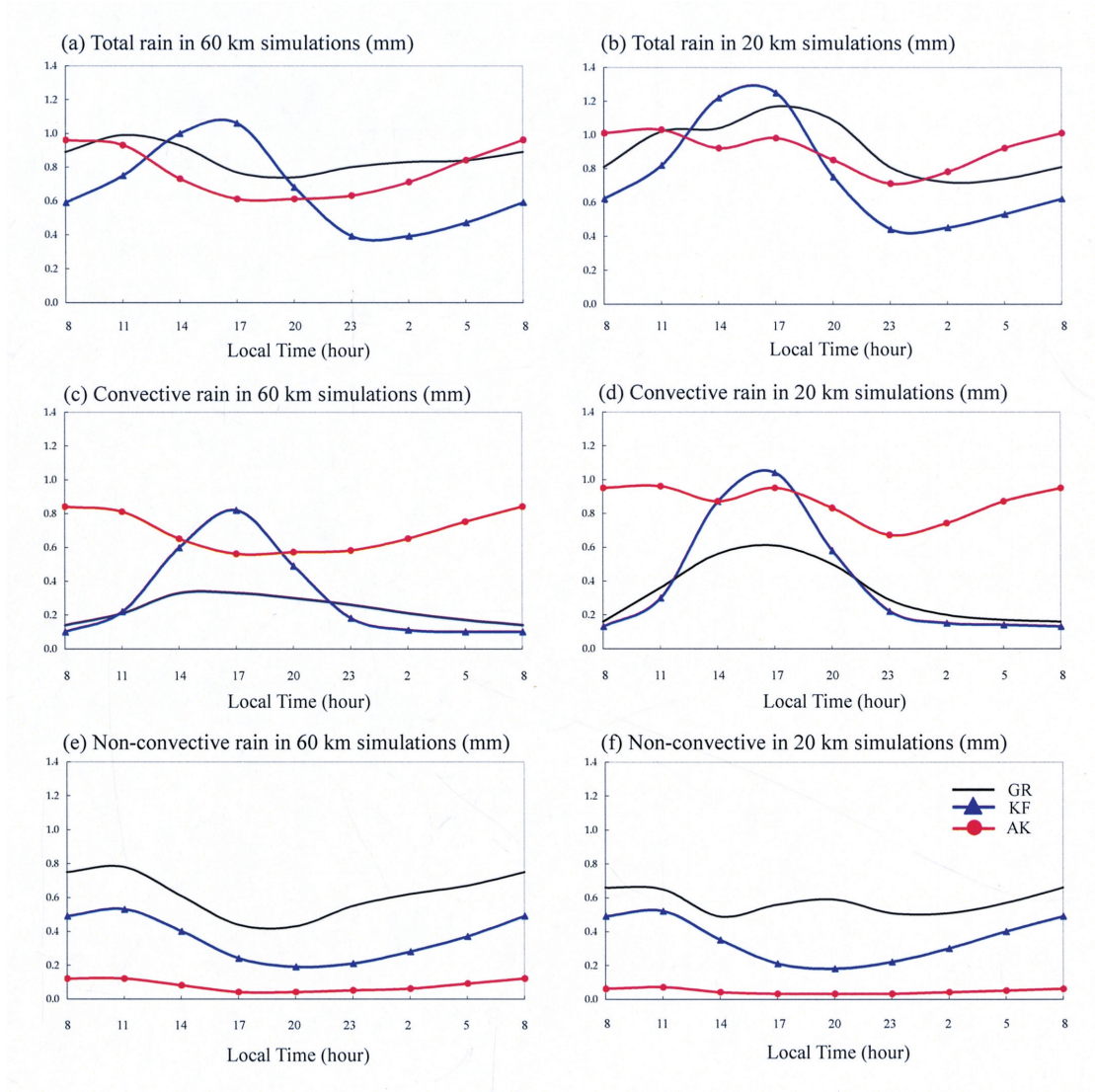
Fig. 10. Diurnal variations of simulated 3-hour (a, b) total rain (mm), (c, d) convective rain and (e, f) non-convective rain (mm) averaged over land in the nested domain.
