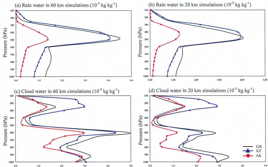
Fig. 9. Vertical profiles of seasonal mean (a, b) rain water, and (c, d) cloud water during the summer of 1998 (JJA) averaged over land in the nested domain.
