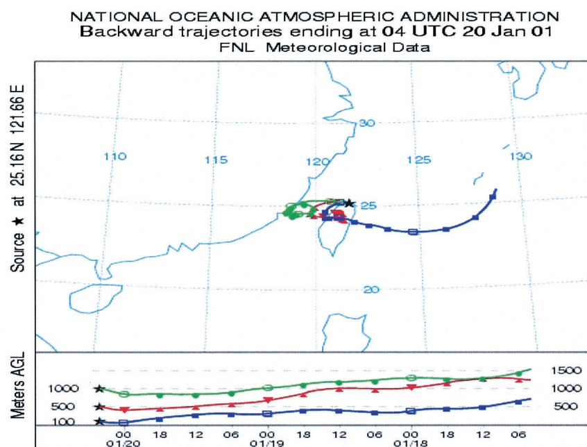
Fig. 5. Result of the HYSPLIT model 3-day backward trajectory analysis started at 0400UTC (1200LST) Jan. 20, 2001 at altitudes of 100, 500 and 1000 m at Wan-Li station in northern Taiwan. The top and bottom panels display horizontal and vertical motion. Symbols denote the location of the air parcel every 6 hours.
