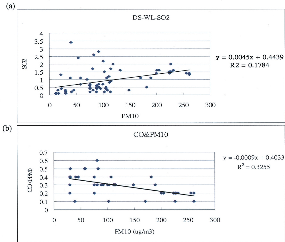
Fig. 8. Relationship between (a) PM 10 and SO 2 (b) PM 10 and CO during (0100LST April 12 to 2400LST April 13, 2001 at Wan-Li station).
