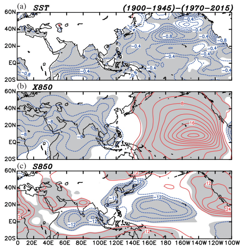
Fig. 4. As in Fig. 2, except for the differences of (a) SST, (b) 850-hPa velocity potential, and (c) 850-hPa streamfunction in July–September of 1900–1945 minus those of 1970–2015. Differences with significance at the 0.10 level of the Student's t test are shaded. Contour intervals are 0.1^{\circ}\text{C} in (a), 2 \times 10^5 \text{ m}^2 \text{ s}^{-1} in (b), and 4 \times 10^5 \text{ m}^2 \text{ s}^{-1} in (c). The zero contours are suppressed.
