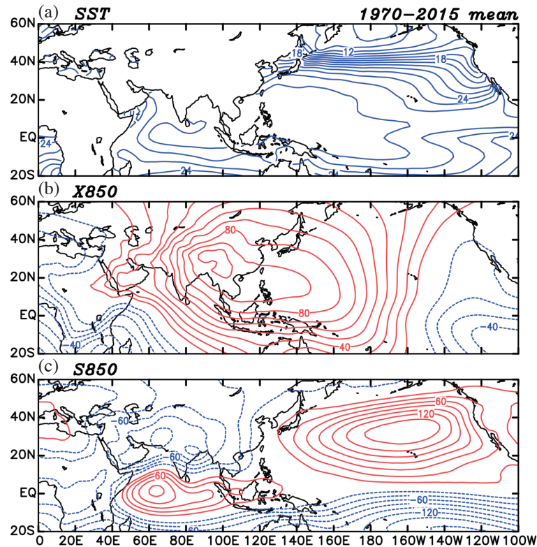
Fig. 3. As in Fig. 2, except for the climatological means of (a) SST, (b) 850-hPa velocity potential, and (c) 850-hPa streamfunction in July–September of 1970–2015.
