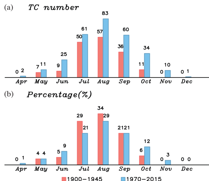
Fig. 1. The monthly average (a) number and (b) percentage (%) of typhoons affecting Taiwan from April to December during 1900–1945 (red color) and 1970–2015 (blue color).
