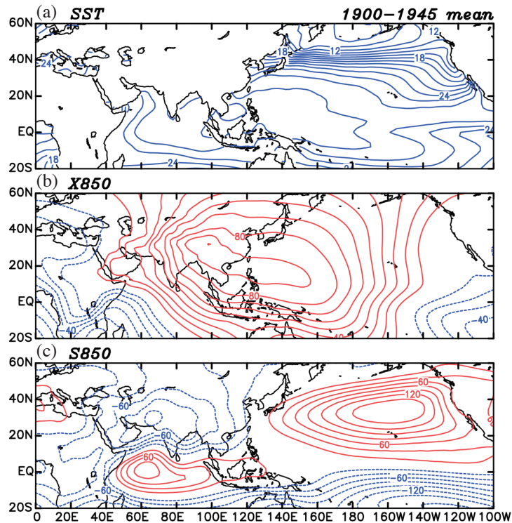
Fig. 2. The climatological means of (a) sea surface temperature (SST), (b) 850-hPa velocity potential (X850), and (c) 850-hPa streamfunction (S850) in July–September of 1900–1945. Contour intervals are 1.5^{\circ}\text{C} in (a), 10 \times 10^5 \text{ m}^2 \text{ s}^{-1} in (b), and 20 \times 10^5 \text{ m}^2 \text{ s}^{-1} in (c). The zero contours are suppressed.
