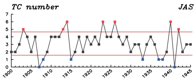
Fig. 5. The time series of the number of typhoons affecting Taiwan in July–September of 1900–1945. The long-term mean is 3.11 and standard deviation is 1.54. The one standard deviation above and below the average are indicated by red dashed lines, respectively.
