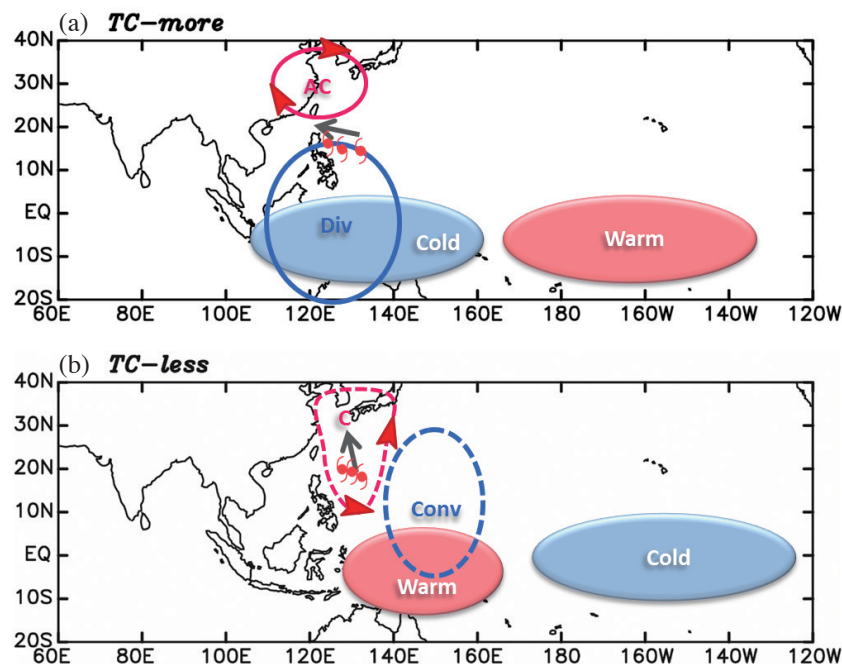
Fig. 13. Schematic diagrams for large-scale modulating processes in the (a) typhoon-more, and (b) typhoon-less years. Positive/negative SST anomalies are marked by “Warm”/“cold” and red/blue shaded areas. Anticyclonic/cyclonic anomalies are represented by “AC”/“C” and red thin solid/dashed lines. Divergence/convergence anomalies are marked by “Div”/“Conv” and blue thin solid/dashed lines. Anomalous steering flows are indicated by black solid arrows.
