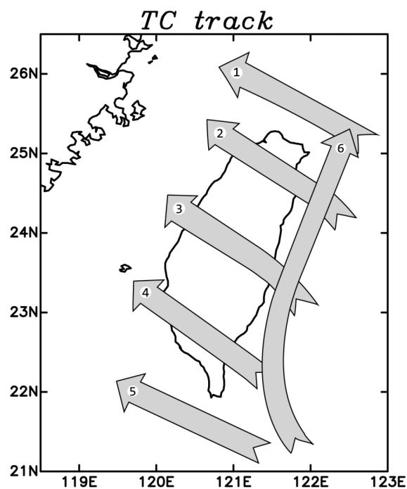
Fig. 10. Typhoon track numbers 1–6 denote the six major typhoon tracks affecting Taiwan.
