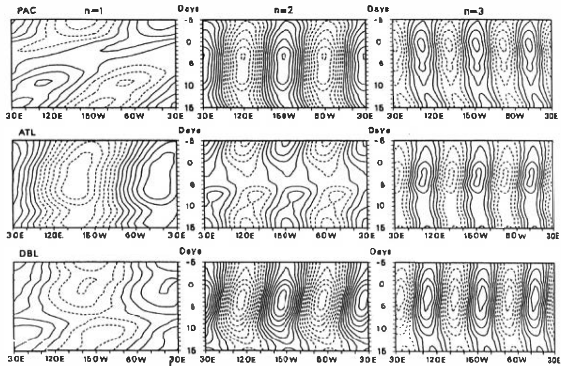
Fig. 8. The composite ridge-trough diagrams of 500 mb Z for n=1, 2 and 3 in the 54^{\circ} - 70^{\circ} N latitude belt. The contour interval is 40 m. The "0" in the ordinate denotes the onset day of blocking episodes.
