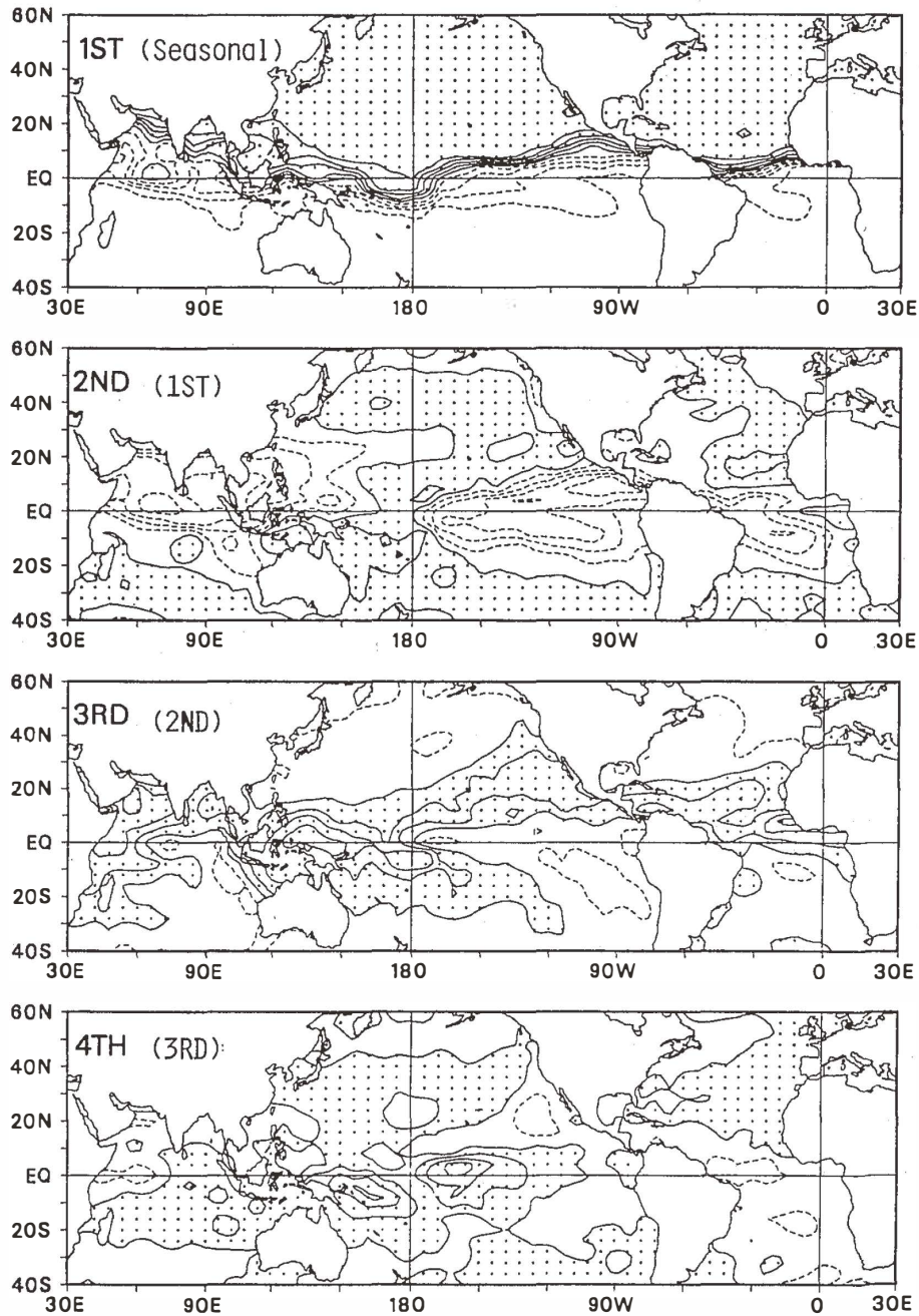
Fig. 7. Characteristic patterns for the first four principal components of monthly SSTs for the 30-month period from July 1991 to December 1993. The contour interval is 0.2. The identification of components in parentheses is the order after elimination of the 1st component which is the intraannual seasonal variation.
