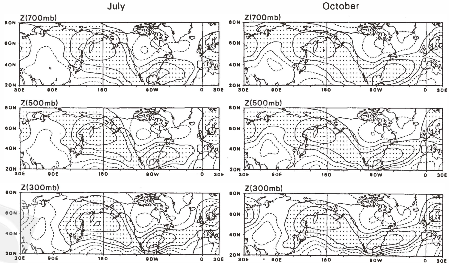
Fig. 3. Cross-correlation patterns of July and October ENIs with February Z fields at 700, 500 and 300 mb for 1958-92. Positive areas are shaded, and the contour interval is 0.2.
