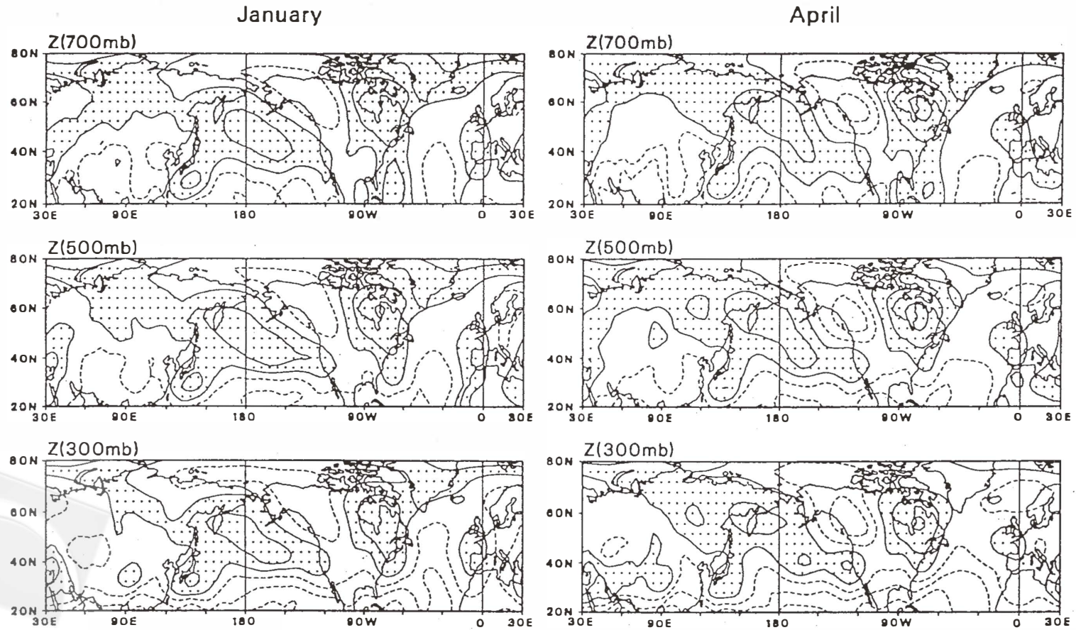
Fig. 6. Same as Figure 3, but for January and April ENIs with June Z fields.
