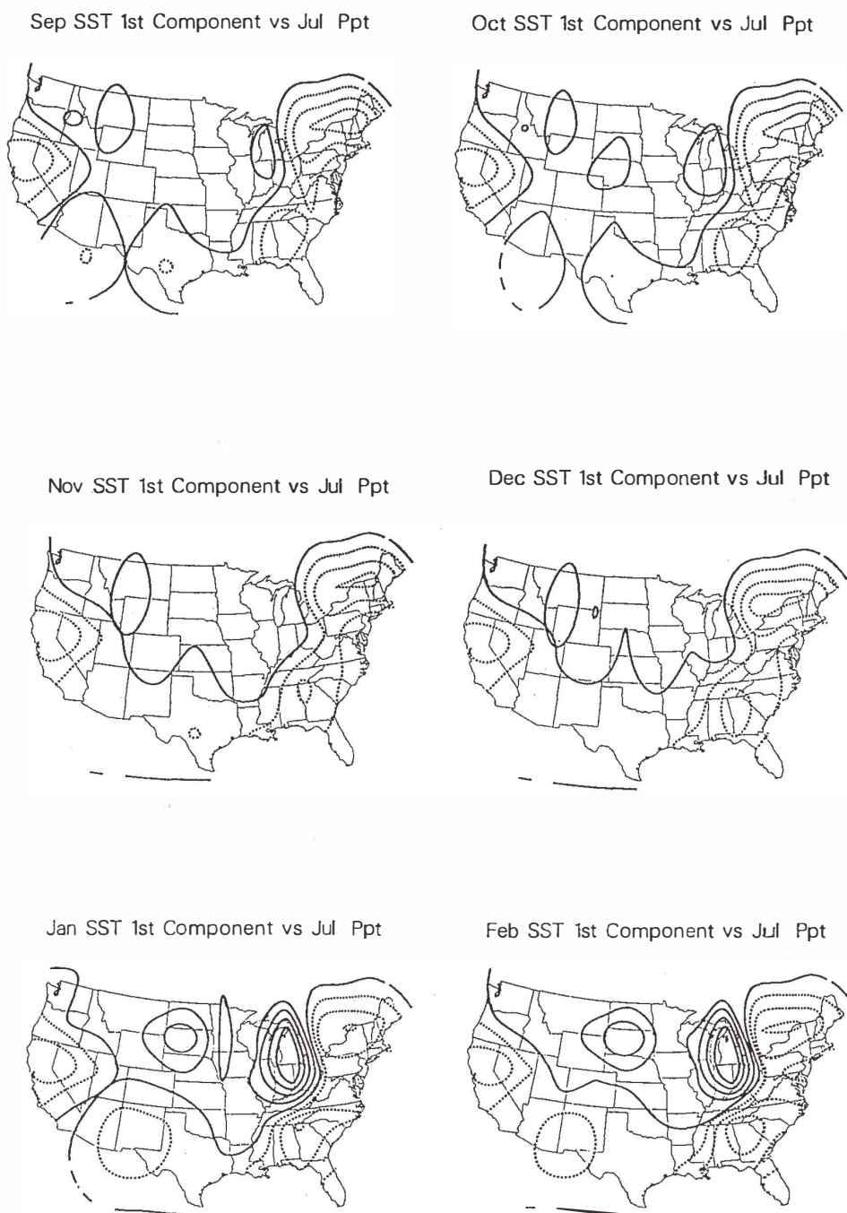
Fig. 13. Correlation pattern for the 1st principal component of SSTs and July U.S. precipitation during the period of 1961-1962. Contour interval is 0.1. The real line is for zero and positive, and the broken line for negative.
