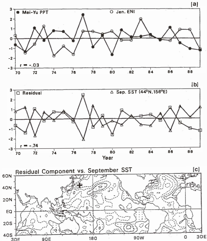
Fig. 10. Same as Figure 8, but for the Mei-Yu precipitation.
