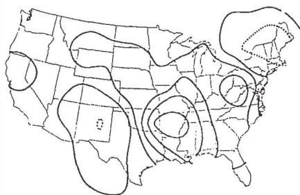
Fig. 11. Correlation patterns for the 1st principal component of SSTs with June U.S. temperatures during the period of 1961-1962. Contour interval is 0.1. The real line is for zero and positive, and the broken line for negative.
