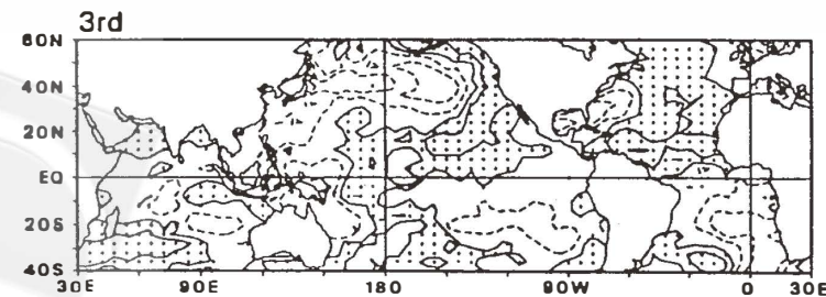
Fig. 1. Characteristic patterns (pattern vectors) for the first three principal components of January and July SSTs during the period of 1955-1992. Positive areas are shaded. The contour interval is 0.2. (After Kung and Chern, 1994)
