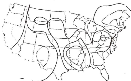
Fig. 11. Correlation patterns for the 1st principal component of SSTs with June U.S. temperatures during the period of 1961-1962. Contour interval is 0.1. The real line is for zero and positive, and the broken line for negative.
