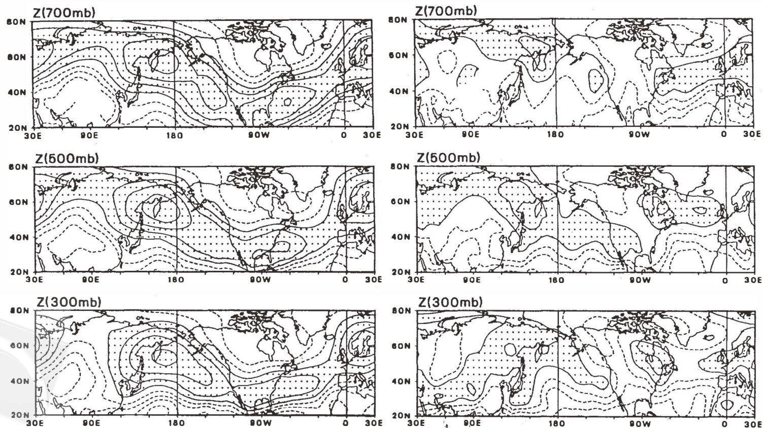
Fig. 4. Characteristic patterns of the first components of February and June Z fields at 700, 500 and 300 mb during 1955-1992. Positive areas are shaded and the contour interval is 0.2.
