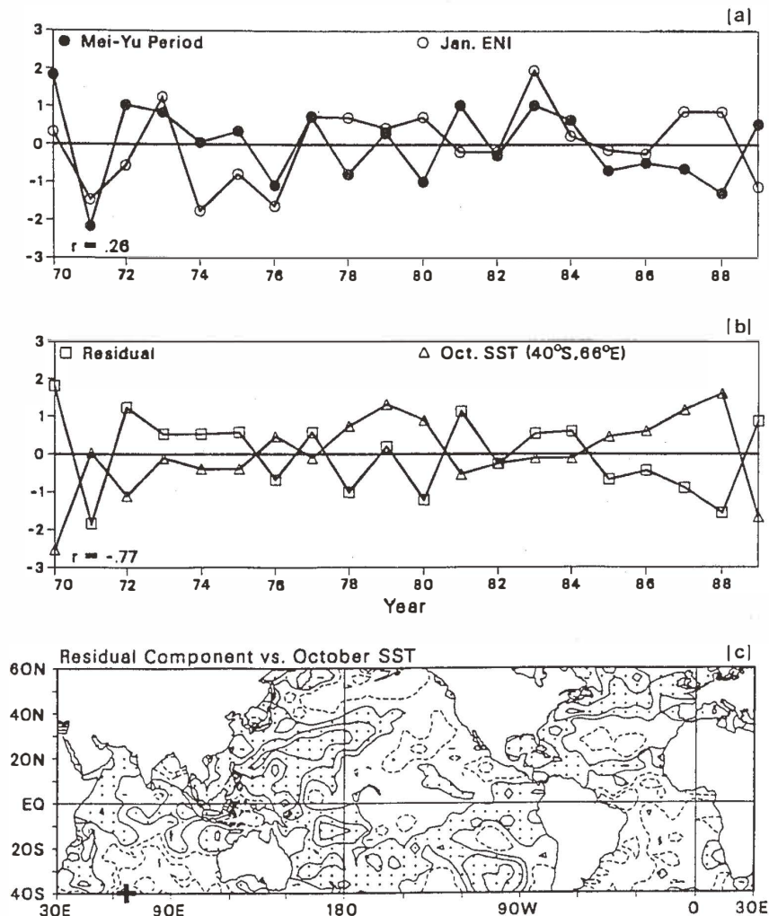
Fig. 9. Same as Figure 8, but for the Mei-Yu period.
