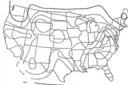
Fig. 12. Correlation patterns for the 2nd principal component of SSTs with June U.S. temperature during the period of 1961-1962. Contour interval is 0.1. The real line is for zero and positive, and the broken line for negative.
