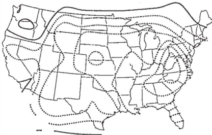
Fig. 12. Correlation patterns for the 2nd principal component of SSTs with June U.S. temperature during the period of 1961-1962. Contour interval is 0.1. The real line is for zero and positive, and the broken line for negative.
