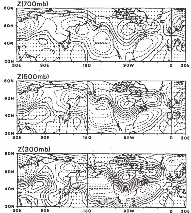
Fig. 5. Flow patterns and anomalies of February Z fields at 700, 500 and 300 mb for composites of prominent ENSO cases.
