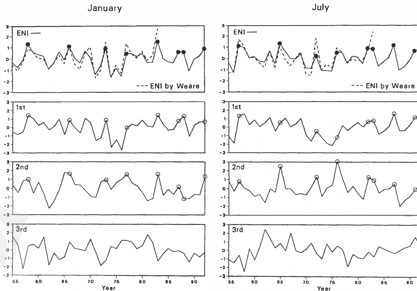
Fig. 2. Inter-annual variations of coefficients of the first three principal components of January and July SSTs during the period of 1955-1992. Dots denote years of major winter ENSO episodes. ENI is as defined in the text. ENI by Weare (1986) is represented by dashed lines. (After Kung and Chern, 1994)
