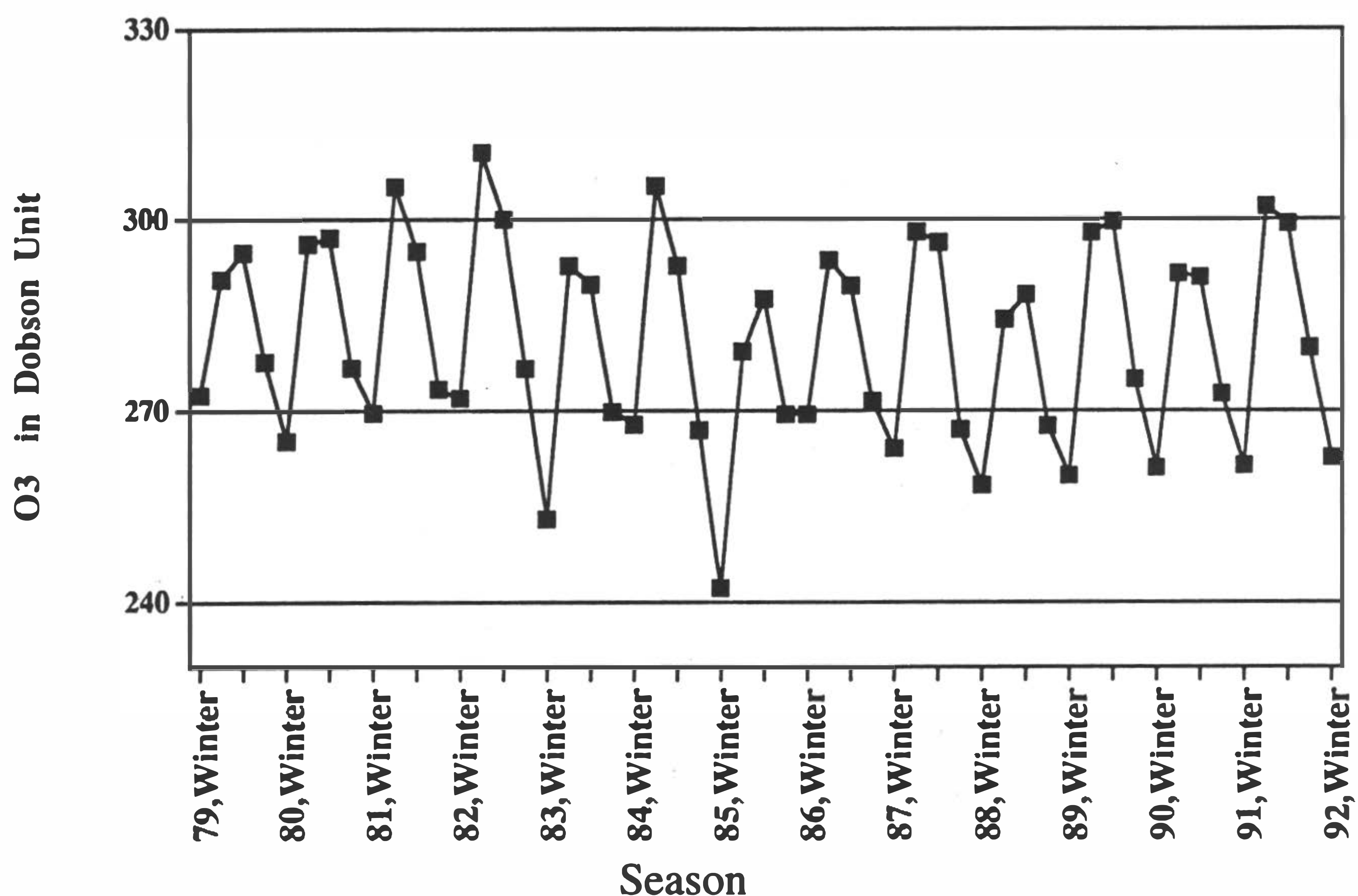
Fig. 5. Seasonal ozone variations over Taipei from 1979-1992.
