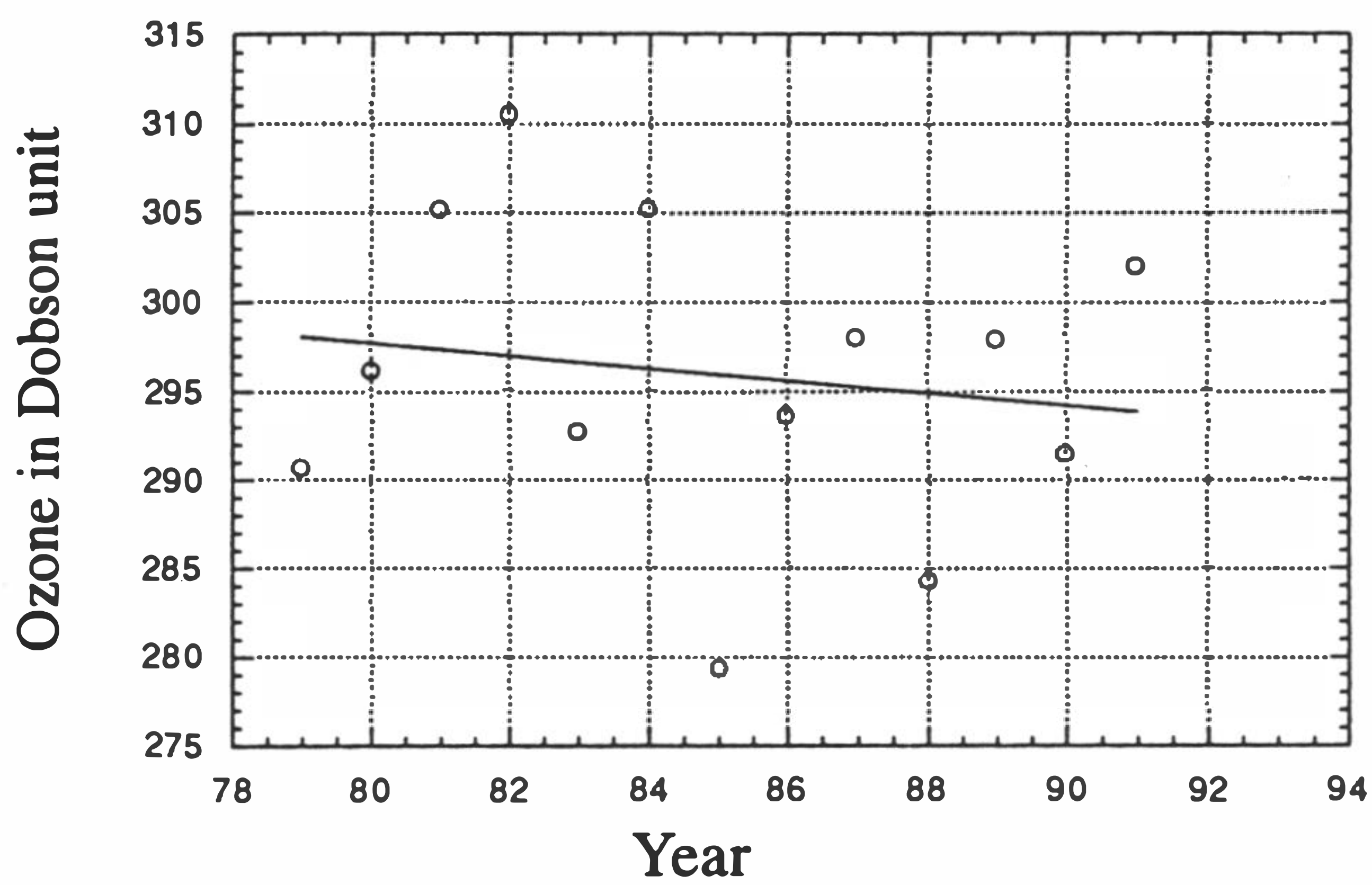
Fig. 7. Seasonal ozone variations for Spring.
