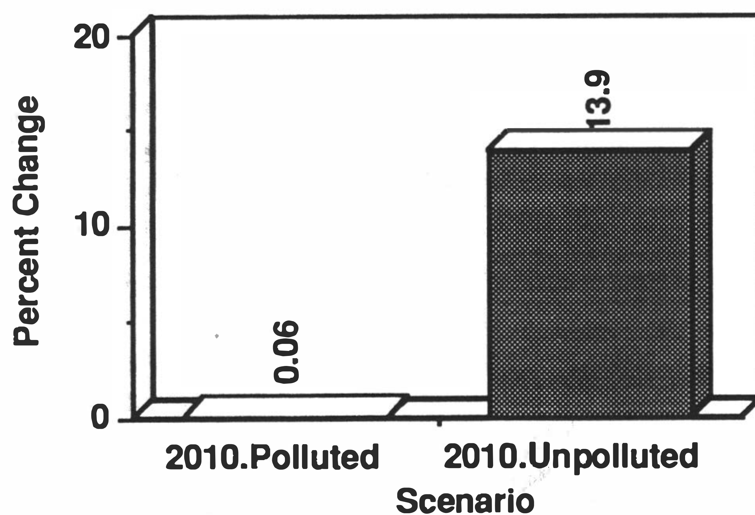
Fig. 12. predicted UV-B for scenarios of polluted and unpolluted Spring in year 2010.
