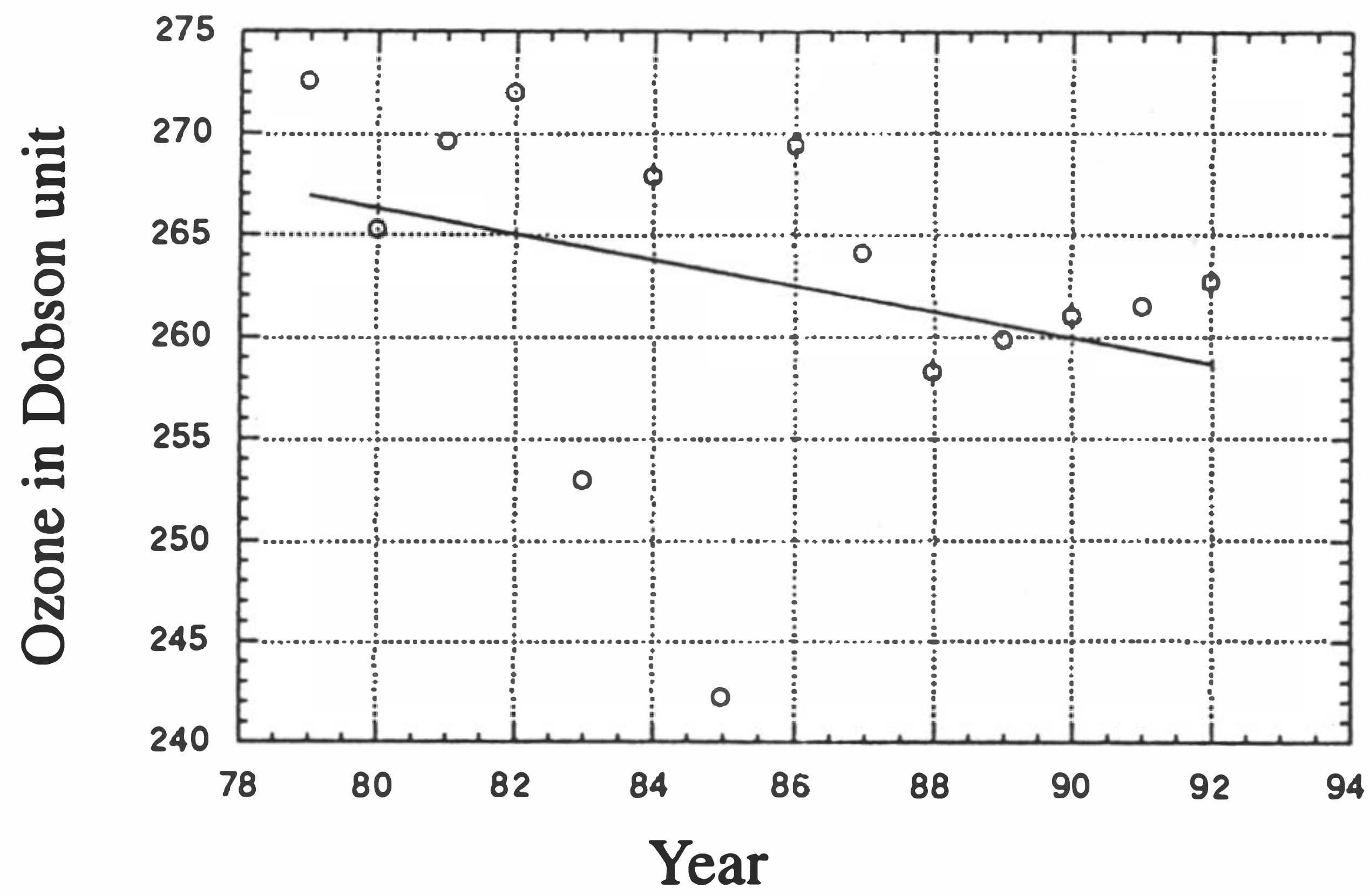
Fig. 6. Seasonal ozone variations for Winter.
