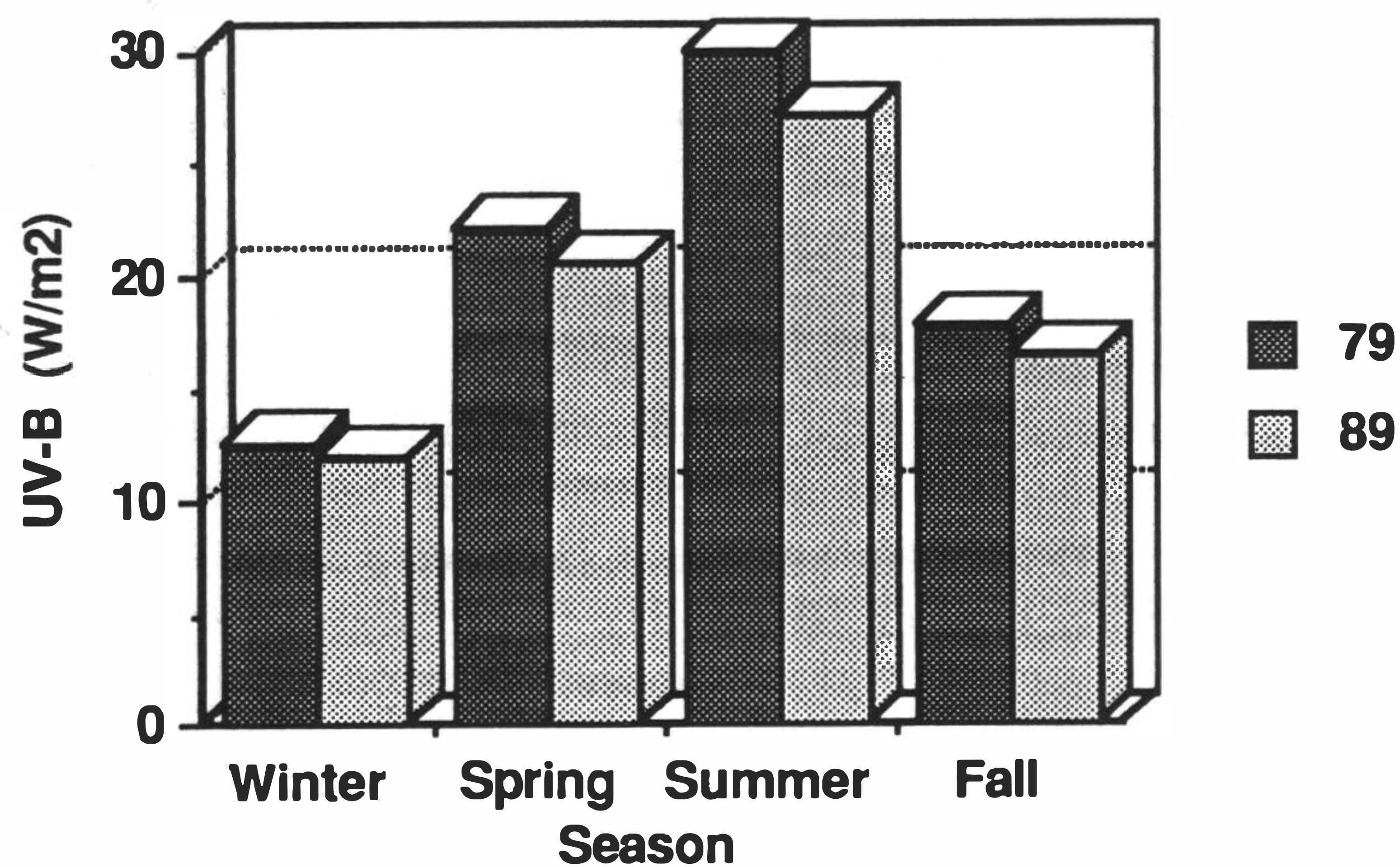
Fig. 10. Integrated UV-B estimated for Taipei.
