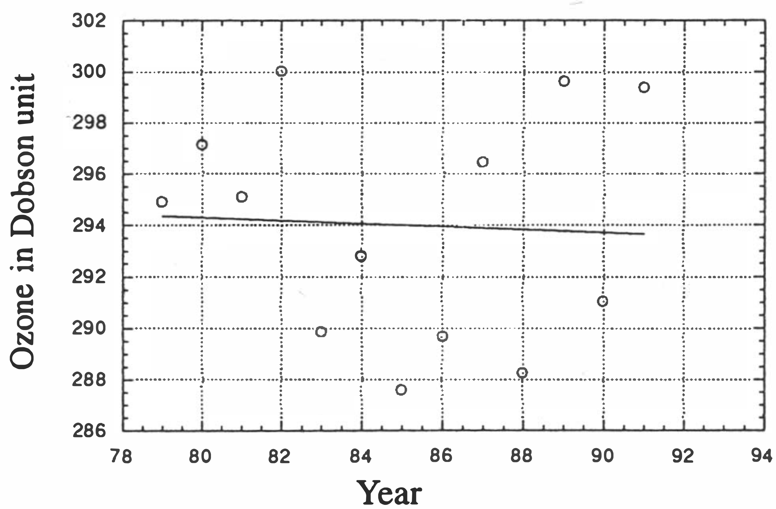
Fig. 8. Seasonal ozone variations for Summer.
