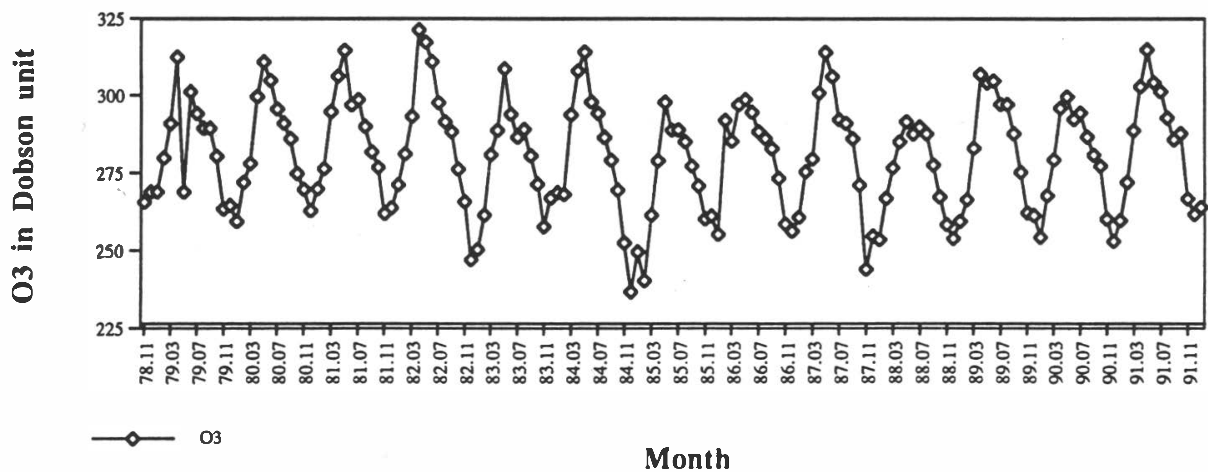
Fig. 4. Monthly ozone over Taipei from 1978-1992.
