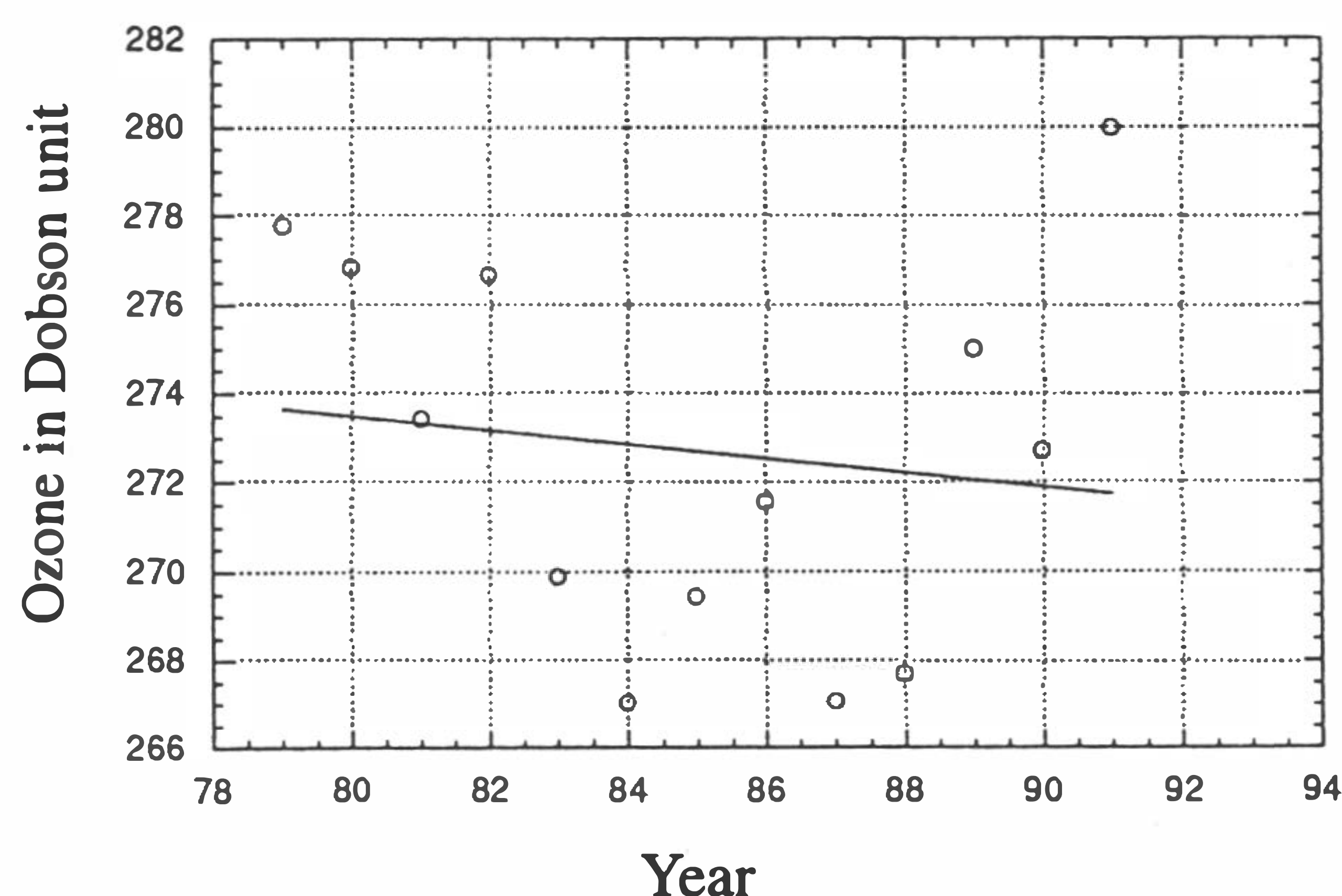
Fig. 9. Seasonal ozone variations for Fall.
