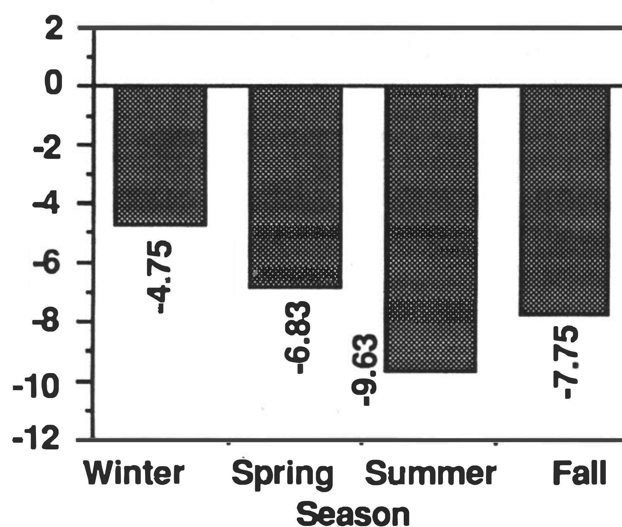
Fig. 11. Estimated percent change of UV-B over the past decade.
