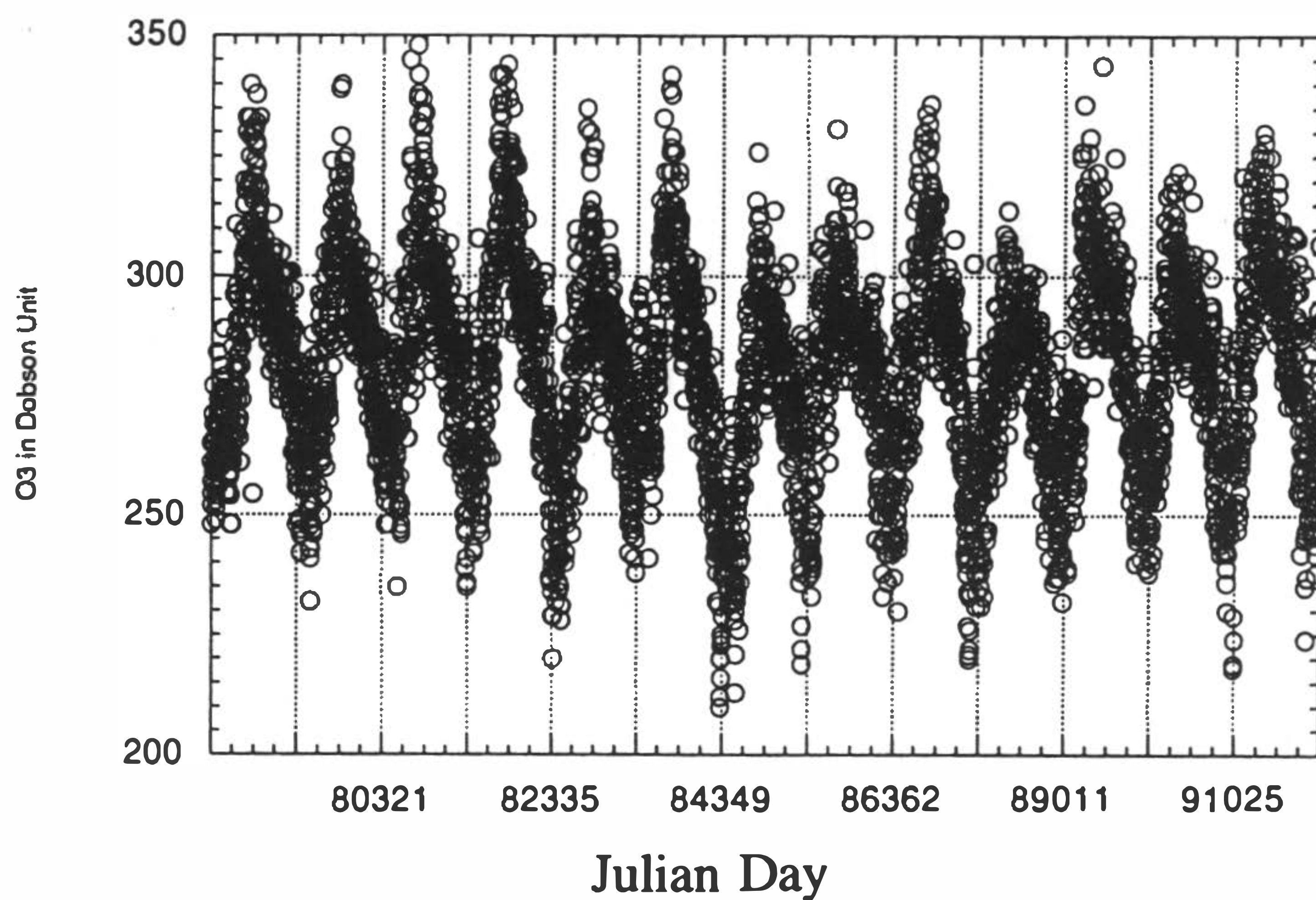
Fig. 3. Daily measurements of total ozone over Taipei, 1978-1992.
