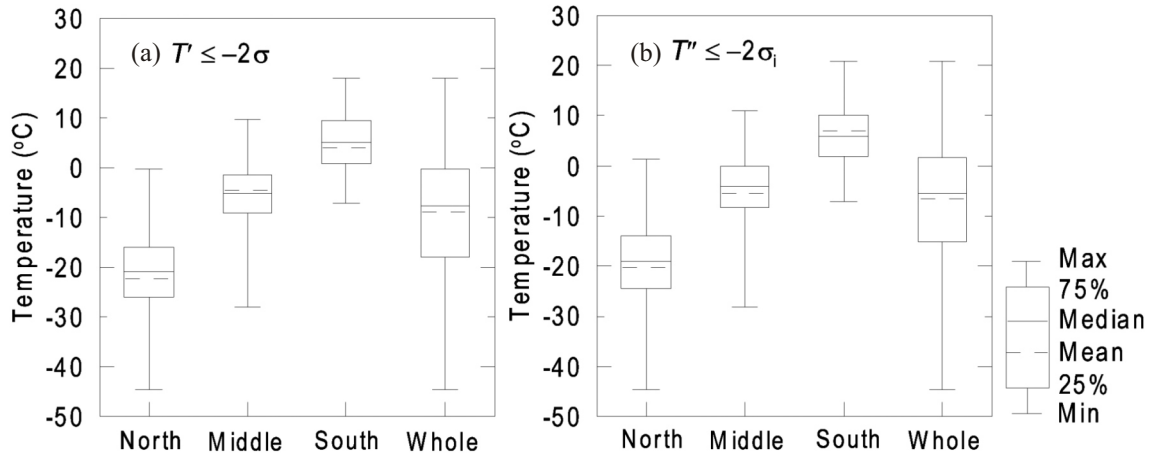
Fig. 2. Real temperature distribution of (a) T' \leq -2\sigma events and (b) T'' \leq -2\sigma_i events for northern region (north of 40°N), central region (40°N - 30°N), southern region (south of 30°N), and entire study area.
