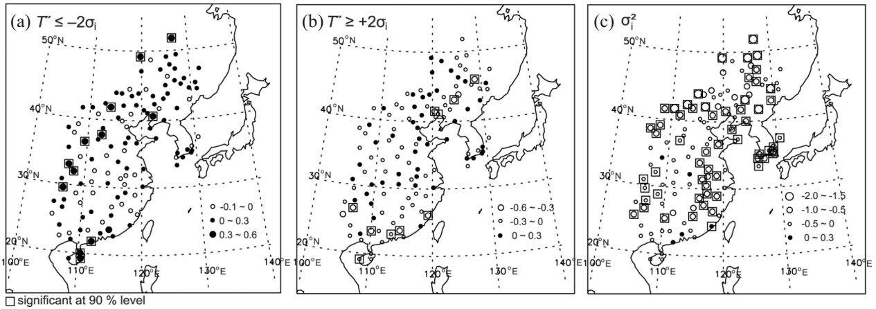
Fig. 3. Trends of (a) frequency of relatively cold events ( T' \leq -2\sigma_i ), (b) frequency of relatively warm events ( T'' \geq +2\sigma_i ), and (c) intraseasonal variance of daily temperature. Units for (a) and (b) are days per decade, and for (c), ^{\circ}\text{C}^2 per decade. Linear trends are estimated using the ordinary least squares method in filtered data for the period 1954 - 2006.
