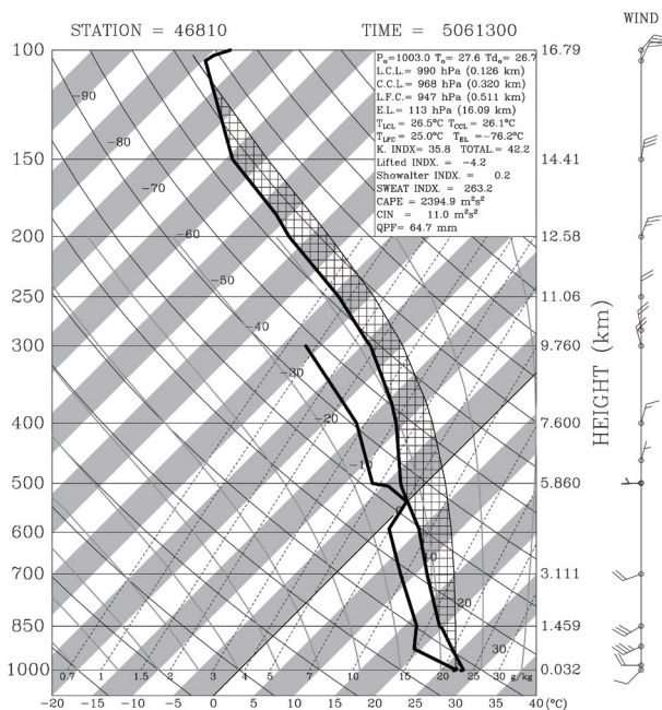
Fig. 4. Skew-T log P diagrams at Tongsha station at 0000 UTC 13 June 2005. Hatched regions indicate the area of positive energy. Some commonly used parameters associated with sounding are calculated and shown in upper right.
