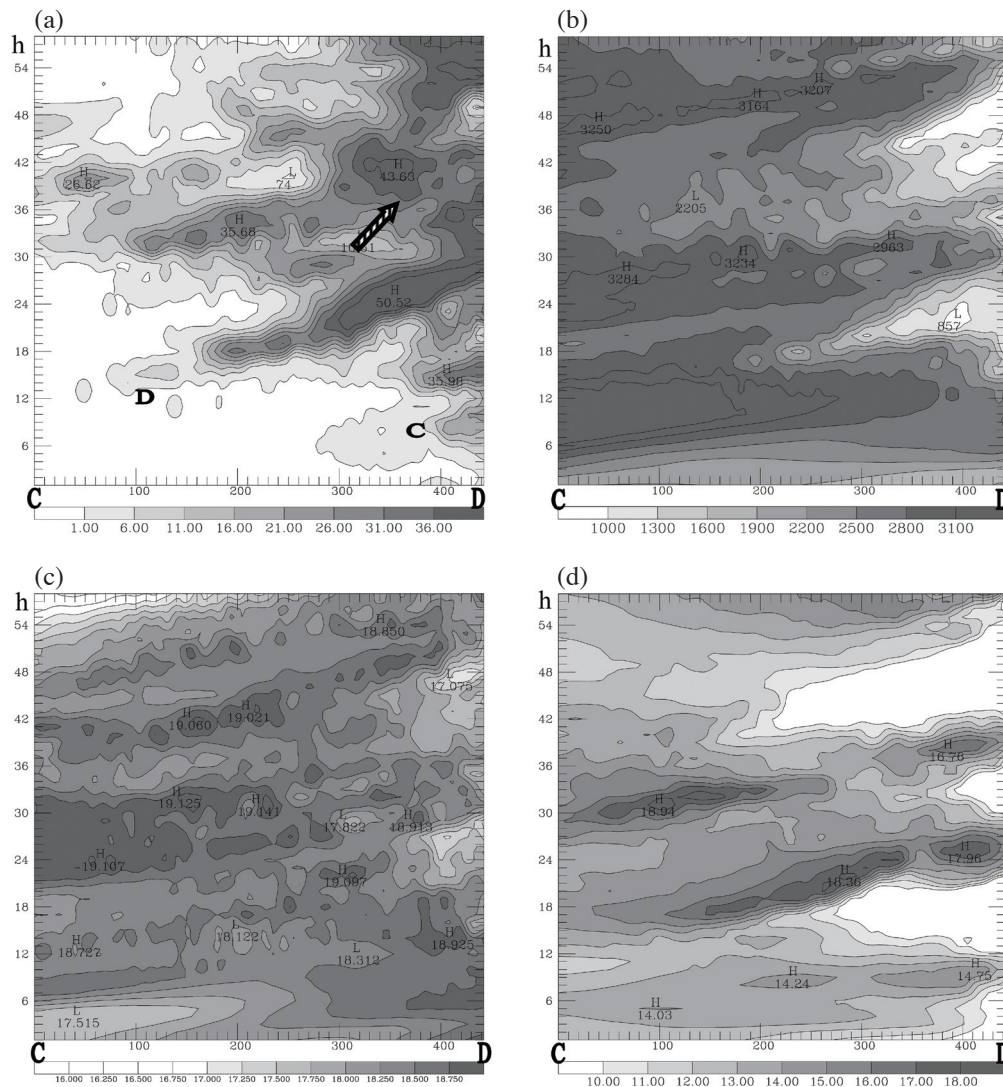
Fig. 12. Same as Fig. 11, but for cross section CD (location shown in Fig. 3b).
