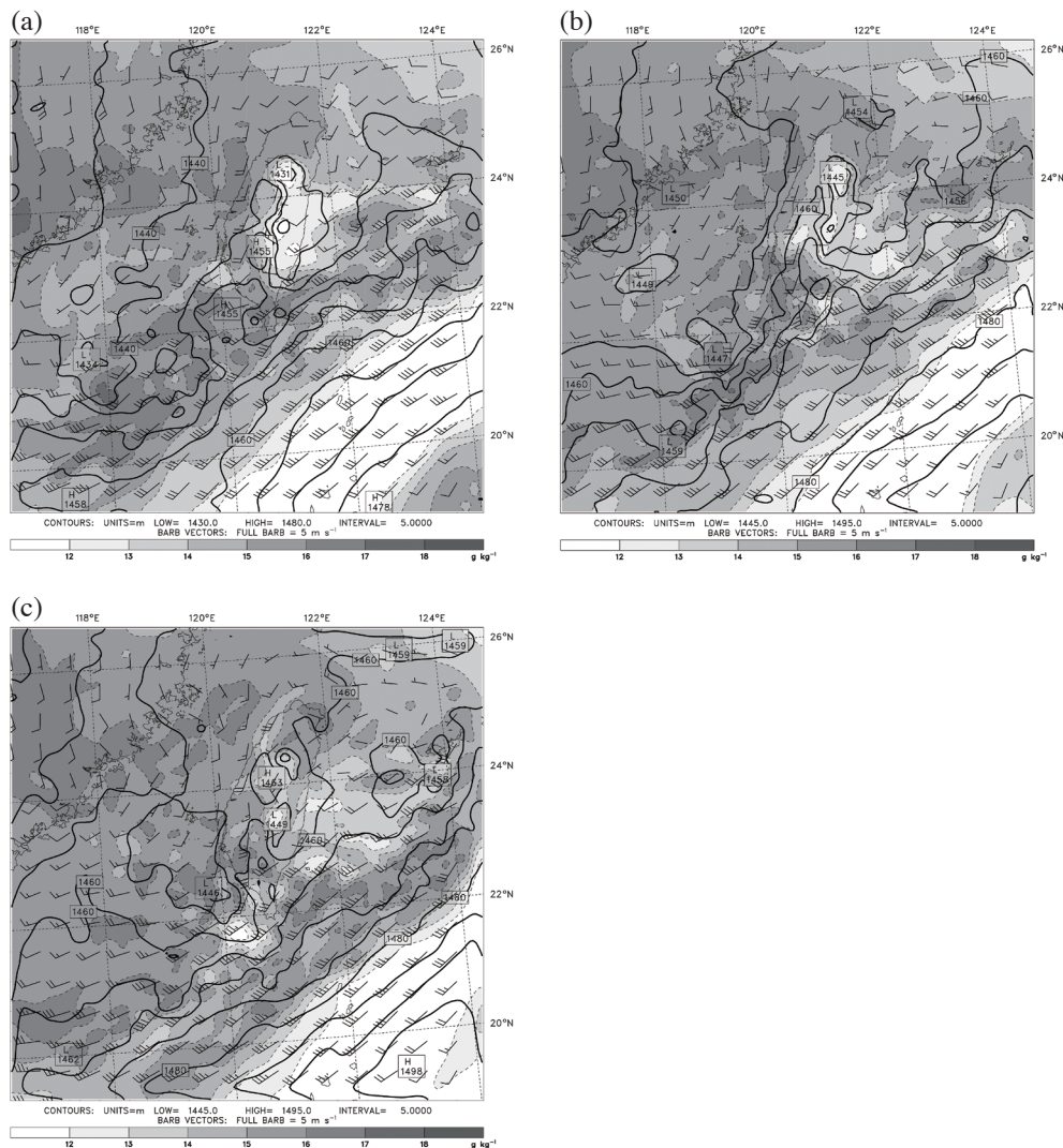
Fig. 15. The 850-hPa water vapor mixing ratio (shading and dashed lines, with scale shown in bottom; \text{g kg}^{-1} ), geopotential height (solid lines with a 5-m interval), and wind barbs (full bar: 5 \text{ m s}^{-1} ) of domain 3 at (a) 32 h (2000 UTC 12 June), (b) 35 h (2300 UTC 12 June), and (c) 38 h (0200 UTC 13 June).
