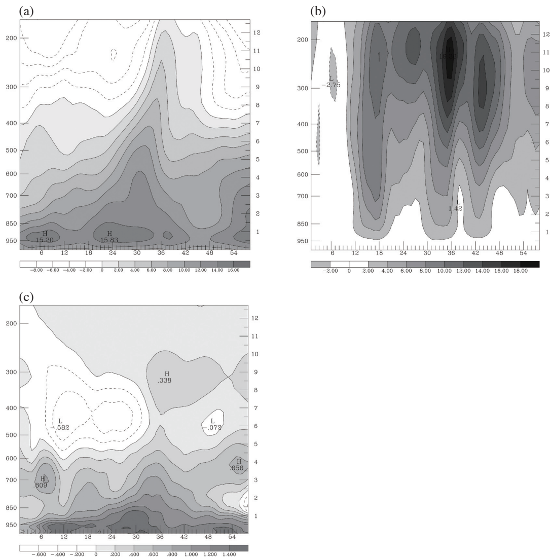
Fig. 13. Time evolution of (a) southwesterly wind component ( \text{m s}^{-1} ), (b) vertical velocity ( \text{cm s}^{-1} ), and (c) water vapor mixing ratio perturbation ( \text{g kg}^{-1} ) averaged inside box CFDG (location shown in Fig. 3b). The abscissa is time from 1 - 58 h of model simulation, and the ordinate is height. The scale is shown in bottom for each plot.
