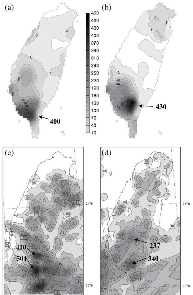
Fig. 7. The observed 24-h accumulated rainfall (mm) in Taiwan (a) from 1200 UTC 11 June to 1200 UTC 12 June 2005, and (b) from 1200 UTC 12 June to 1200 UTC 13 June 2005. The simulated rainfall (mm) from domain 3 at (c) 0 - 24 h and (d) 24 - 48 h. The contour interval is 30 mm, with scale shown on the middle top and maximum rainfall amounts denoted.
