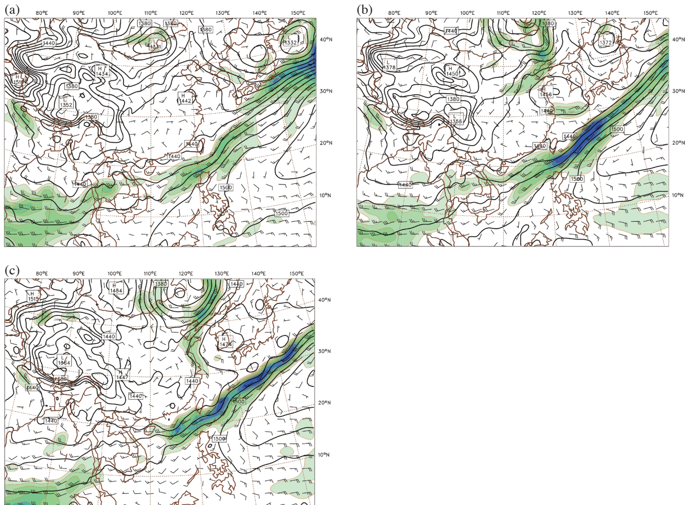
Fig. 2. The 850-hPa geopotential height (solid lines with a 15-m interval), wind barbs (full bar: 5 \text{ m s}^{-1} ), and wind speed (color shading with red lines, starting at 10 \text{ m s}^{-1} with a 2 \text{ m s}^{-1} interval) from the NCEP final analysis (FNL) data at (a) 1200 UTC 11 June 2005, (b) 1200 UTC 12 June 2005, and (c) 1200 UTC 13 June 2005.
