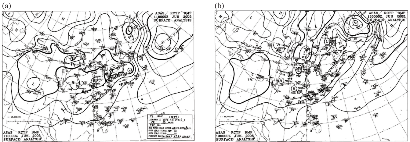
Fig. 1. Surface weather maps issued by the Central Weather Bureau (CWB) at (a) 0000 UTC 11 June 2005, and (b) 0000 UTC 13 June 2005. Contour interval for sea level pressure is 4 hPa.
