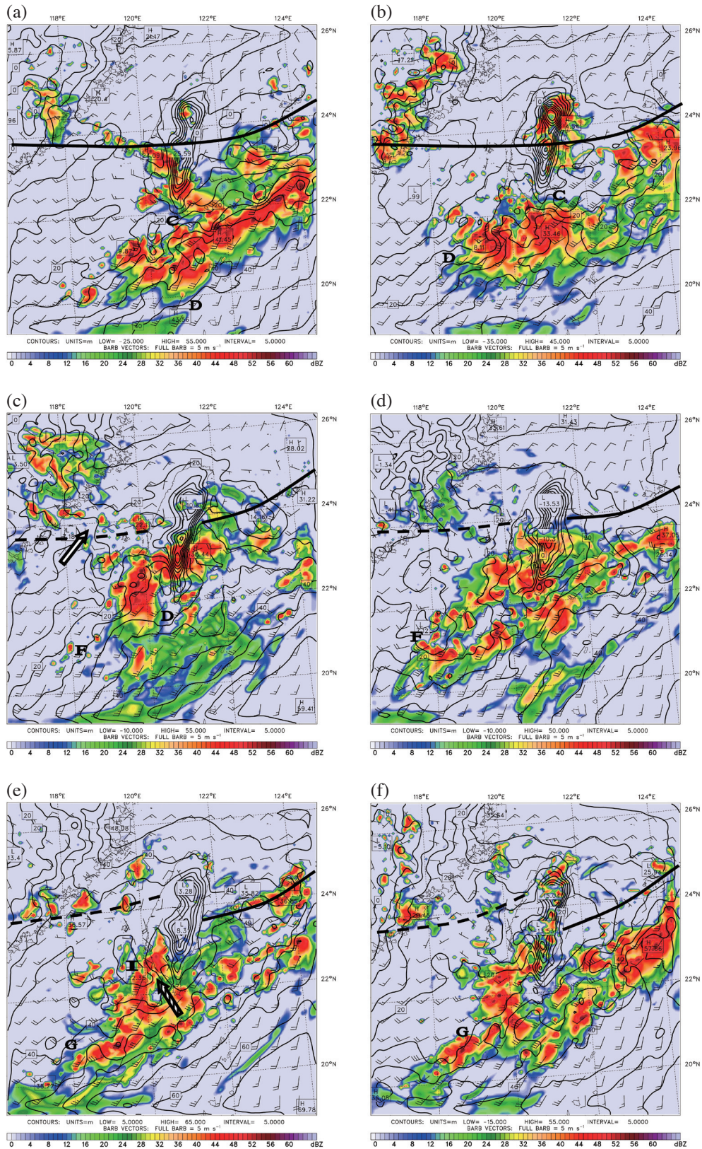
Fig. 8. Maximum radar reflectivity (shading, with dBZ scale shown in bottom), 1000-hPa geopotential height (contour lines at a 5-gpm interval) and winds (full barb is 5 \text{ m s}^{-1} ) of domain 3 at (a) 14 h (0200 UTC 12 June 2005), (b) 20 h (0800 UTC 12 June), (c) 26 h (1400 UTC 12 June), (d) 32 h (2000 UTC 12 June), (e) 38 h (0200 UTC 13 June), and (f) 41 h (0500 UTC 13 June). The frontal location is indicated by thick solid and dashed lines. Convective bands Y and Z are indicated by hollow and hatched arrows, respectively. MCSs corresponding to Figs. 5 and 6 are denoted by upper-case letters.
