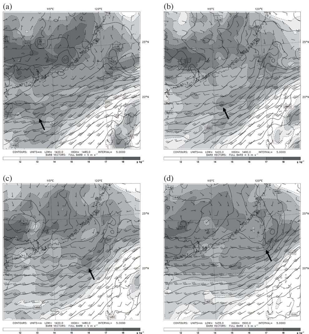
Fig. 9. The 850-hPa water vapor mixing ratio (shading and dashed lines, with scale shown in bottom; \text{g kg}^{-1} ), geopotential height (solid lines with a 5-m interval), and wind barbs (full bar: 5 \text{ m s}^{-1} ) of domain 2 at (a) 20 h (0800 UTC 12 June), (b) 26 h (1400 UTC 12 June), (c) 32 h (2000 UTC 12 June), and (d) 38 h (0200 UTC 13 June). A short-wave trough with moister air is indicated by an arrow.
