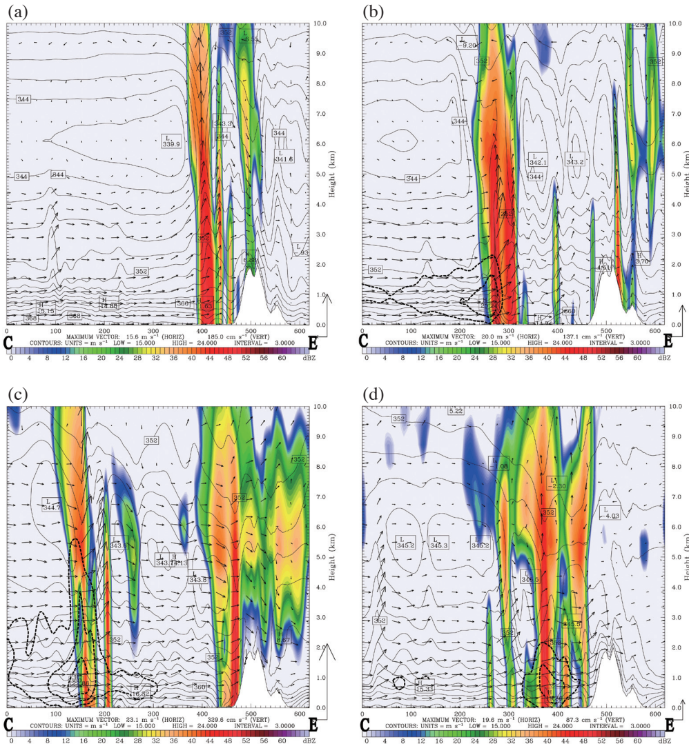
Fig. 10. Simulated radar reflectivity (color, dBZ), equivalent potential temperature (contour lines at a 2-K interval), and wind vectors (scale shown in the lower right) of domain 3 along cross section CE (location shown in Fig. 3b) at (a) 14 h (0200 UTC 12 June 2005), (b) 20 h (0800 UTC 12 June), (c) 32 h (2000 UTC 12 June), and (d) 38 h (0200 UTC 13 June). Along-section winds greater than 15 \text{ m s}^{-1} are plotted in dashed lines with a 3 \text{ m s}^{-1} interval.
