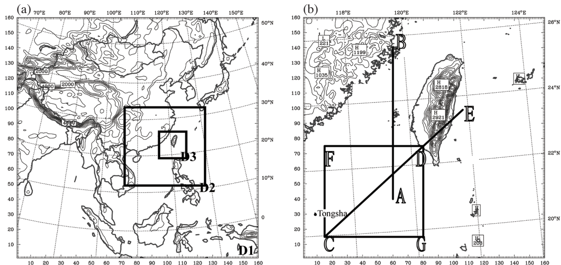
Fig. 3. The domain setting of model simulation. (a) Horizontal resolution of domains 1, 2, and 3 are 45, 15, and 5 km, respectively. Terrain height is plotted with a 500-m interval. (b) Terrain height of domain 3 is plotted with a 200-m interval. Lines AB, CD, and CE denote the locations of cross sections. Box CFDG represents the area of domain average.
