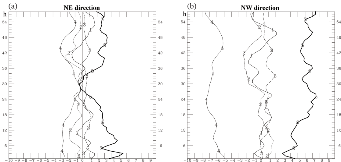
Fig. 14. Time evolution of momentum budgets in the (a) northeastward and (b) northwestward directions along line CD at 850 hPa averaged inside box CFDG (location shown in Fig. 3b). Curves 1 - 5 denote local change (LC), horizontal advection (HA), vertical advection (VA), Coriolis force (CF), and pressure gradient force (PGF), respectively. The ordinate is time from 1 - 58 h of model simulation, and the abscissa is magnitude (unit: 1 \times 10^{-4} \text{ m s}^{-2} ).
