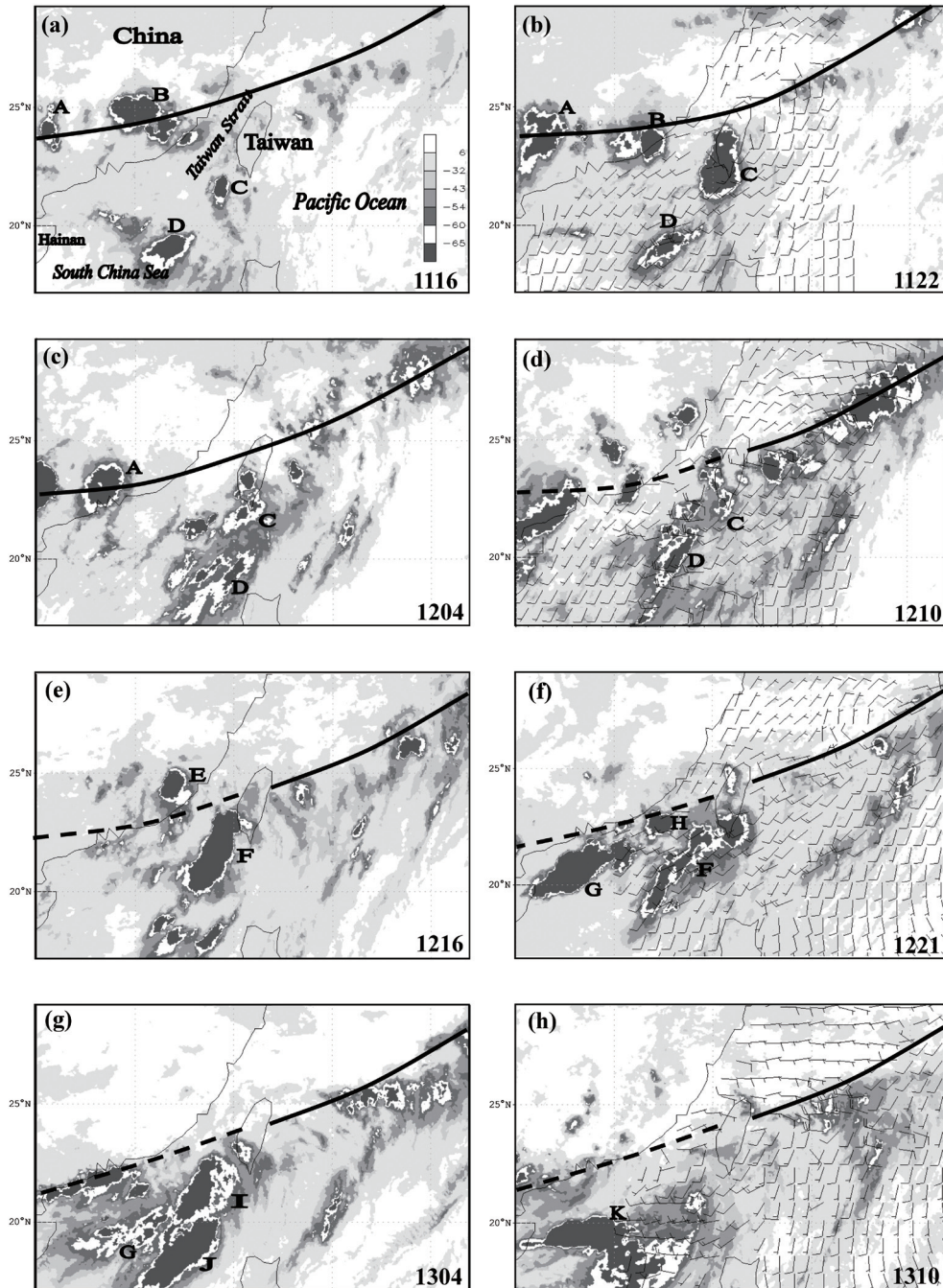
Fig. 5. Infrared satellite brightness temperature (shading) and QuikSCAT surface wind (full barb is 5 \text{ m s}^{-1} ) at (a) 1600 UTC 11 June, (b) 2200 UTC 11 June, (c) 0400 UTC 12 June, (d) 1000 UTC 12 June, (e) 1600 UTC 12 June, (f) 2100 UTC 12 June, (g) 0400 UTC 13 June, and (h) 1000 UTC 13 June 2005. The thick line indicates the location of a front, with dashed line denoting a weak or insignificant front. MCSs are denoted by letters A - K.
