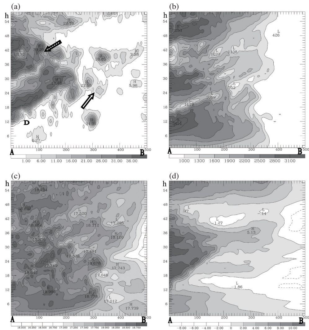
Fig. 11. Time evolution of (a) maximum radar reflectivity (dBZ), (b) maximum CAPE ( J kg^{-1} ), (c) water vapor mixing ratio ( g kg^{-1} ), and (d) along-section wind ( m s^{-1} , positive velocity denotes a toward-the-right wind direction) of domain 3 along cross section AB (location shown in Fig. 3b). Fields in (c) and (d) are averaged below 850 hPa. The ordinate is time from 1 - 58 h of model simulation, and the abscissa is distance in km. Shading indices are shown in bottom with solid lines denoting positive and dashed lines representing negative values. Convective bands Y and Z are denoted by hollow and hatched arrows, respectively, and MCS D is indicated by capital letter D.
