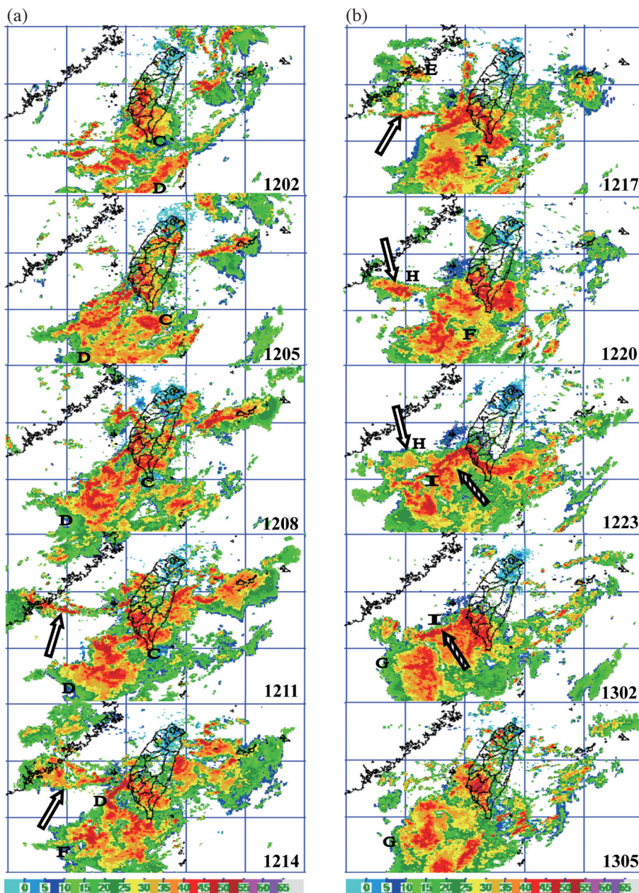
Fig. 6. Radar reflectivity images (dBZ, with scale shown on the bottom) (a) from 0200 UTC 12 to 1400 UTC 12 June 2005, and (b) from 1700 UTC 12 to 0500 UTC 13 June 2005 at a 3-h interval. Convective bands Y and Z are indicated by hollow and hatched arrows, respectively. MCSs corresponding to Fig. 5 are denoted by upper-case letters.
